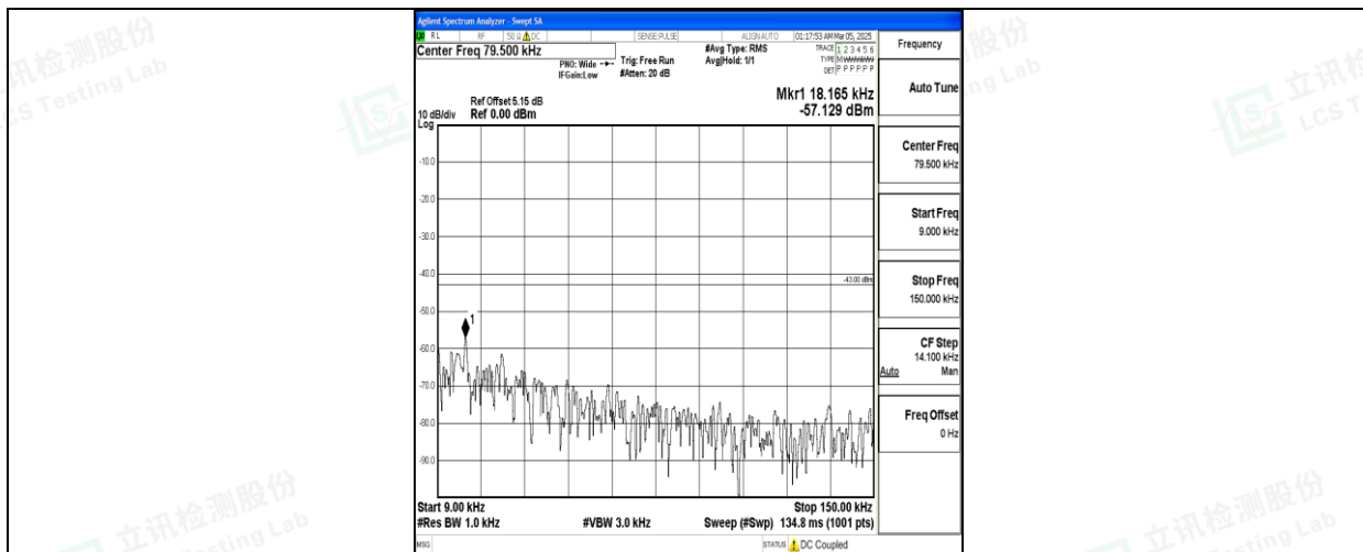
Band66_20MHz_QPSK_132322_1RB#0_0.009~0.15_0.009~0.15
