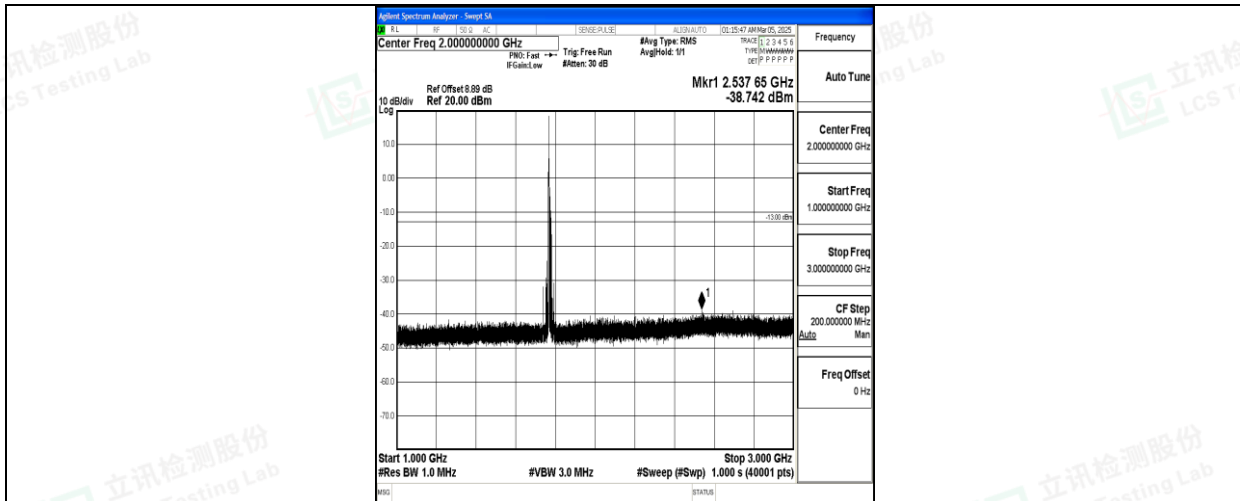
Band66_15MHz_16QAM_132597_1RB#0_1000~3000_1000~3000
