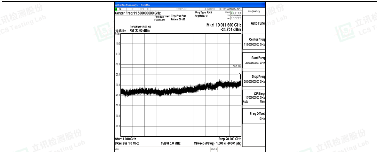
Band66_20MHz_16QAM_132322_1RB#0_3000~20000_3000~20000
