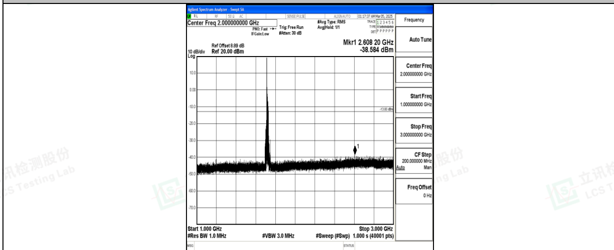
Band66_20MHz_16QAM_132072_1RB#0_1000-3000_1000-3000
