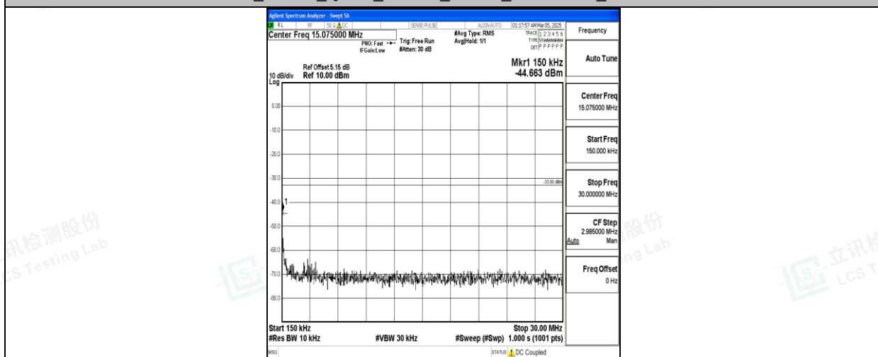
Band66_20MHz_QPSK_132322_1RB#0_0.15~30_0.15~30
