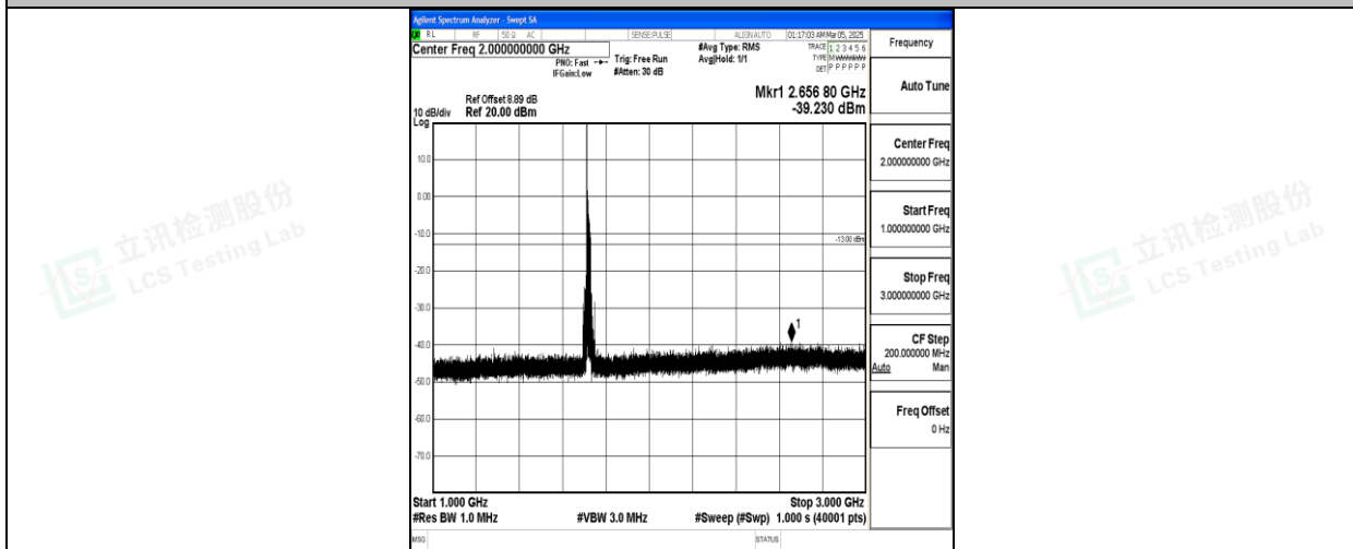
Band66_20MHz_QPSK_132072_1RB#0_1000~3000_1000~3000
