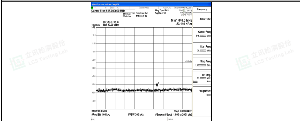
Band66_20MHz_16QAM_132572_1RB#0_30~1000_30~1000
