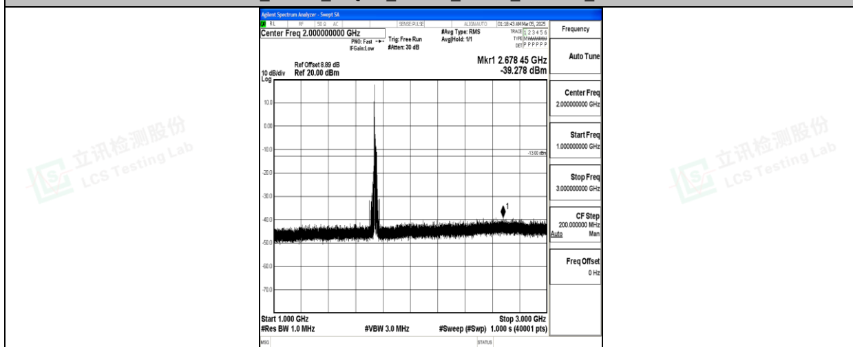
Band66_20MHz_16QAM_132322_1RB#0_1000~3000_1000~3000
