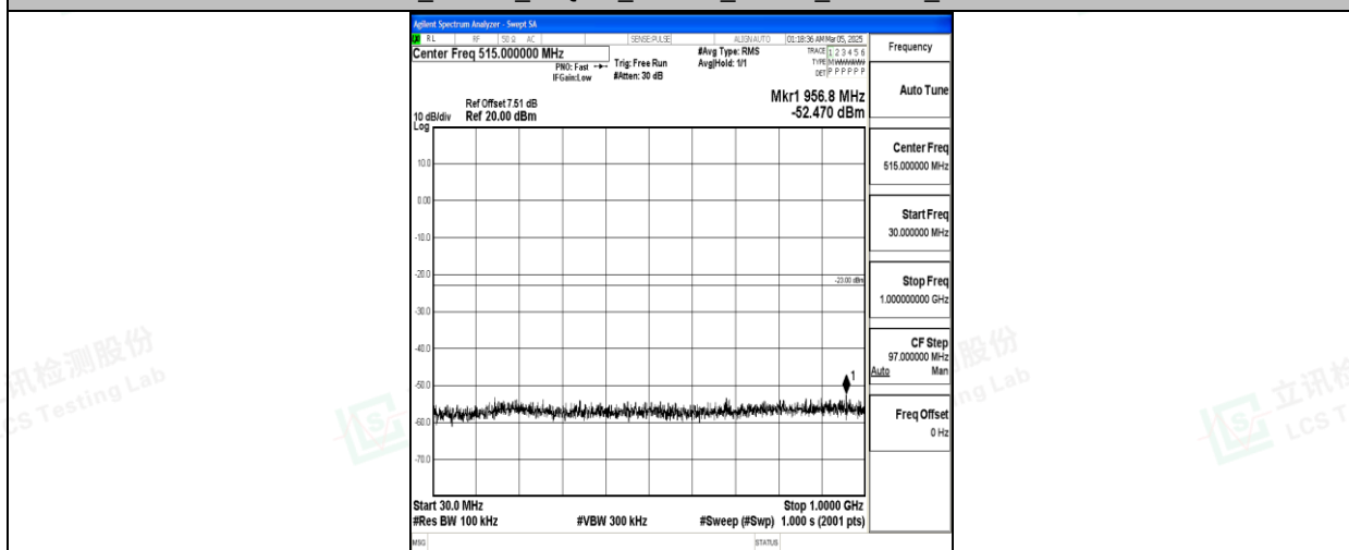
Band66_20MHz_16QAM_132322_1RB#0_30~1000_30~1000
