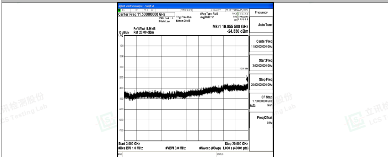
Band66_20MHz_QPSK_132322_1RB#0_3000~20000_3000~20000
