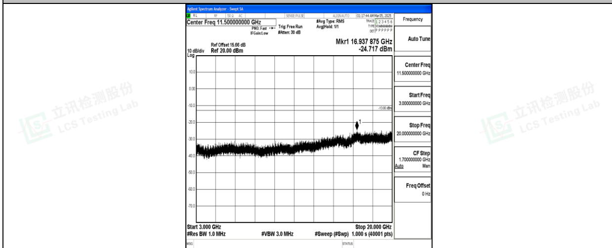
Band66_20MHz_16QAM_132072_1RB#0_3000-20000_3000-20000
