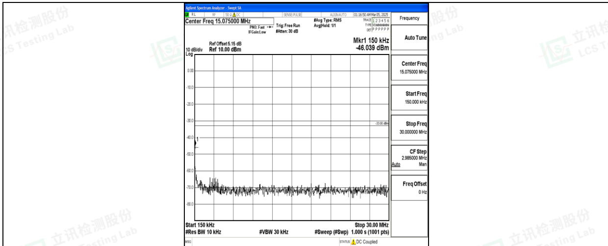
Band66_20MHz_QPSK_132072_1RB#0_0.15~30_0.15~30
