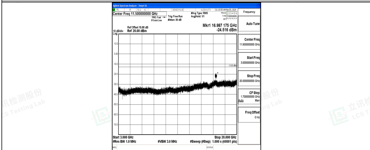
Band66_15MHz_16QAM_132597_1RB#0_3000~20000_3000~20000
