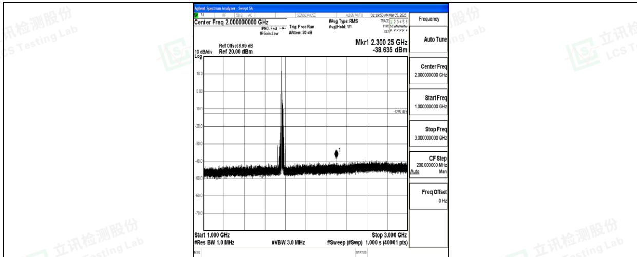
Band66_20MHz_16QAM_132572_1RB#0_1000~3000_1000~3000
