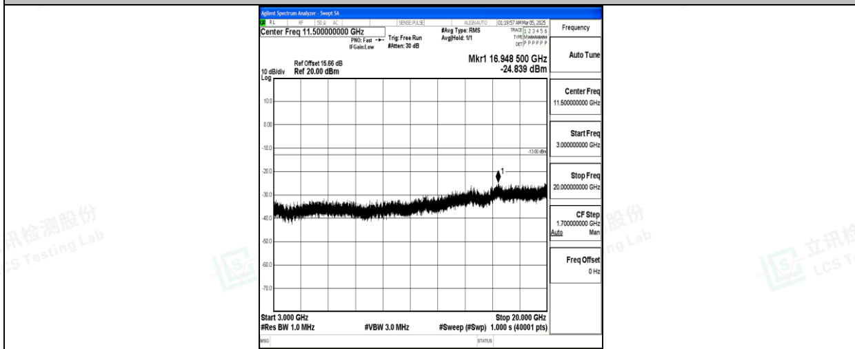
Band66_20MHz_16QAM_132572_1RB#0_3000~20000_3000~20000
