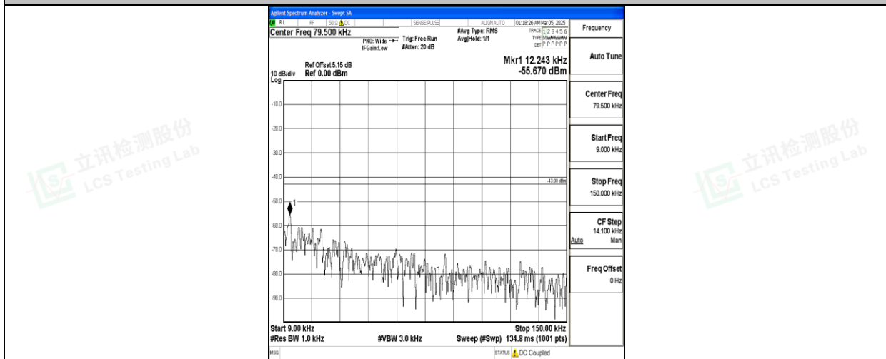
Band66_20MHz_16QAM_132322_1RB#0_0.009~0.15_0.009~0.15
