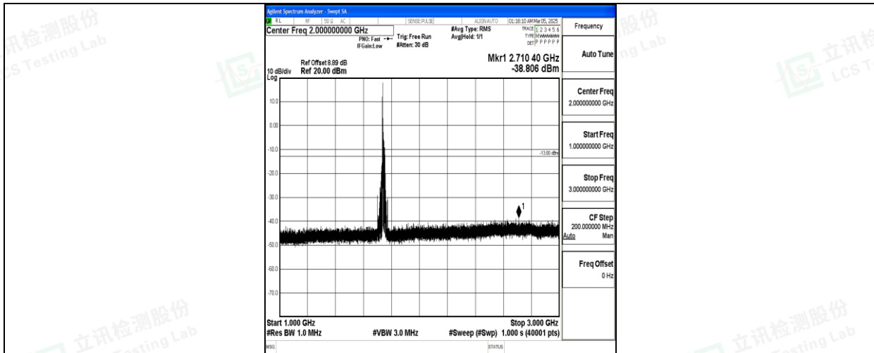
Band66_20MHz_QPSK_132322_1RB#0_1000~3000_1000~3000
