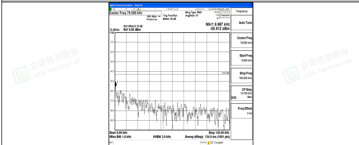
Band66_20MHz_QPSK_132072_1RB#0_0.009~0.15_0.009~0.15
