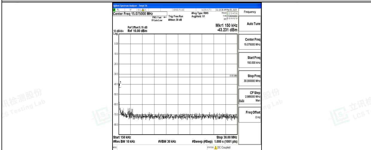
Band66_20MHz_16QAM_132572_1RB#0_0.15~30_0.15~30
