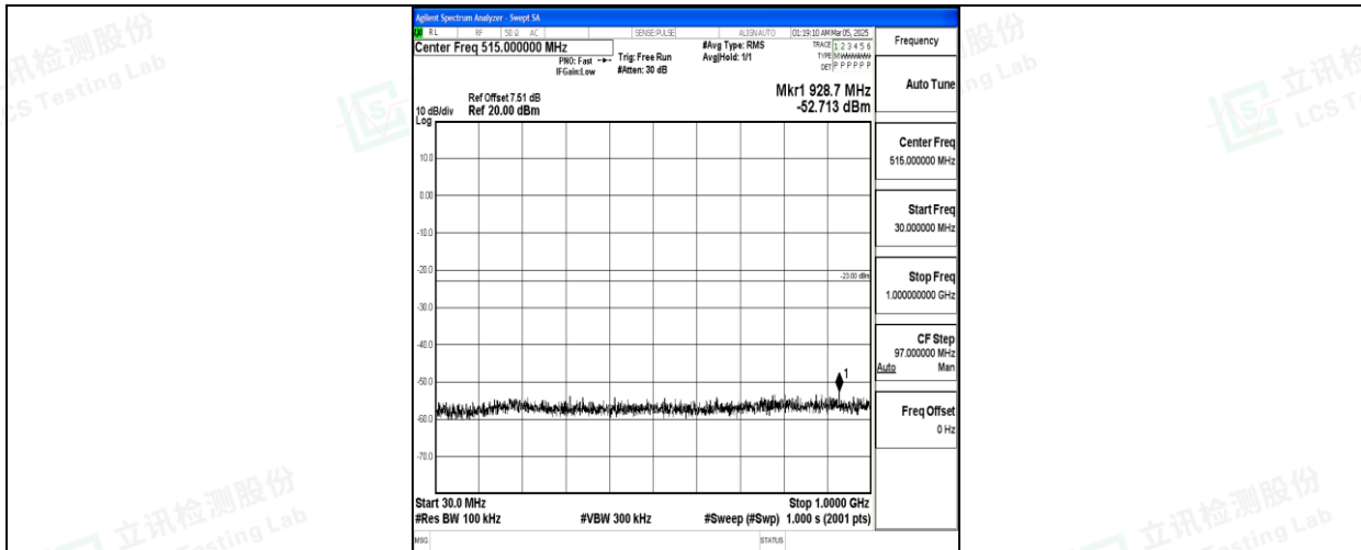
Band66_20MHz_QPSK_132572_1RB#0_30~1000_30~1000
