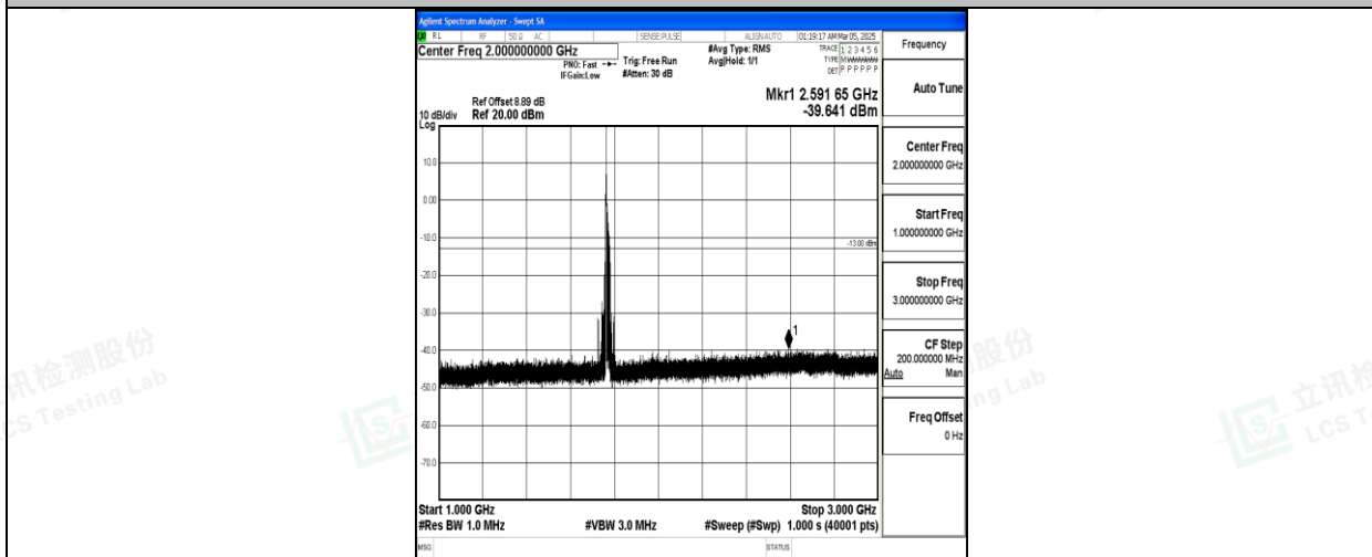
Band66_20MHz_QPSK_132572_1RB#0_1000~3000_1000~3000
