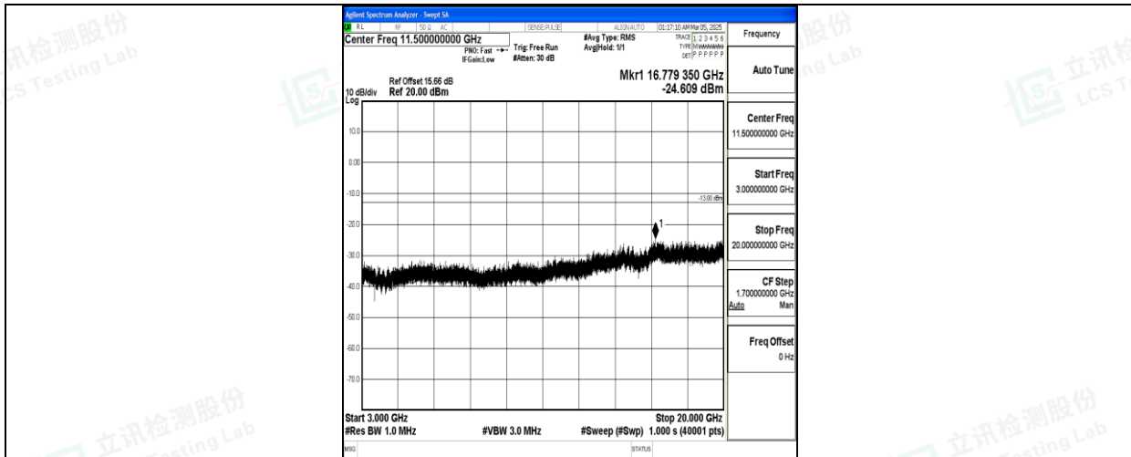
Band66_20MHz_QPSK_132072_1RB#0_3000~20000_3000~20000
