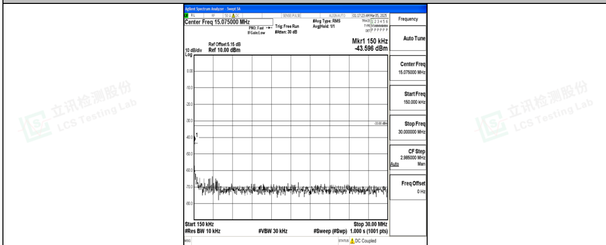
Band66_20MHz_16QAM_132072_1RB#0_0.15~30_0.15~30
