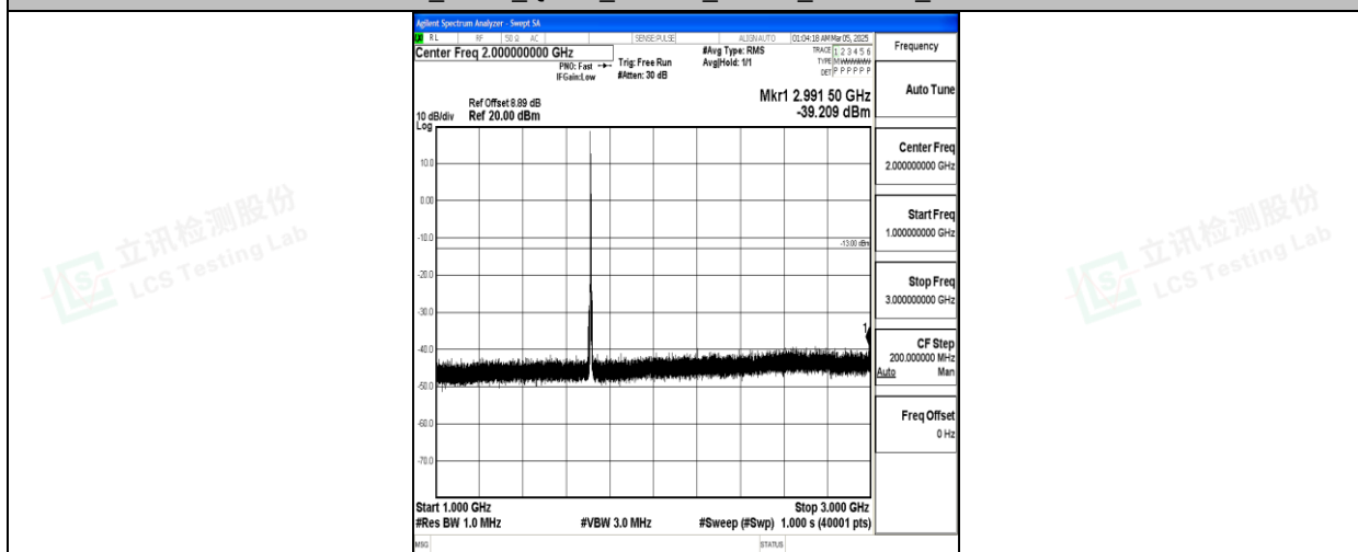
Band66_5MHz_QPSK_131997_1RB#0_1000~3000_1000~3000
