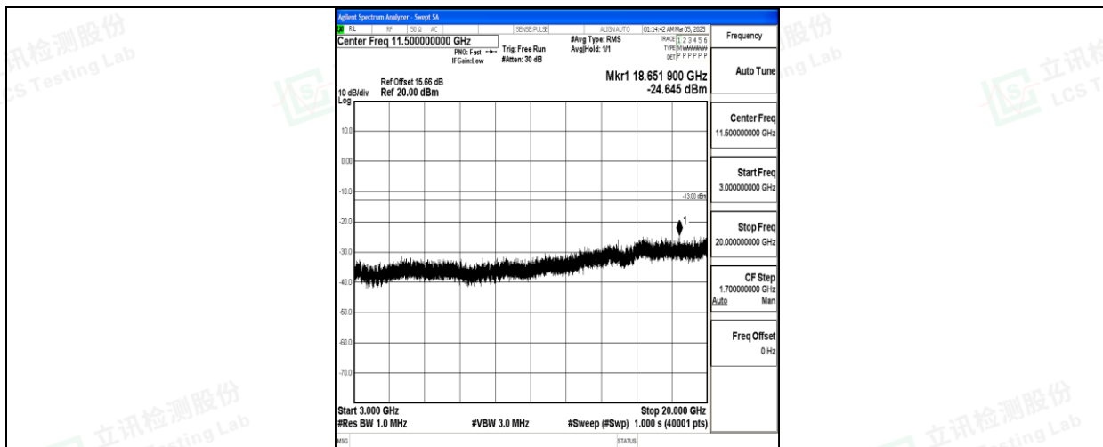
Band66_15MHz_16QAM_132322_1RB#0_3000~20000_3000~20000
