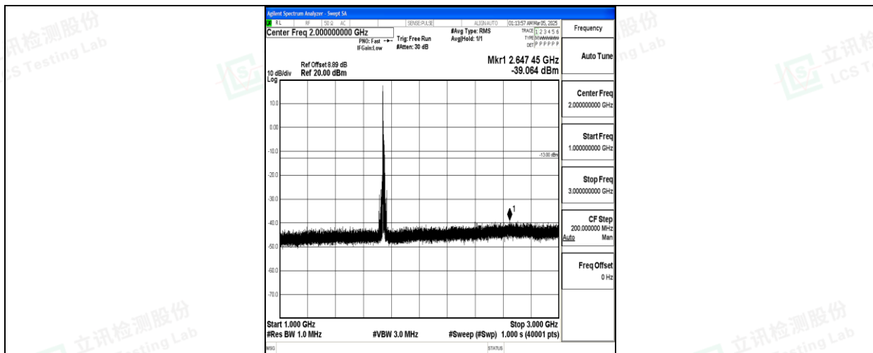
Band66_15MHz_QPSK_132322_1RB#0_1000~3000_1000~3000
