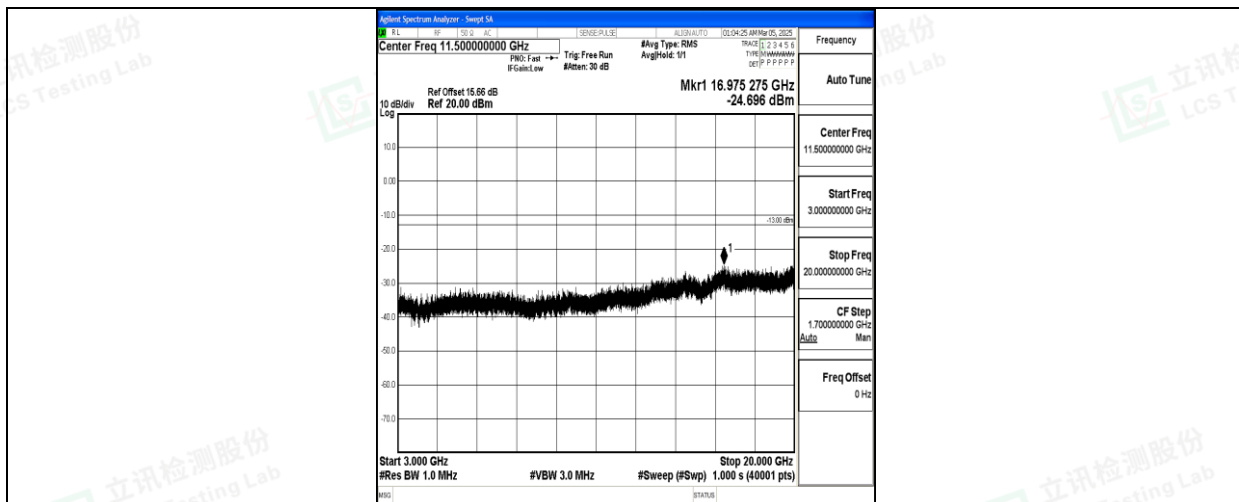
Band66_5MHz_QPSK_131997_1RB#0_3000~20000_3000~20000
