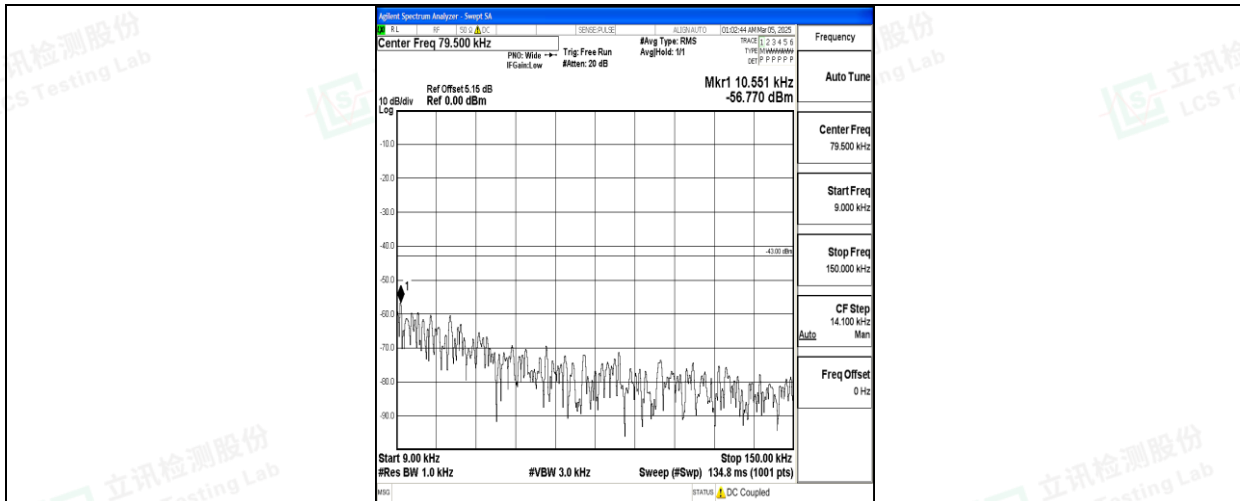
Band66_3MHz_16QAM_132657_1RB#0_0.009~0.15_0.009~0.15
