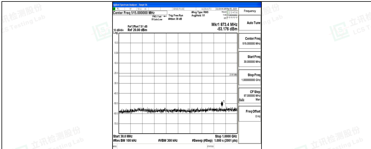
Band66_5MHz_16QAM_131997_1RB#0_30~1000_30~1000
