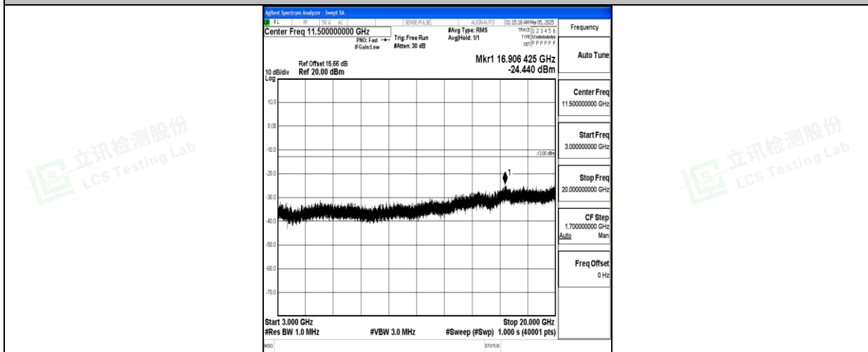
Band66_15MHz_QPSK_132597_1RB#0_3000~20000_3000~20000
