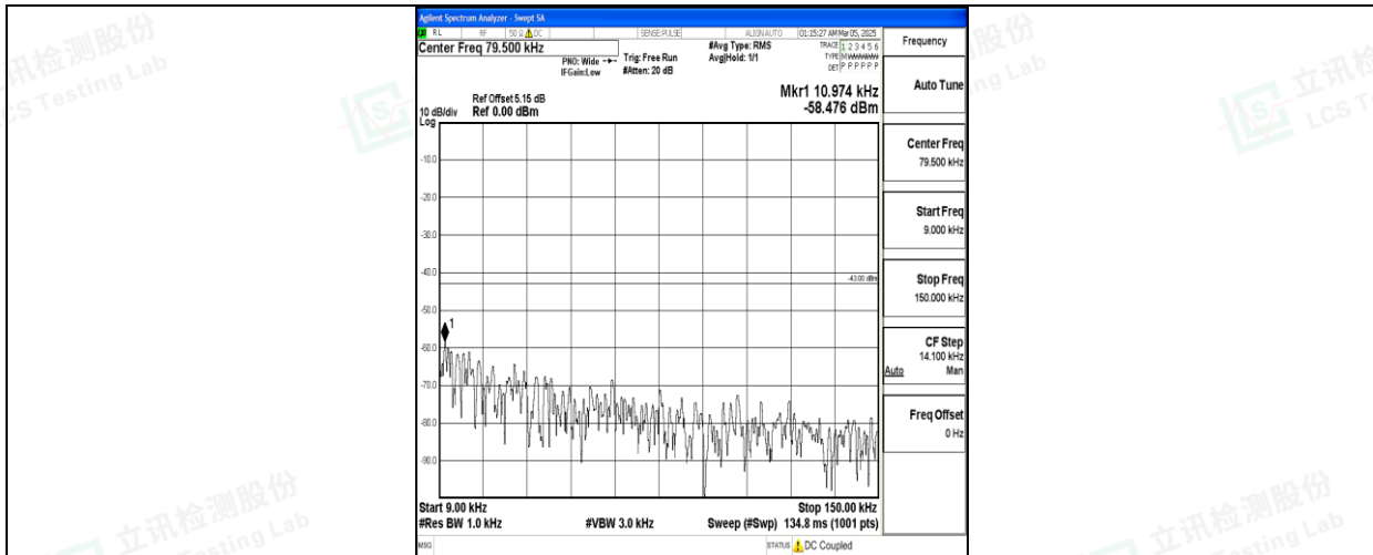
Band66_15MHz_16QAM_132597_1RB#0_0.009~0.15_0.009~0.15
