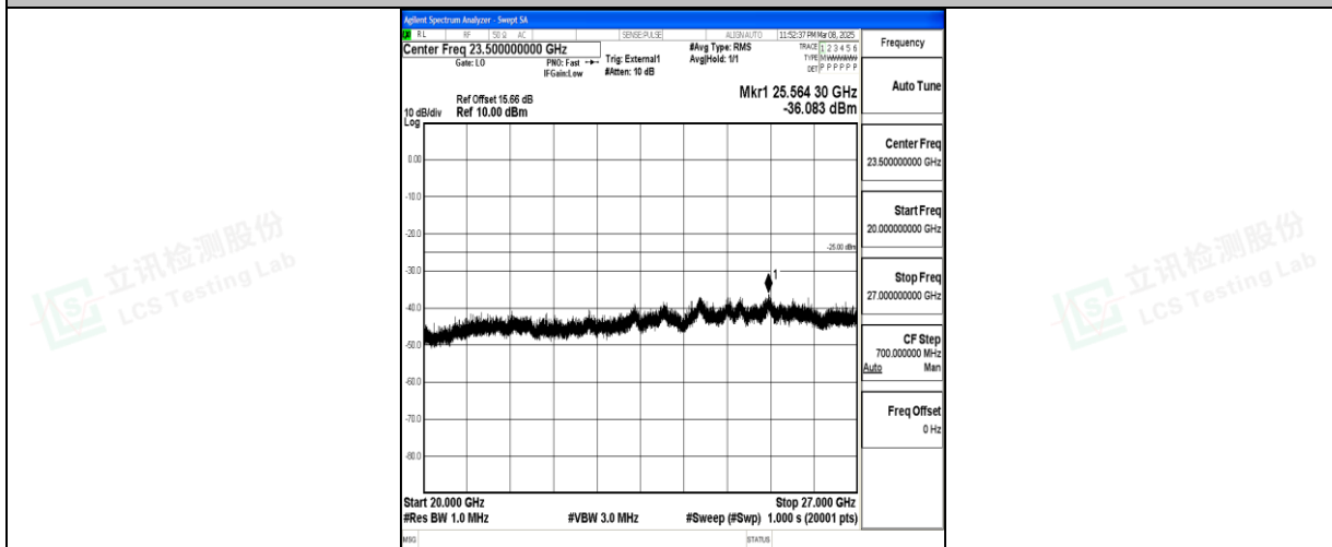
Band41_20MHz_16QAM_41490_1RB#0_20000~27000_20000~27000
