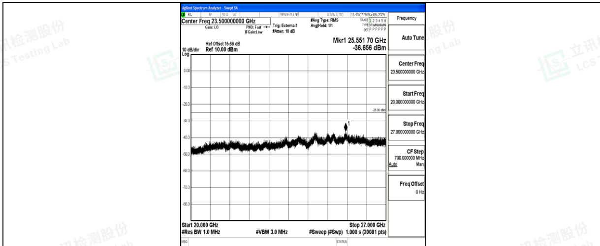
Band41_20MHz_QPSK_39750_1RB#0_20000~27000_20000~27000
