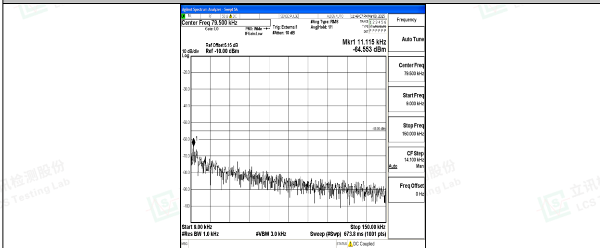
Band41_20MHz_QPSK_41490_1RB#0_0.009~0.15_0.009~0.15
