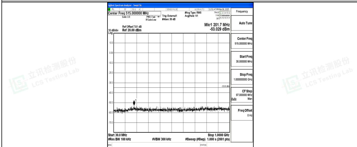
Band41_20MHz_16QAM_41490_1RB#0_30~1000_30~1000
