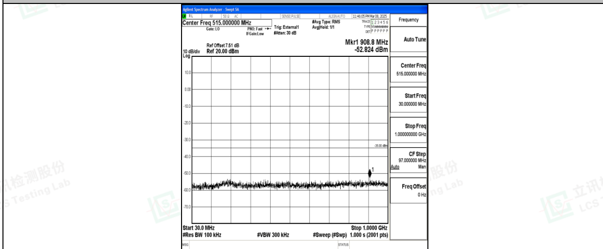
Band41_20MHz_QPSK_40620_1RB#0_30~1000_30~1000
