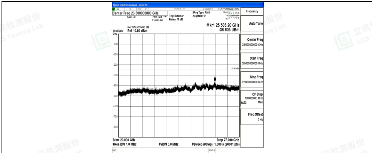
Band41_20MHz_16QAM_39750_1RB#0_20000~27000_20000~27000
