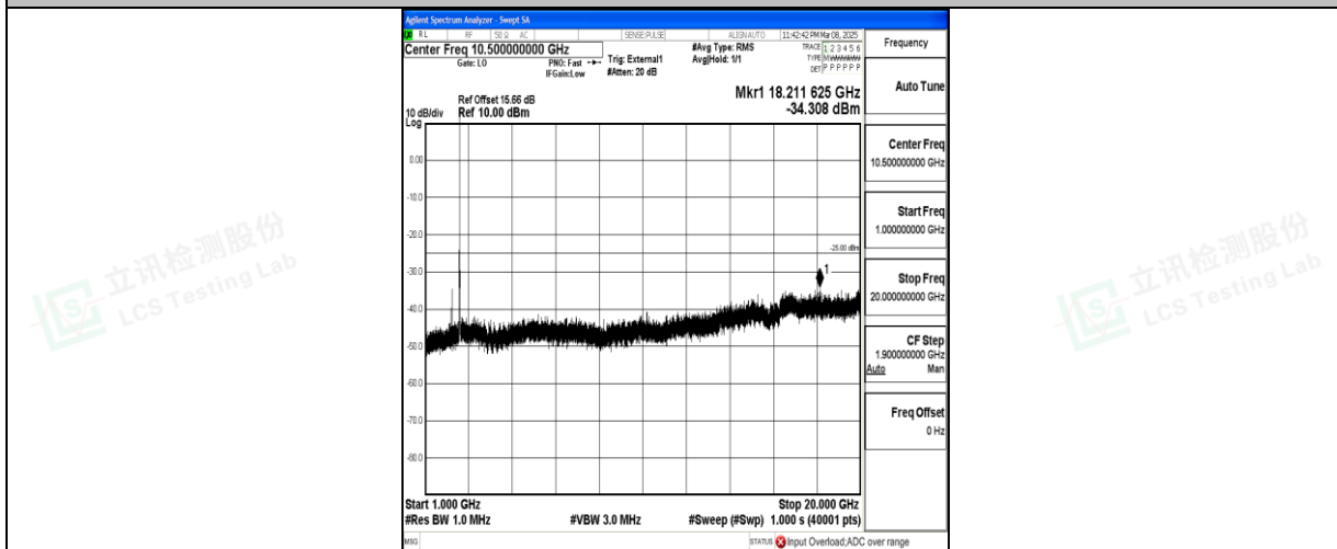
Band41_20MHz_QPSK_39750_1RB#0_1000~20000_1000~20000
