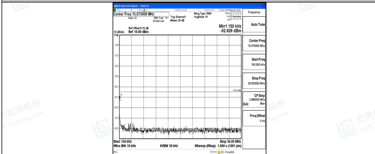
Band41_20MHz_16QAM_41490_1RB#0_0.15~30_0.15~30
