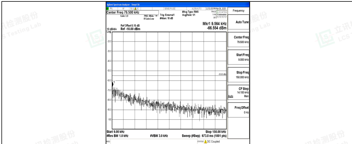
Band41_20MHz_16QAM_41490_1RB#0_0.009~0.15_0.009~0.15
