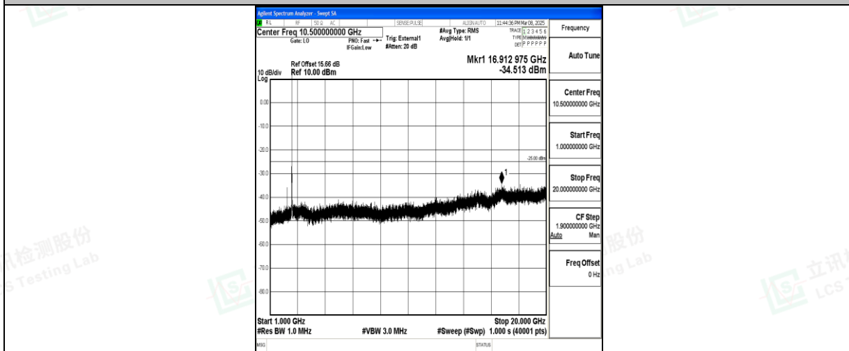
Band41_20MHz_16QAM_39750_1RB#0_1000~20000_1000~20000
