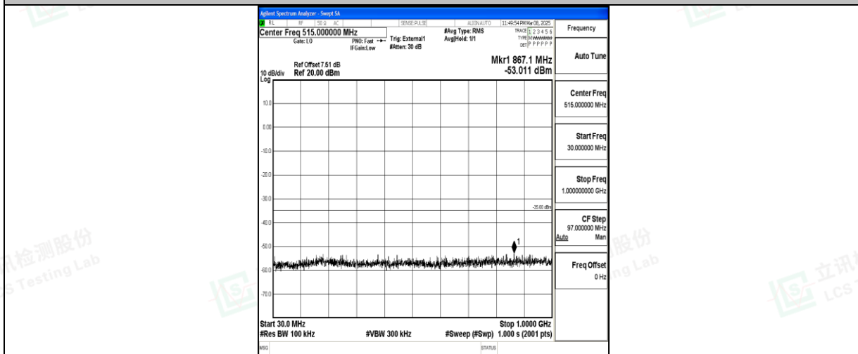
Band41_20MHz_QPSK_41490_1RB#0_30~1000_30~1000
