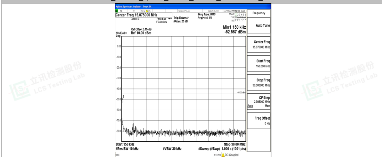
Band41_20MHz_QPSK_41490_1RB#0_0.15~30_0.15~30
