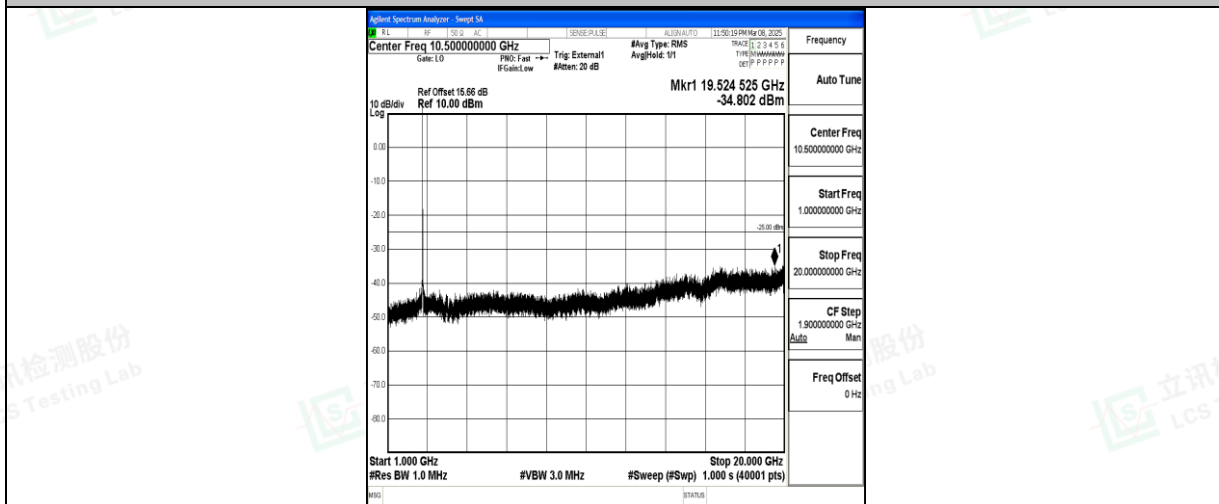
Band41_20MHz_QPSK_41490_1RB#0_1000~20000_1000~20000
