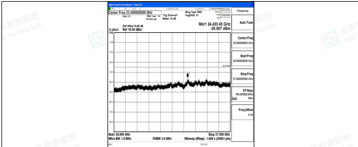
Band41_20MHz_QPSK_40620_1RB#0_20000~27000_20000~27000
