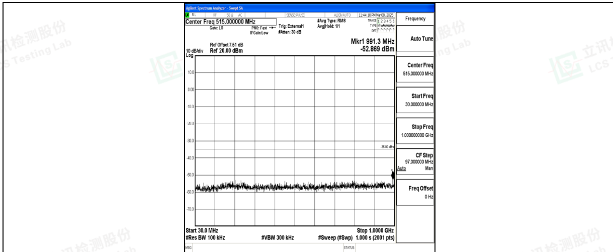
Band41_20MHz_16QAM_39750_1RB#0_30~1000_30~1000
