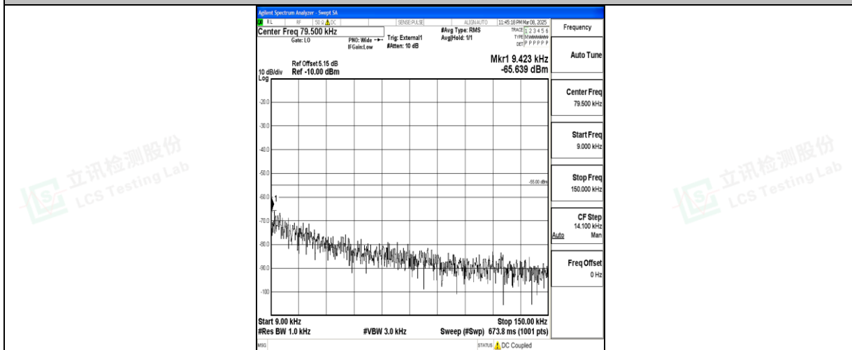
Band41_20MHz_QPSK_40620_1RB#0_0.009~0.15_0.009~0.15
