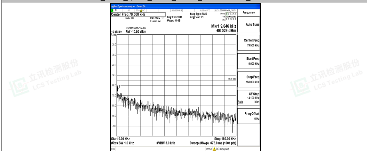
Band41_5MHz_16QAM_39675_1RB#0_0.009~0.15_0.009~0.15
