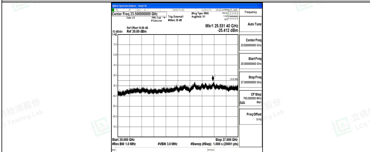
Band41_15MHz_16QAM_41515_1RB#0_20000~27000_20000~27000
