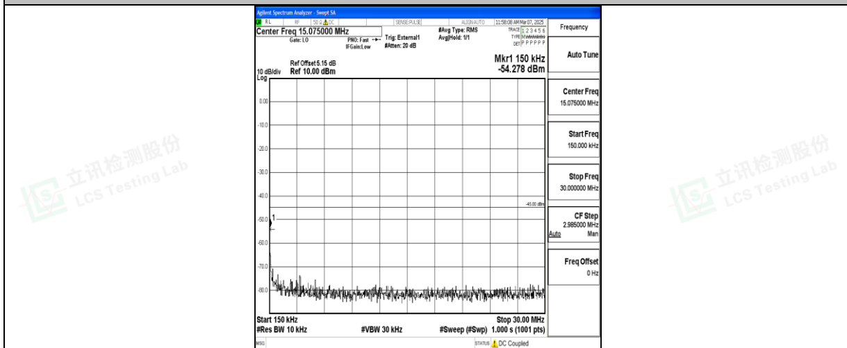
Band41_10MHz_QPSK_41540_1RB#0_0.15~30_0.15~30
