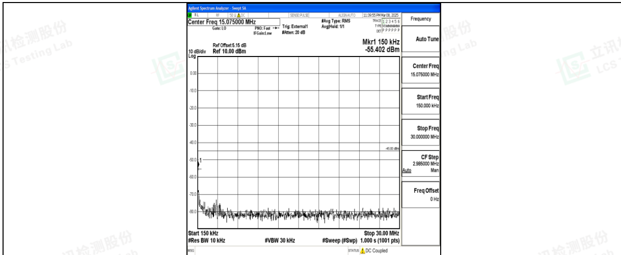
Band41_5MHz_16QAM_41565_1RB#0_0.15~30_0.15~30
