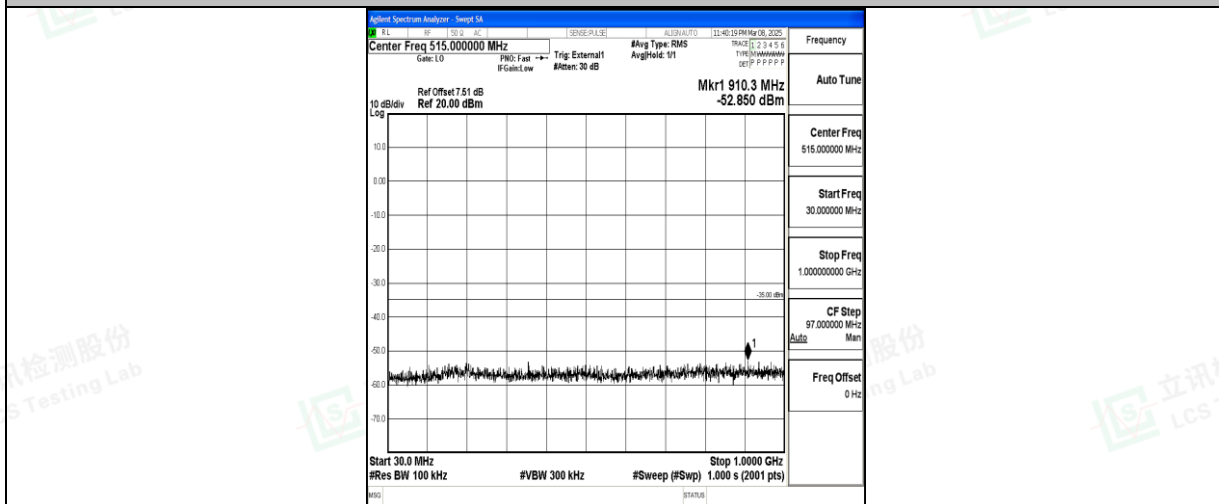
Band41_5MHz_16QAM_41565_1RB#0_30~1000_30~1000
