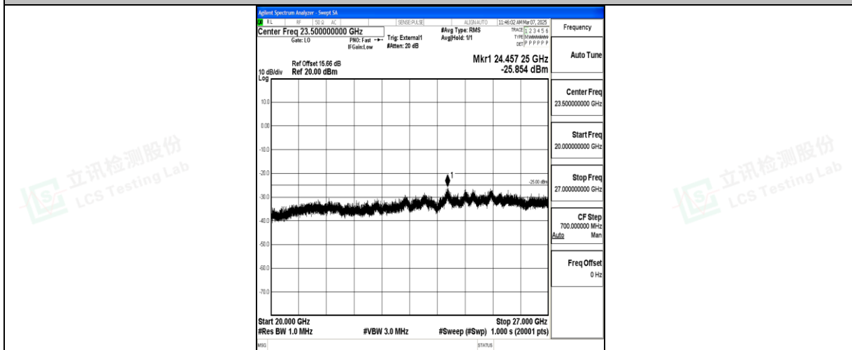
Band41_10MHz_16QAM_39700_1RB#0_20000~27000_20000~27000
