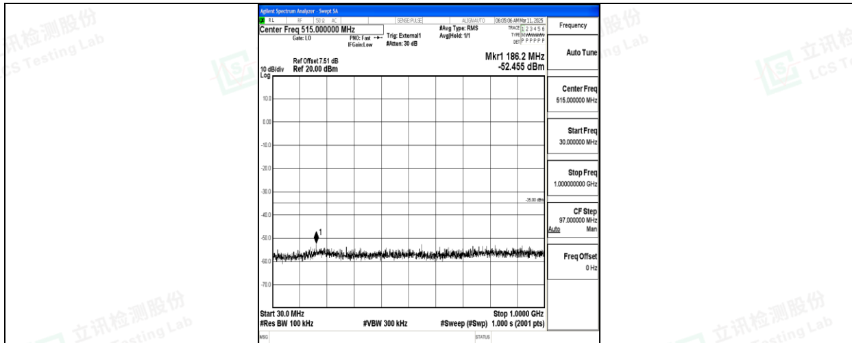
Band38_15MHz_16QAM_38000_1RB#0_30~1000_30~1000
