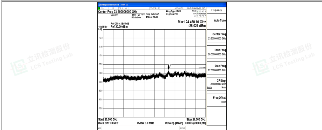
Band38_15MHz_16QAM_38000_1RB#0_20000~27000_20000~27000
