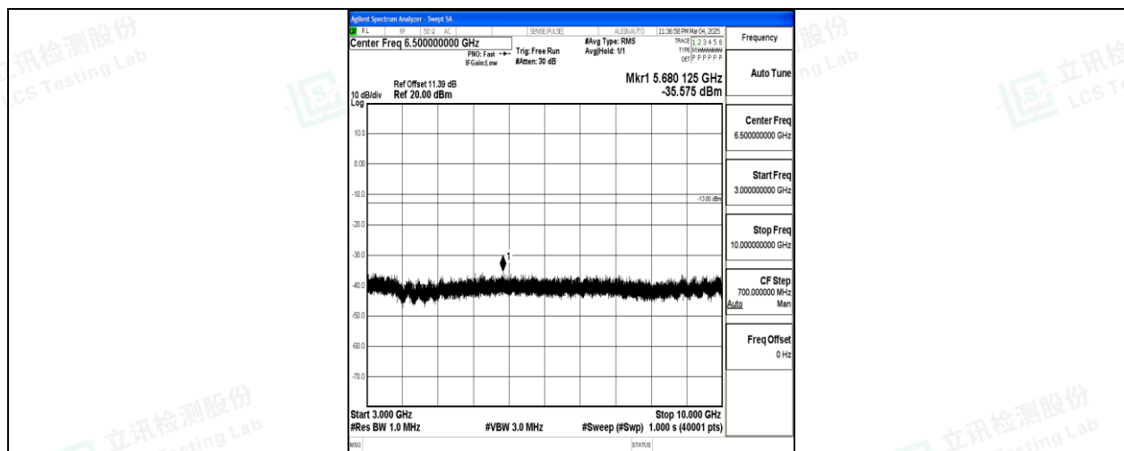
Band26_1.4MHz_QPSK_27033_1RB#0_3000~10000_3000~10000
