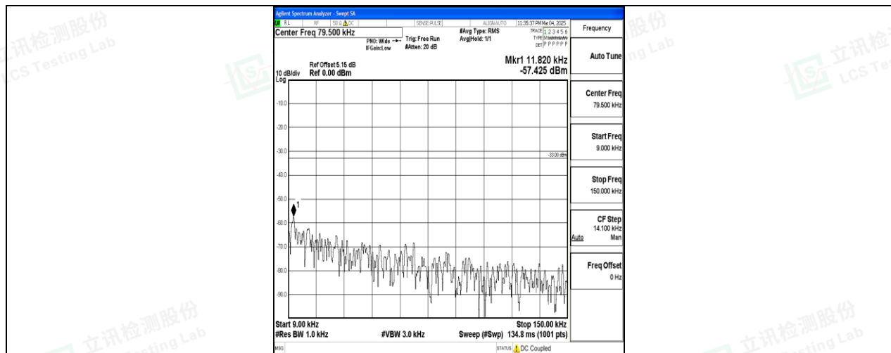
Band26_1.4MHz_16QAM_26915_1RB#0_0.009~0.15_0.009~0.15
