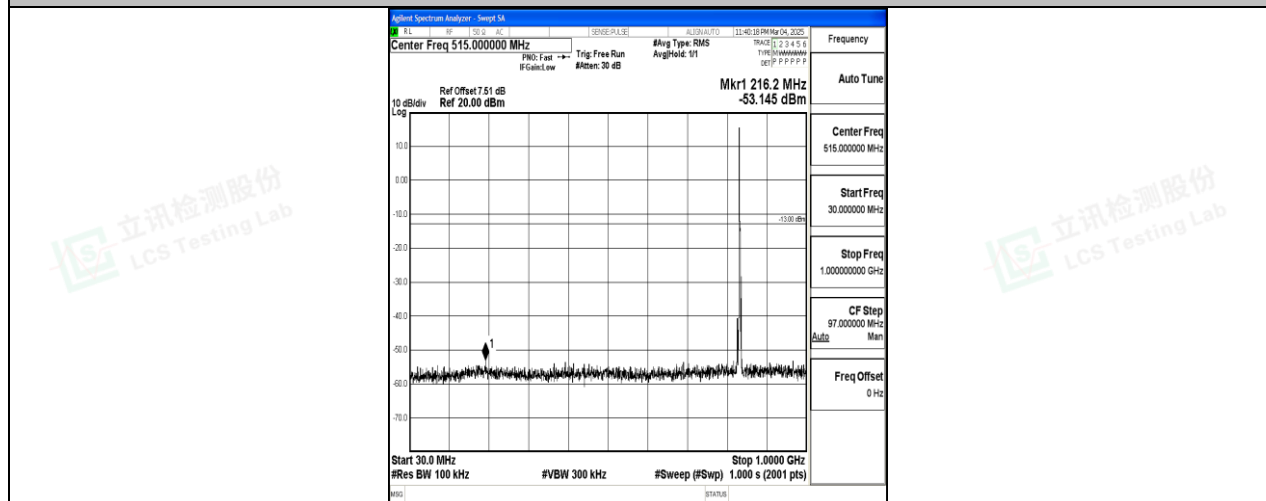
Band26_3MHz_16QAM_26915_1RB#0_30~1000_30~1000
