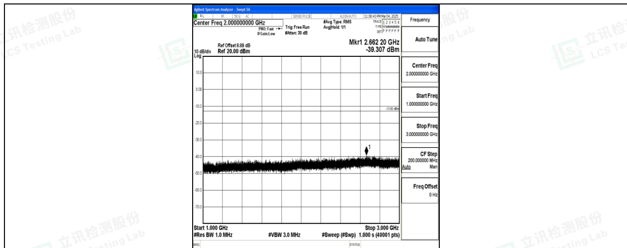
Band26_3MHz_QPSK_26805_1RB#0_1000~3000_1000~3000
