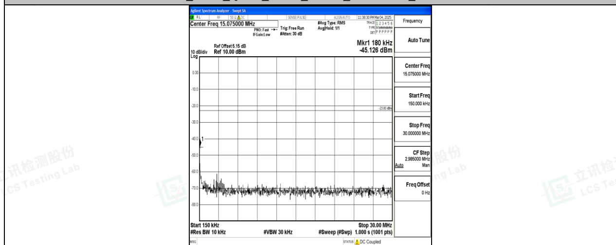
Band26_3MHz_QPSK_26805_1RB#0_0.15~30_0.15~30
