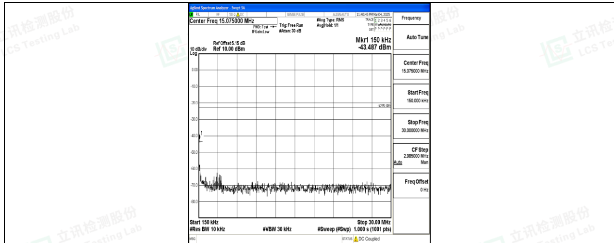
Band26_3MHz_QPSK_27025_1RB#0_0.15~30_0.15~30
