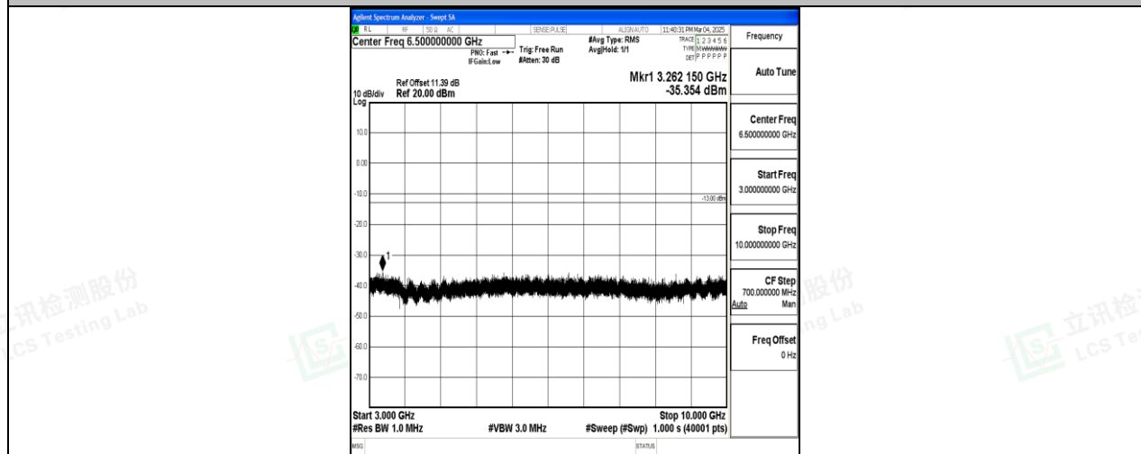
Band26_3MHz_16QAM_26915_1RB#0_3000~10000_3000~10000
