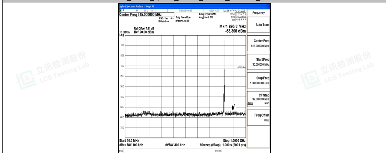
Band26_3MHz_QPSK_26805_1RB#0_30~1000_30~1000
