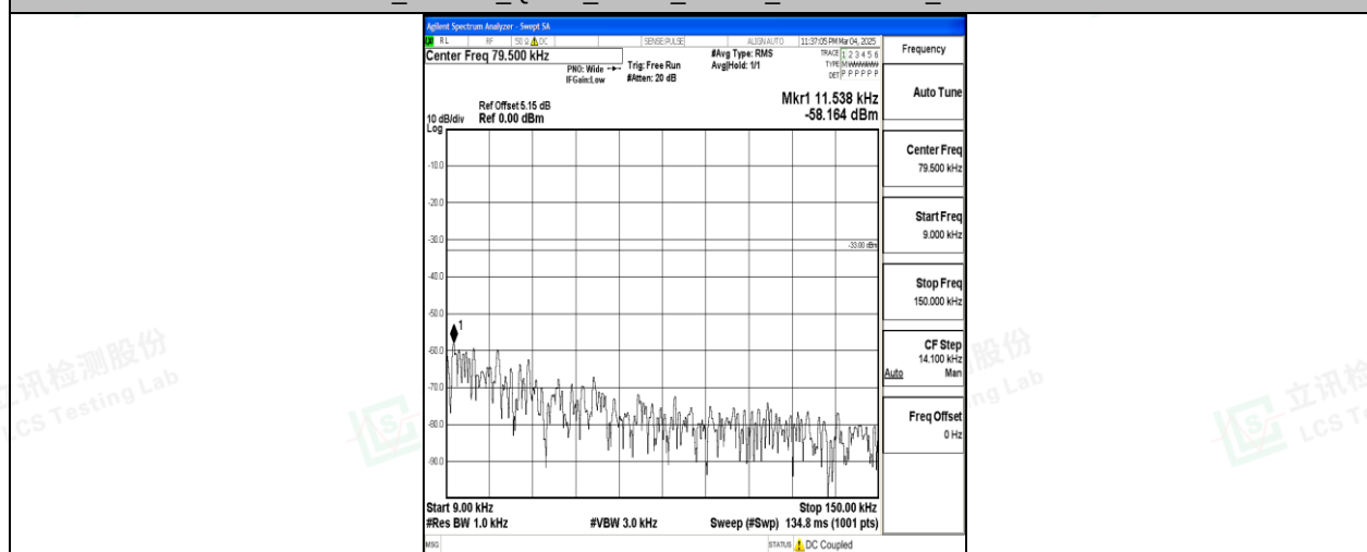
Band26_1.4MHz_16QAM_27033_1RB#0_0.009~0.15_0.009~0.15
