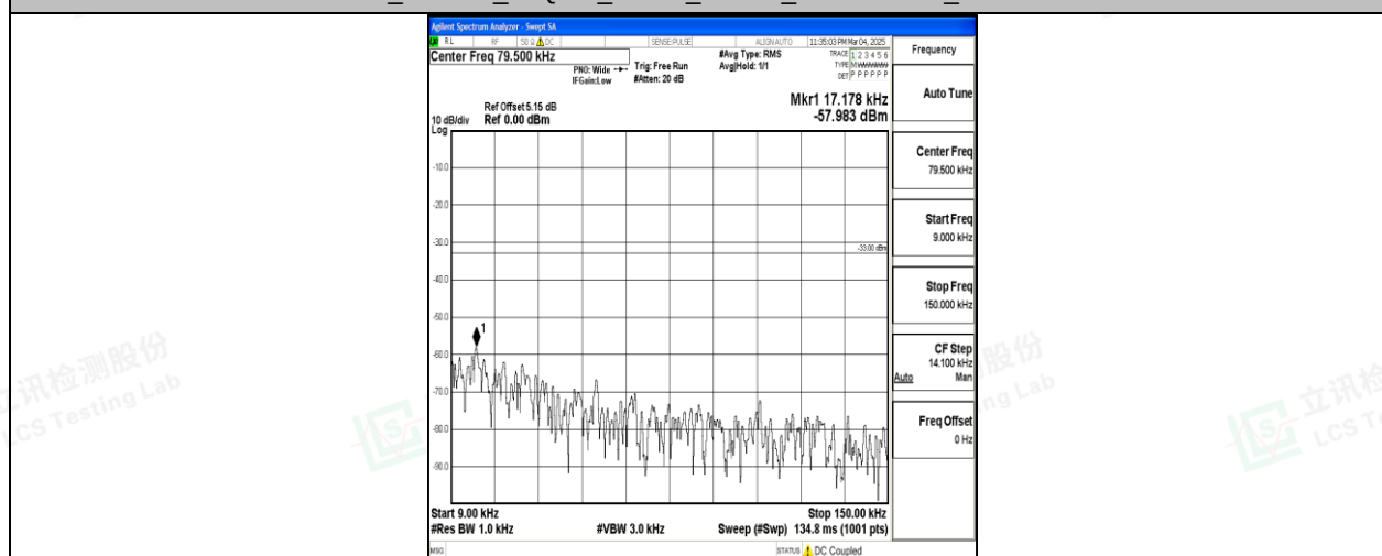
Band26_1.4MHz_QPSK_26915_1RB#0_0.009~0.15_0.009~0.15
