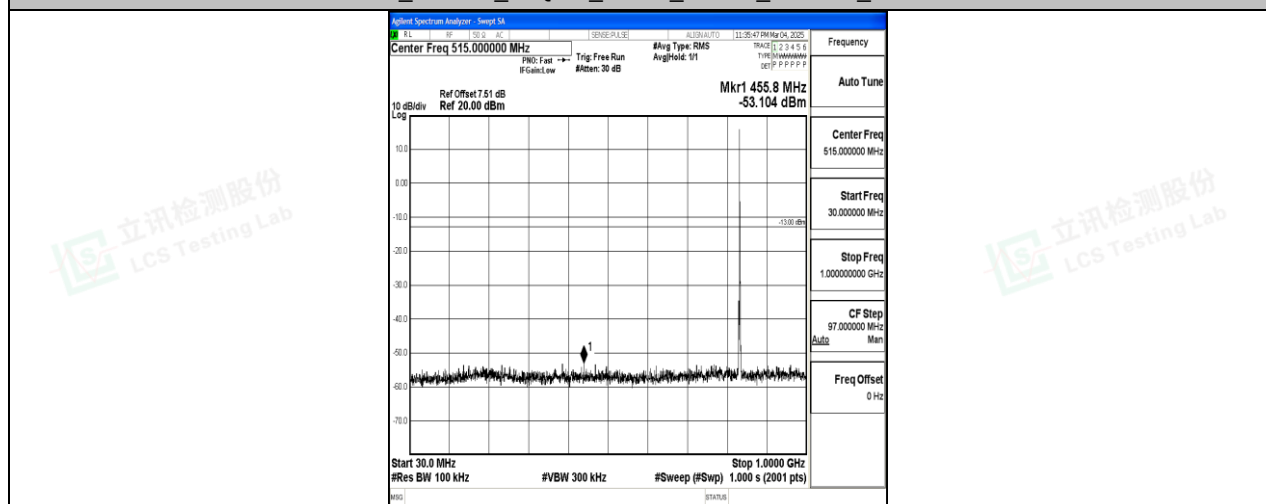
Band26_1.4MHz_16QAM_26915_1RB#0_30~1000_30~1000
