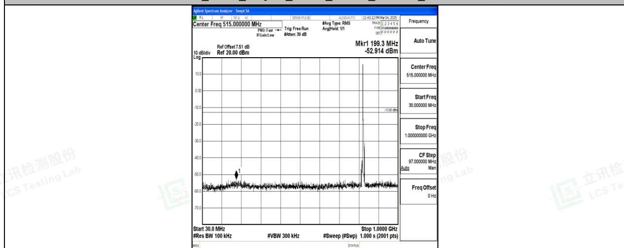
Band26_5MHz_16QAM_26815_1RB#0_30~1000_30~1000
