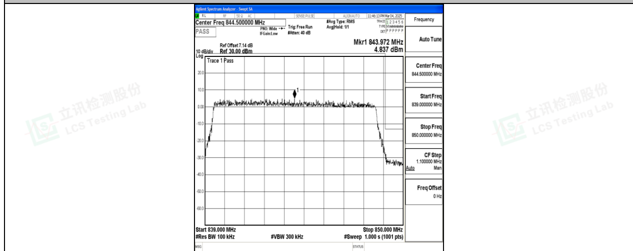
Band26_10MHz_QPSK_26990_50RB#0
