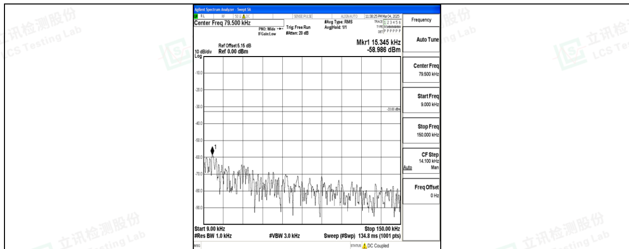
Band26_3MHz_QPSK_26805_1RB#0_0.009~0.15_0.009~0.15
