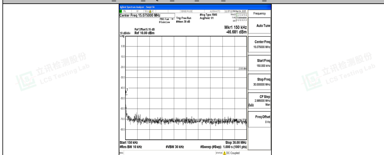
Band26_1.4MHz_16QAM_27033_1RB#0_0.15~30_0.15~30
