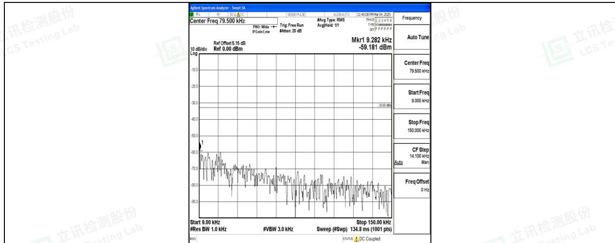
Band26_3MHz_16QAM_26915_1RB#0_0.009~0.15_0.009~0.15
