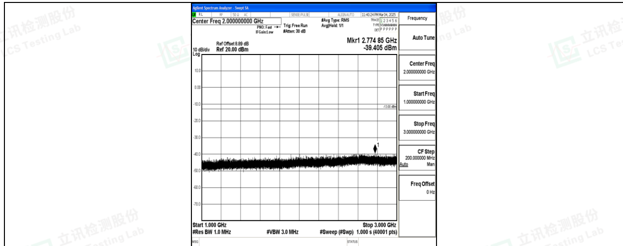
Band26_3MHz_16QAM_26915_1RB#0_1000~3000_1000~3000
