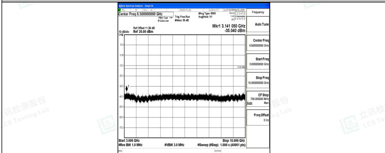
Band26_5MHz_QPSK_26740_1RB#0_3000~10000_3000~10000
