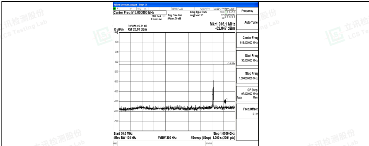
Band26_3MHz_16QAM_26705_1RB#0_30~1000_30~1000
