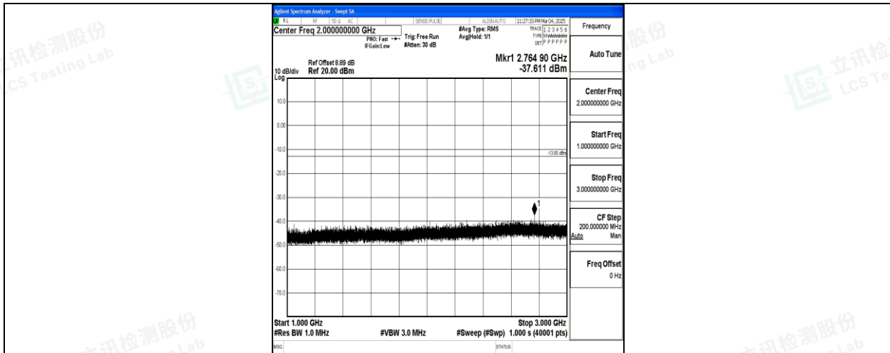
Band26_5MHz_QPSK_26740_1RB#0_1000~3000_1000~3000
