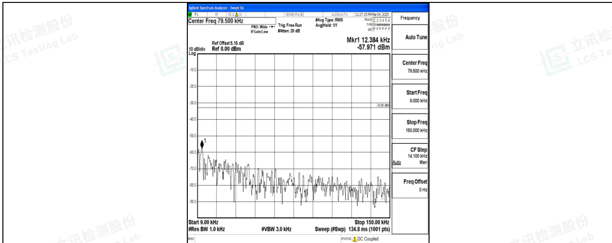
Band26_5MHz_QPSK_26740_1RB#0_0.009~0.15_0.009~0.15
