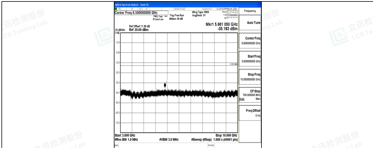
Band26_3MHz_16QAM_26740_1RB#0_3000~10000_3000~10000
