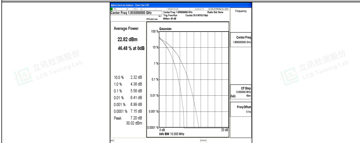
Band25-10MHz-QPSK-26090-50RB#0-PASS
