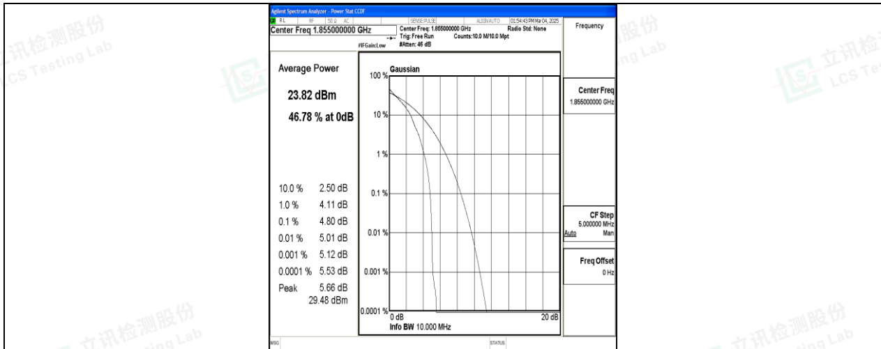
Band25-10MHz-QPSK-26090-1RB#0-PASS
