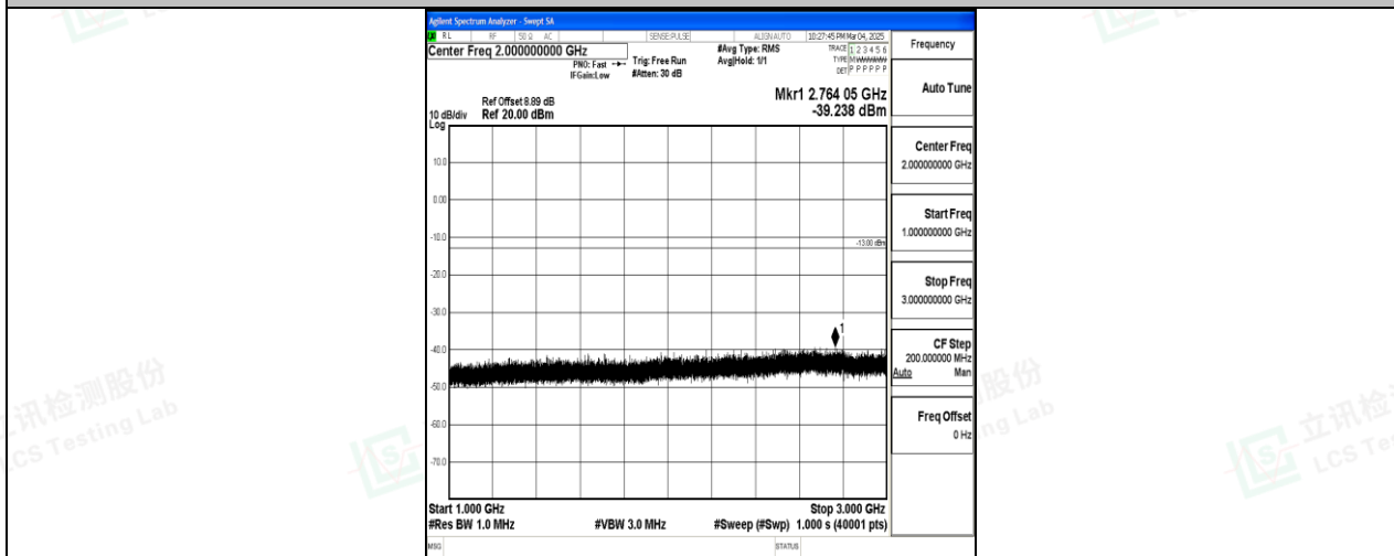
Band12_10MHz_QPSK_23095_1RB#0_1000~3000_1000~3000
