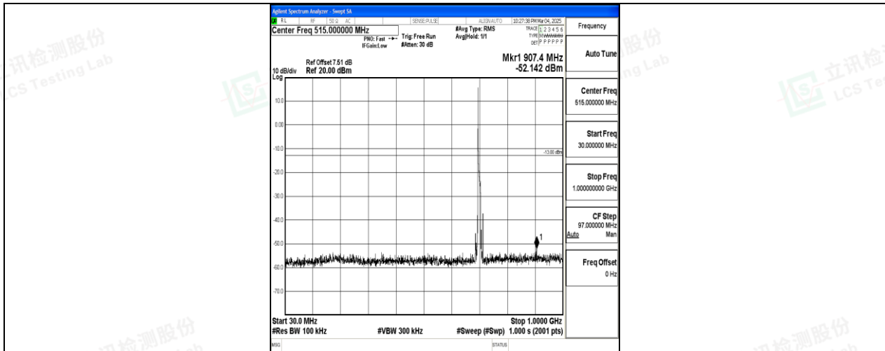
Band12_10MHz_QPSK_23095_1RB#0_30~1000_30~1000
