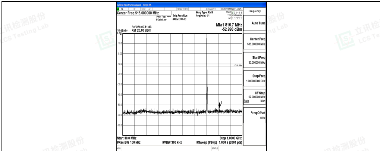
Band12_3MHz_16QAM_23165_1RB#0_30~1000_30~1000
