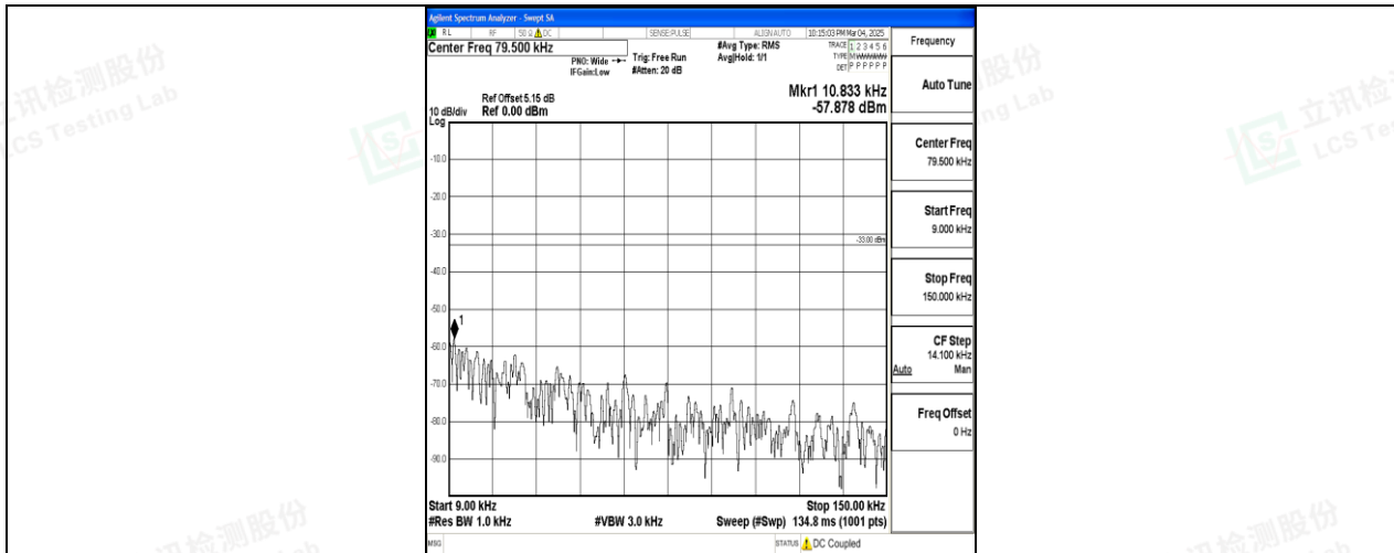
Band12_1.4MHz_16QAM_23095_1RB#0_0.009~0.15_0.009~0.15
