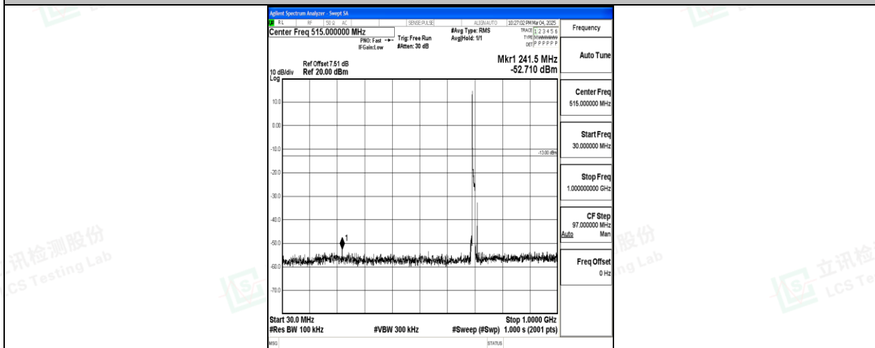
Band12_10MHz_16QAM_23060_1RB#0_30~1000_30~1000
