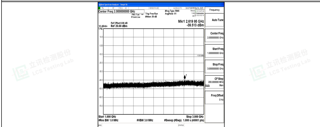
Band12_10MHz_16QAM_23060_1RB#0_1000~3000_1000~3000
