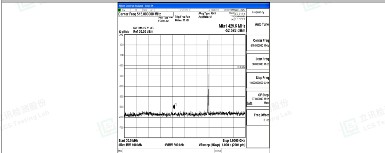
Band12_3MHz_16QAM_23025_1RB#0_30~1000_30~1000
