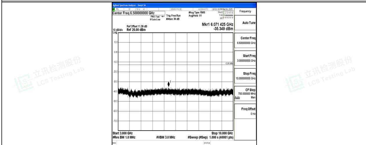
Band12_3MHz_16QAM_23165_1RB#0_3000~10000_3000~10000
