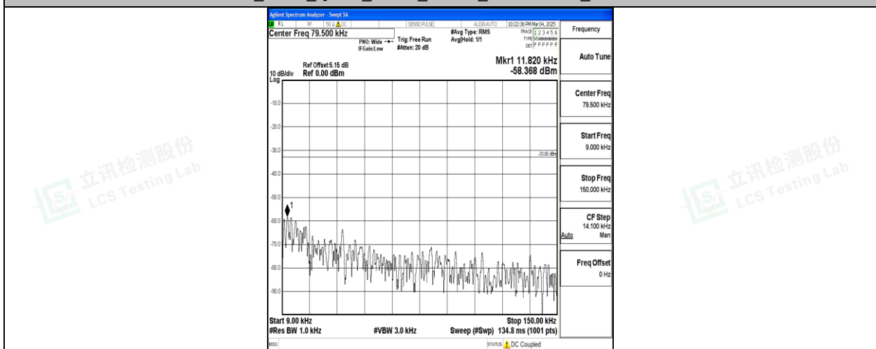
Band12_5MHz_16QAM_23035_1RB#0_0.009~0.15_0.009~0.15
