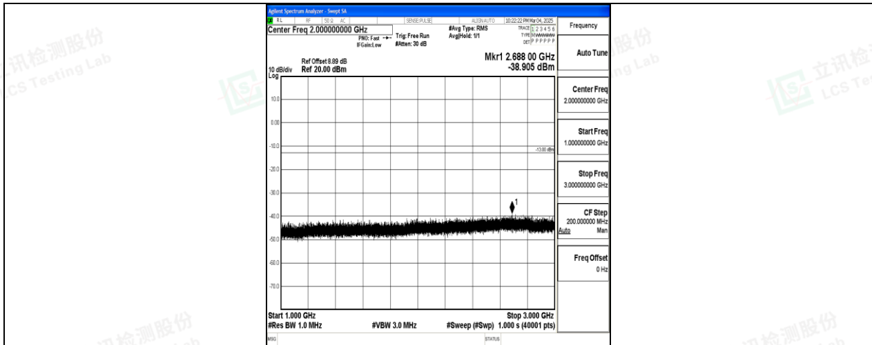
Band12_5MHz_QPSK_23035_1RB#0_1000~3000_1000~3000
