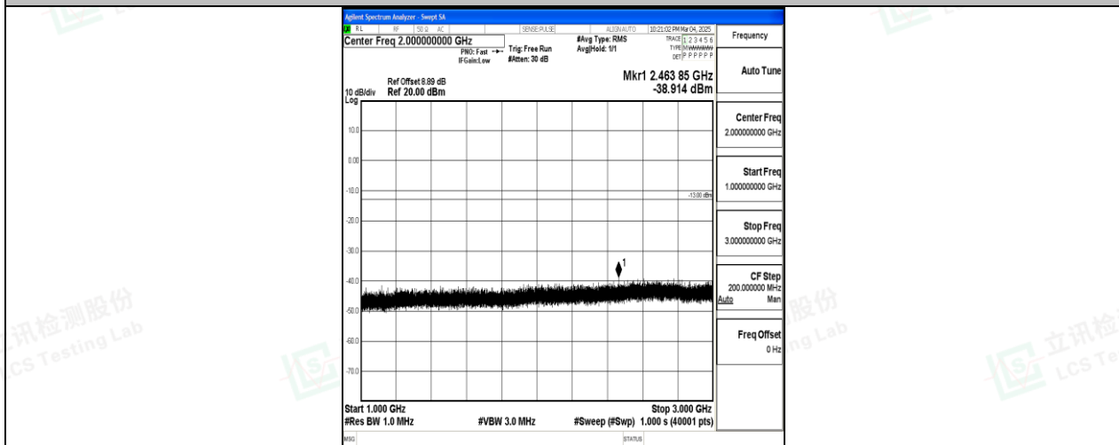
Band12_3MHz_16QAM_23165_1RB#0_1000~3000_1000~3000
