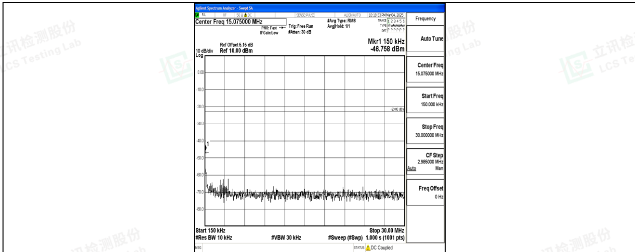
Band12_3MHz_16QAM_23025_1RB#0_0.15~30_0.15~30
