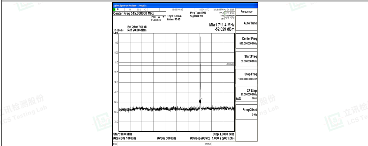
Band12_1.4MHz_QPSK_23173_1RB#0_30~1000_30~1000
