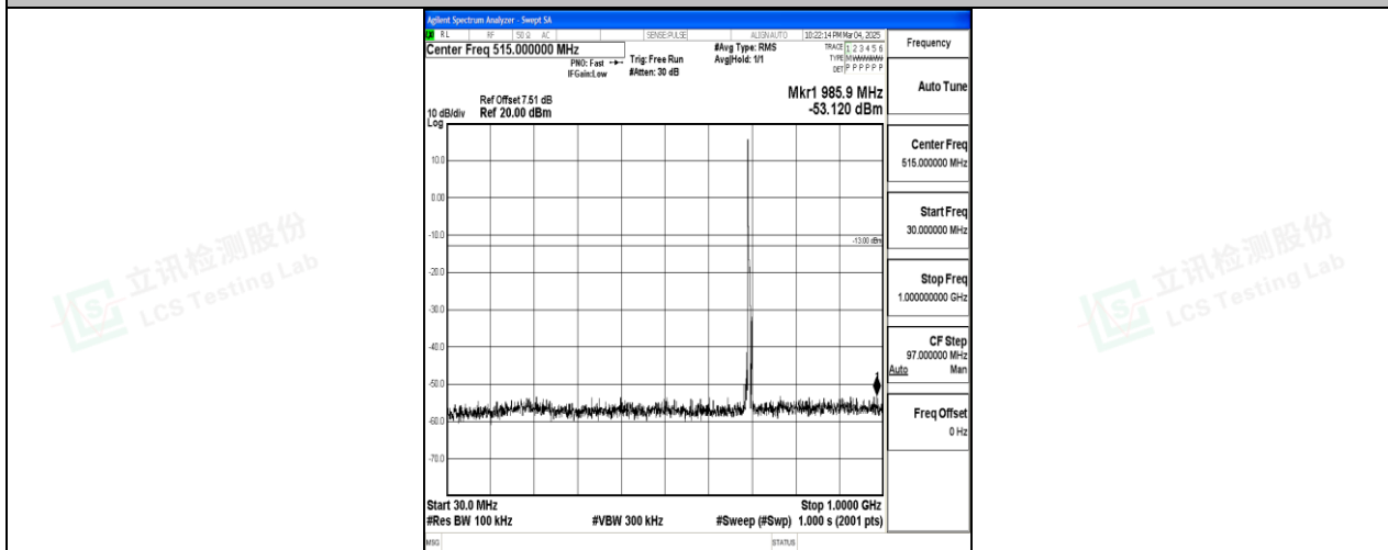
Band12_5MHz_QPSK_23035_1RB#0_30~1000_30~1000
