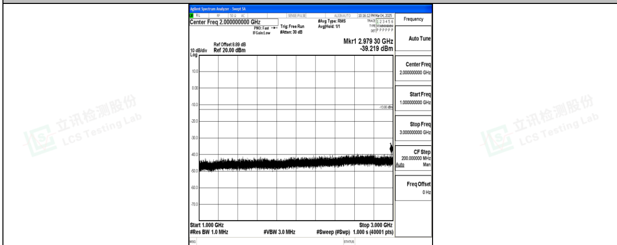
Band12_1.4MHz_QPSK_23173_1RB#0_1000~3000_1000~3000
