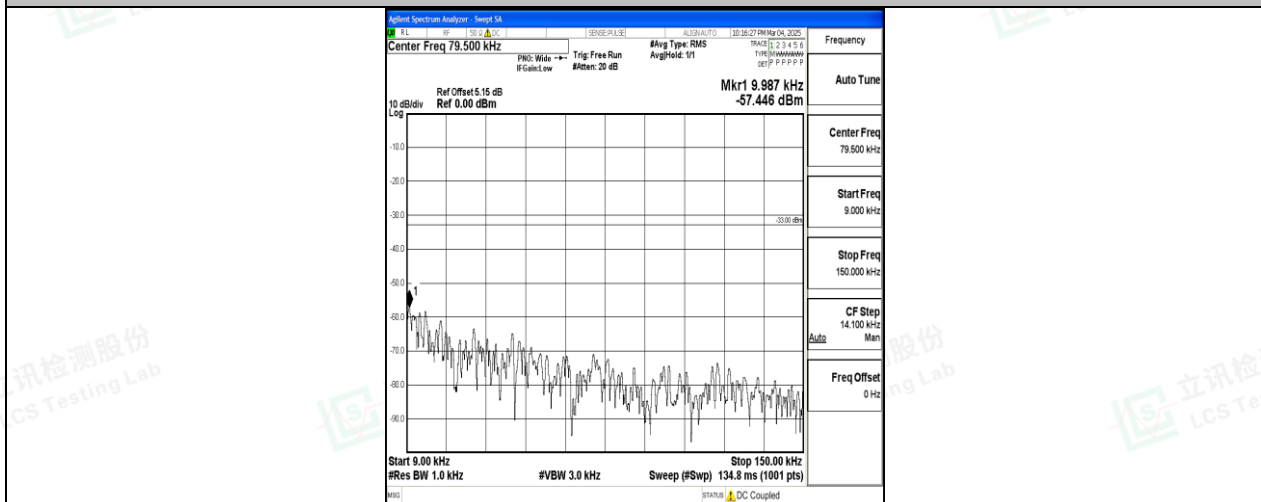
Band12_1.4MHz_16QAM_23173_1RB#0_0.009~0.15_0.009~0.15
