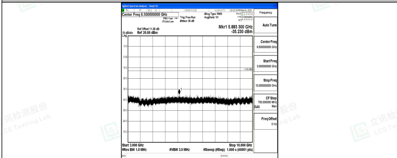
Band12_5MHz_QPSK_23035_1RB#0_3000~10000_3000~10000
