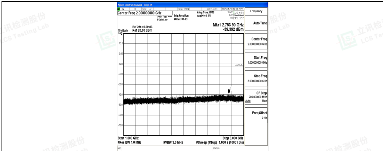
Band12_10MHz_QPSK_23060_1RB#0_1000~3000_1000~3000
