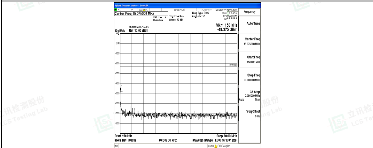
Band12_1.4MHz_16QAM_23095_1RB#0_0.15~30_0.15~30
