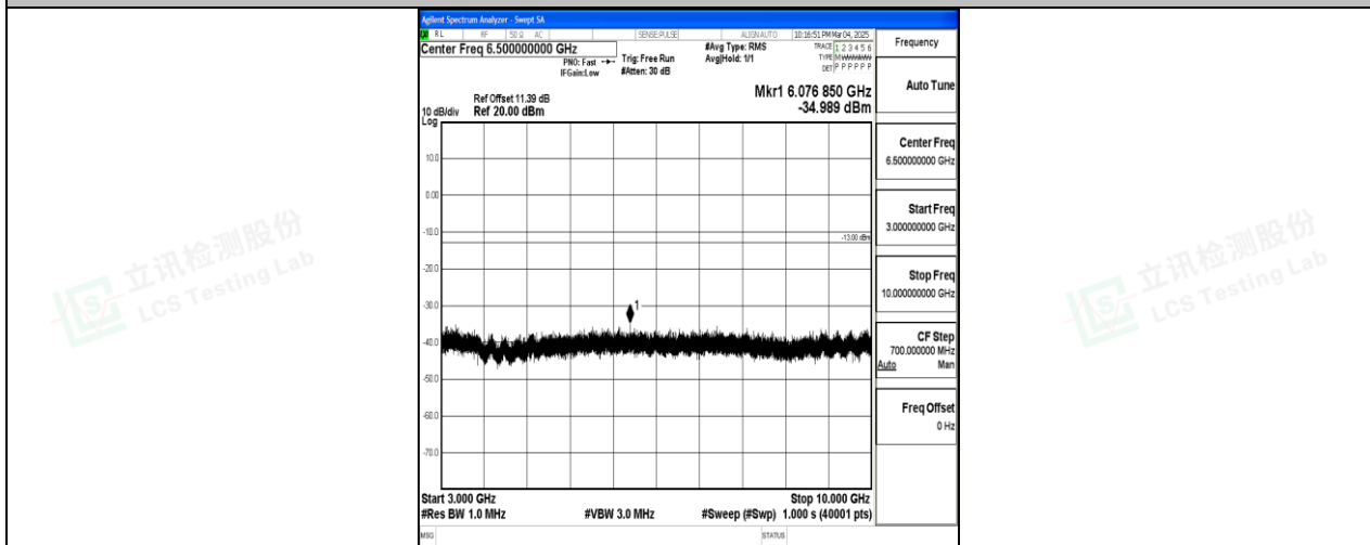
Band12_1.4MHz_16QAM_23173_1RB#0_3000~10000_3000~10000
