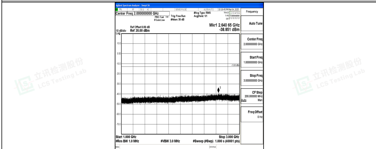
Band12_3MHz_16QAM_23025_1RB#0_1000~3000_1000~3000
