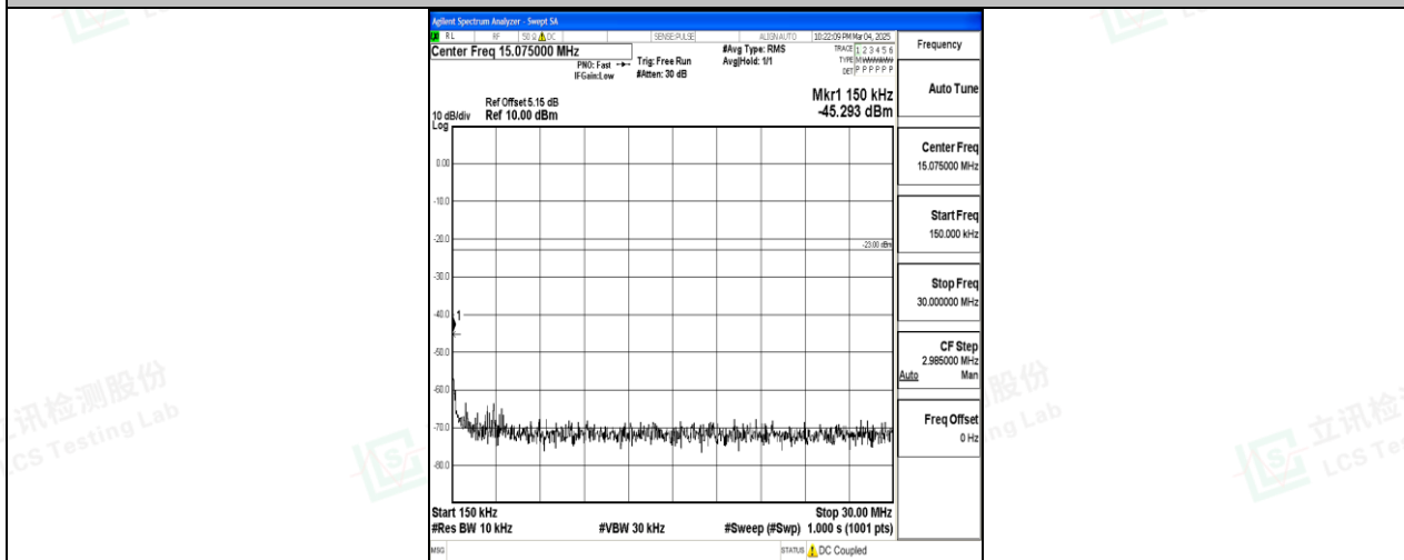
Band12_5MHz_QPSK_23035_1RB#0_0.15~30_0.15~30
