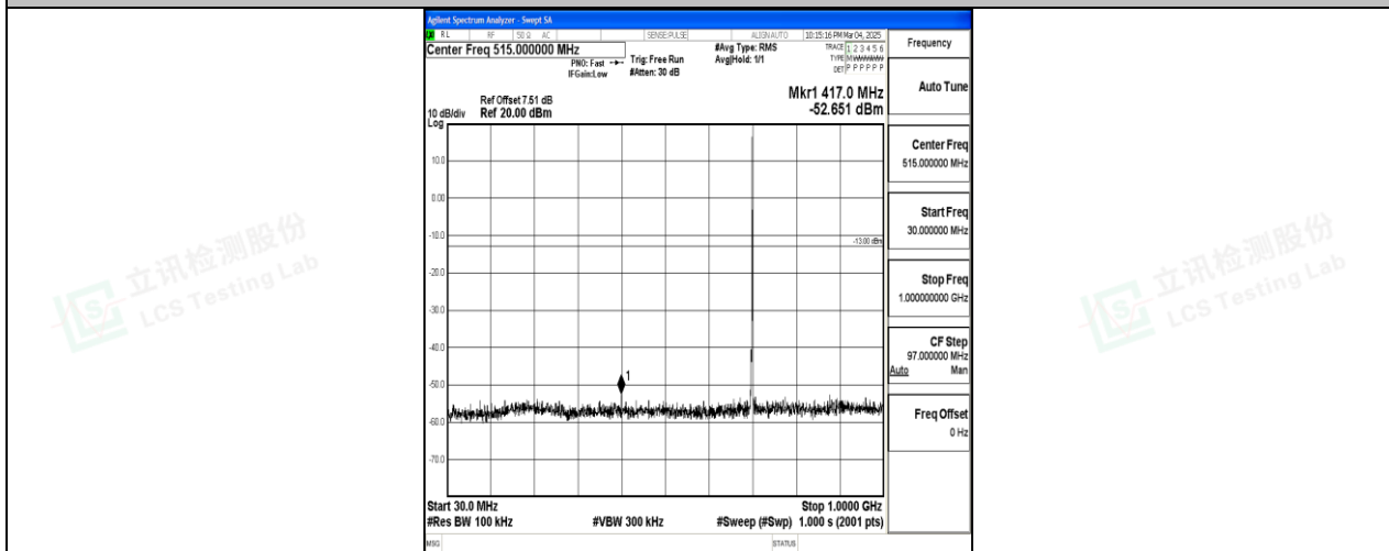
Band12_1.4MHz_16QAM_23095_1RB#0_30~1000_30~1000
