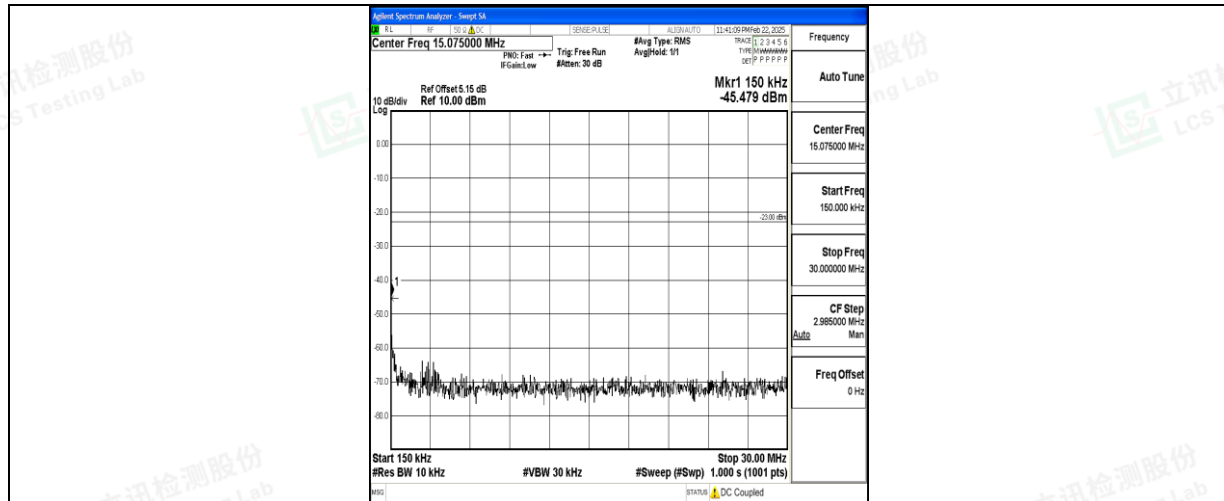
Band5_10MHz_QPSK_20600_1RB#0_0.15~30_0.15~30
