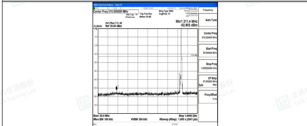
Band5_10MHz_QPSK_20600_1RB#0_30~1000_30~1000
