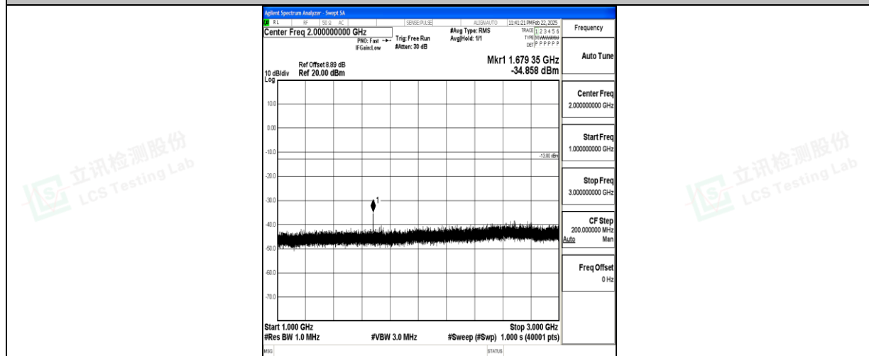
Band5_10MHz_QPSK_20600_1RB#0_1000~3000_1000~3000
