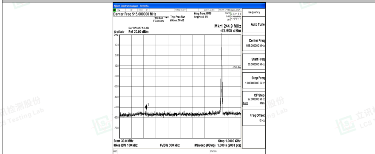
Band5_5MHz_QPSK_20625_1RB#0_30~1000_30~1000
