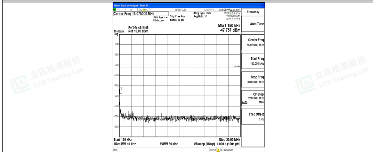
Band5_1.4MHz_QPSK_20525_1RB#0_0.15~30_0.15~30
