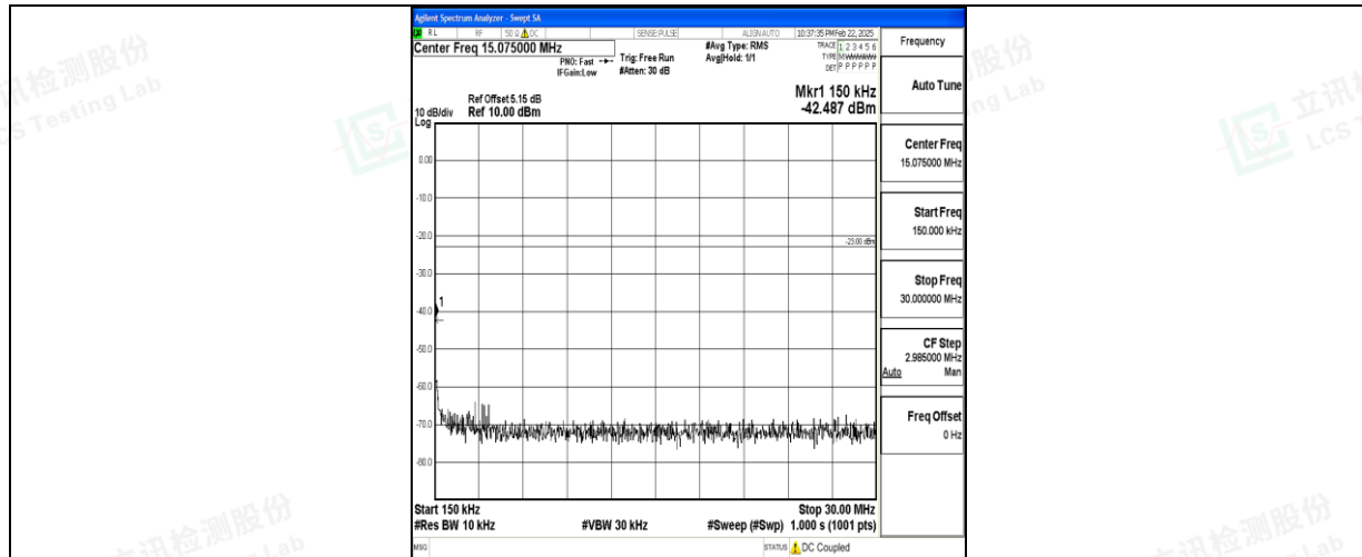
Band5_1.4MHz_QPSK_20643_1RB#0_0.15~30_0.15~30
