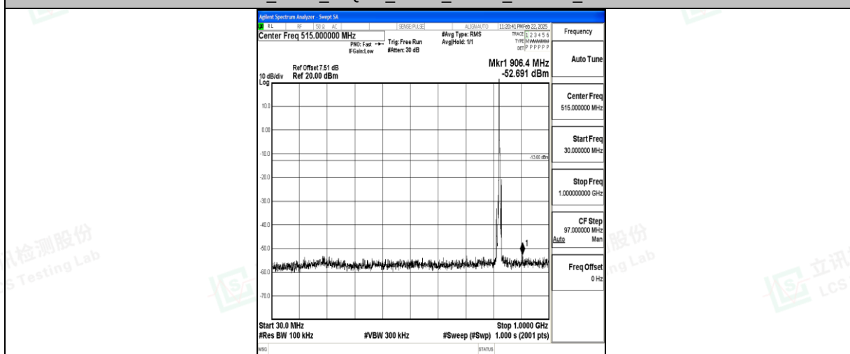
Band5_5MHz_16QAM_20425_1RB#0_30~1000_30~1000
