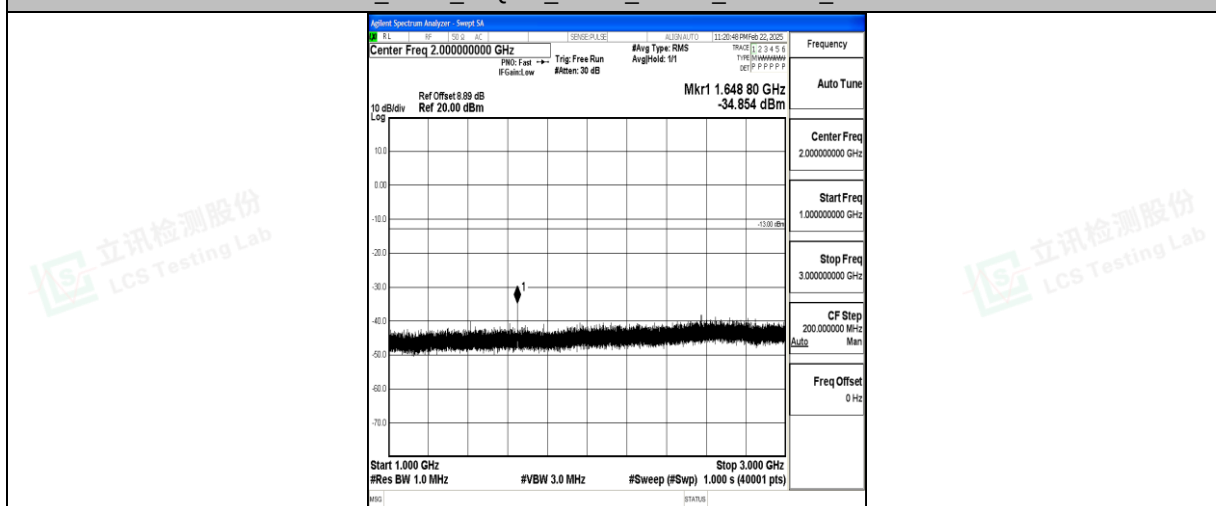
Band5_5MHz_16QAM_20425_1RB#0_1000~3000_1000~3000
