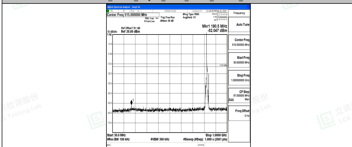
Band5_10MHz_16QAM_20450_1RB#0_30~1000_30~1000
