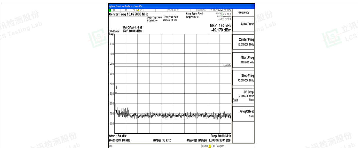
Band5_3MHz_QPSK_20635_1RB#0_0.15~30_0.15~30
