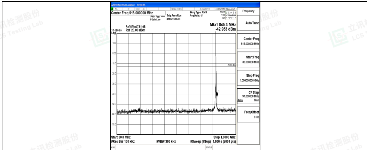
Band5_3MHz_QPSK_20525_1RB#0_30~1000_30~1000
