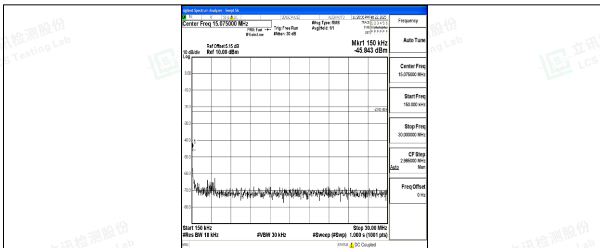
Band5_5MHz_16QAM_20425_1RB#0_0.15~30_0.15~30
