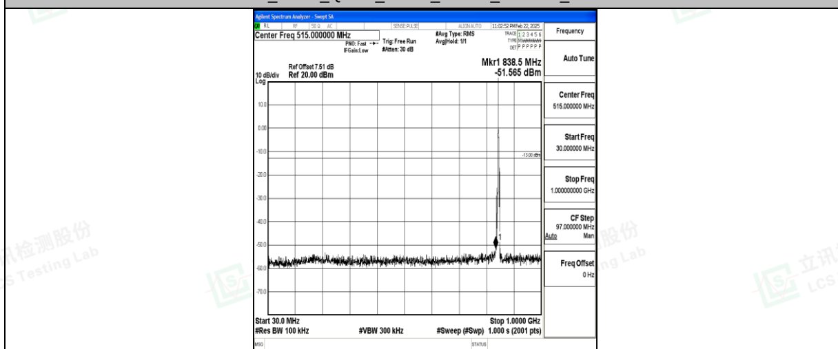
Band5_3MHz_QPSK_20635_1RB#0_30~1000_30~1000
