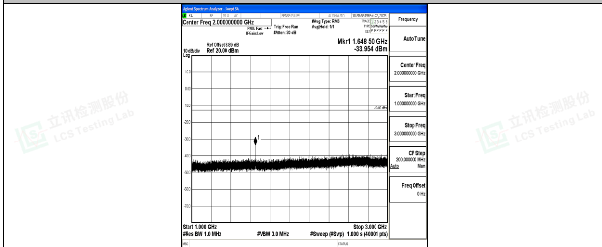
Band5_1.4MHz_16QAM_20407_1RB#0_1000~3000_1000~3000
