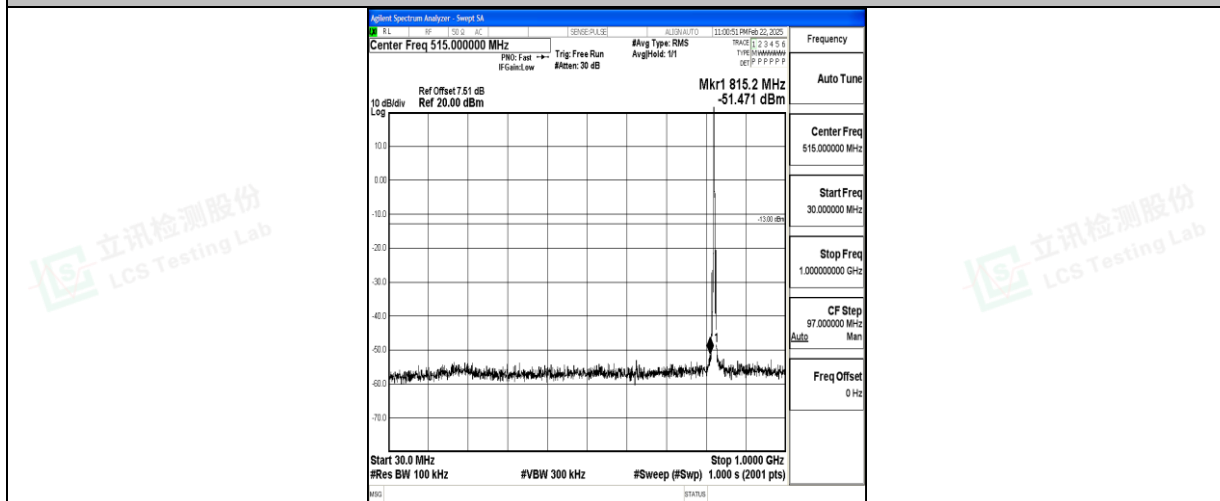
Band5_3MHz_QPSK_20415_1RB#0_30~1000_30~1000
