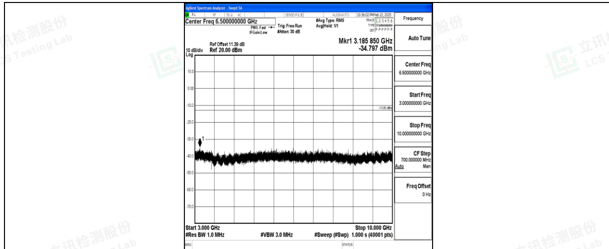
Band5_1.4MHz_16QAM_20407_1RB#0_3000~10000_3000~10000
