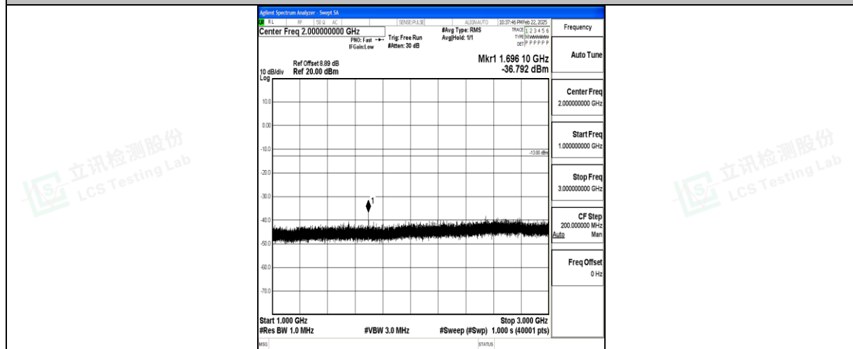
Band5_1.4MHz_QPSK_20643_1RB#0_1000~3000_1000~3000
