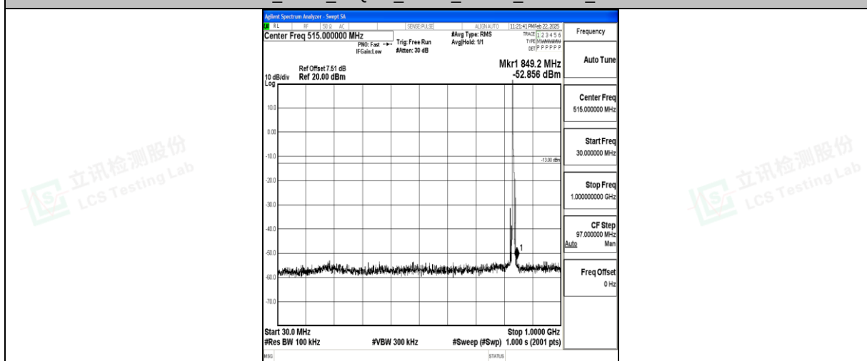
Band5_5MHz_16QAM_20525_1RB#0_30~1000_30~1000
