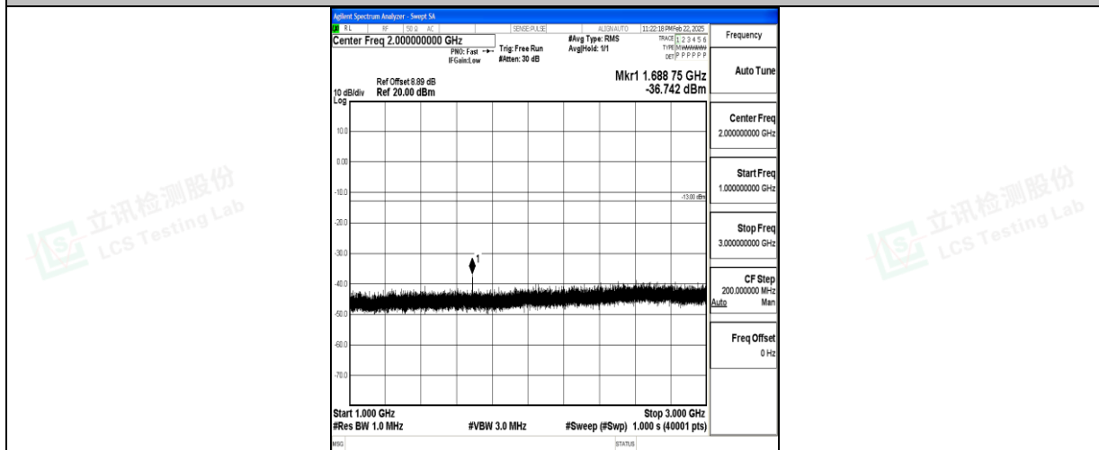
Band5_5MHz_QPSK_20625_1RB#0_1000~3000_1000~3000
