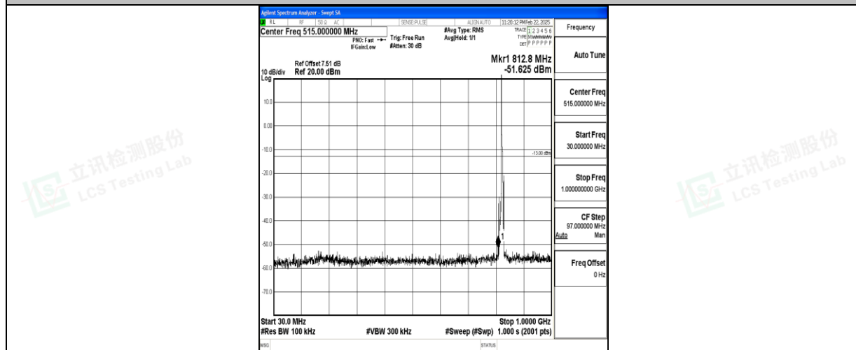
Band5_5MHz_QPSK_20425_1RB#0_30~1000_30~1000
