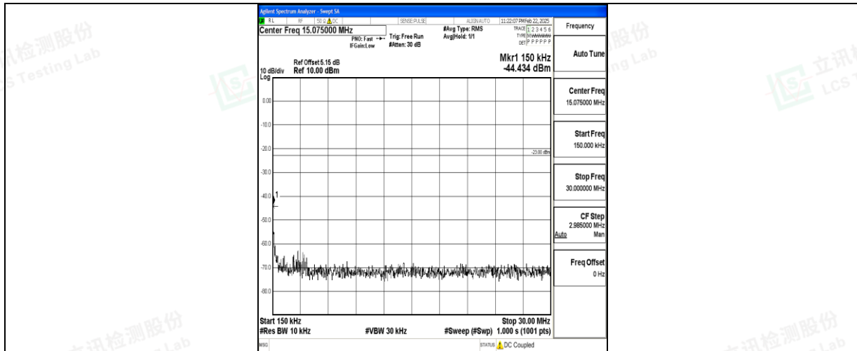
Band5_5MHz_QPSK_20625_1RB#0_0.15~30_0.15~30
