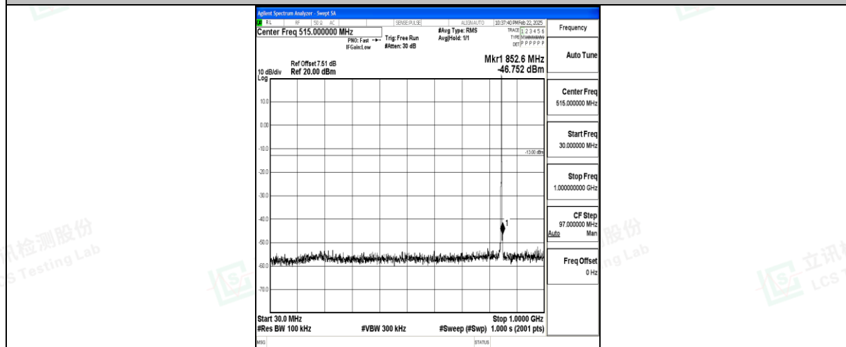
Band5_1.4MHz_QPSK_20643_1RB#0_30~1000_30~1000
