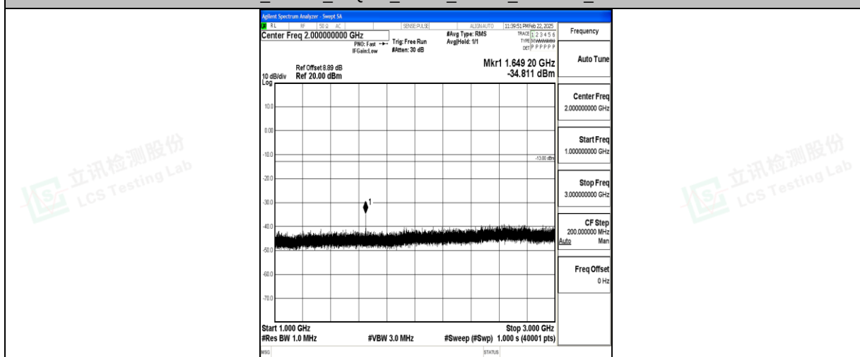
Band5_10MHz_16QAM_20450_1RB#0_1000~3000_1000~3000
