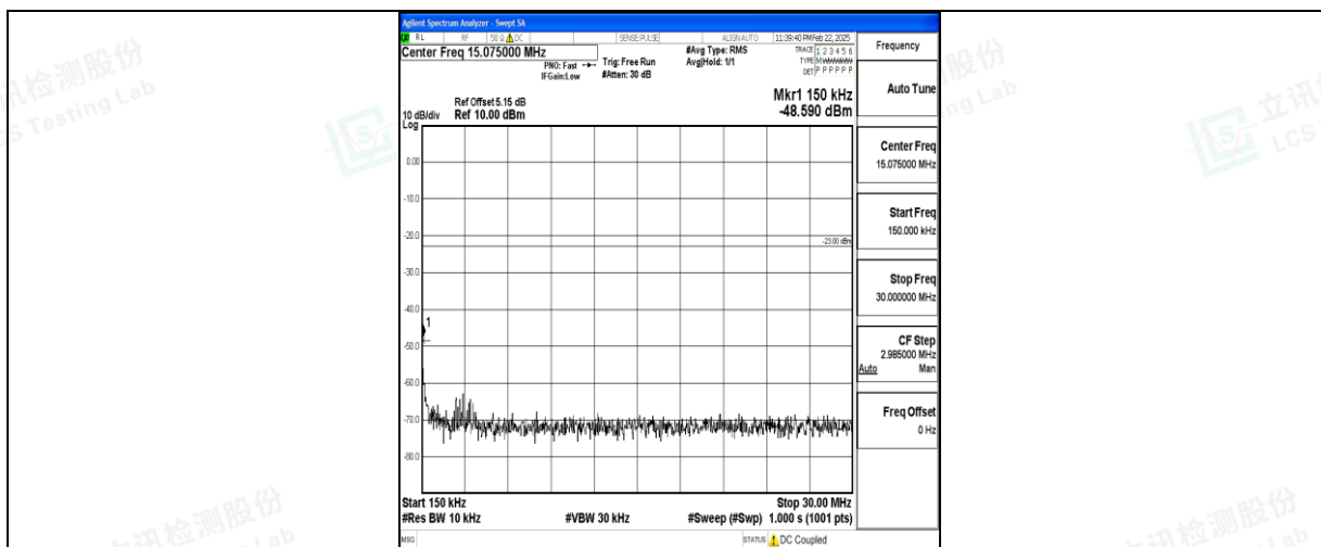
Band5_10MHz_16QAM_20450_1RB#0_0.15~30_0.15~30
