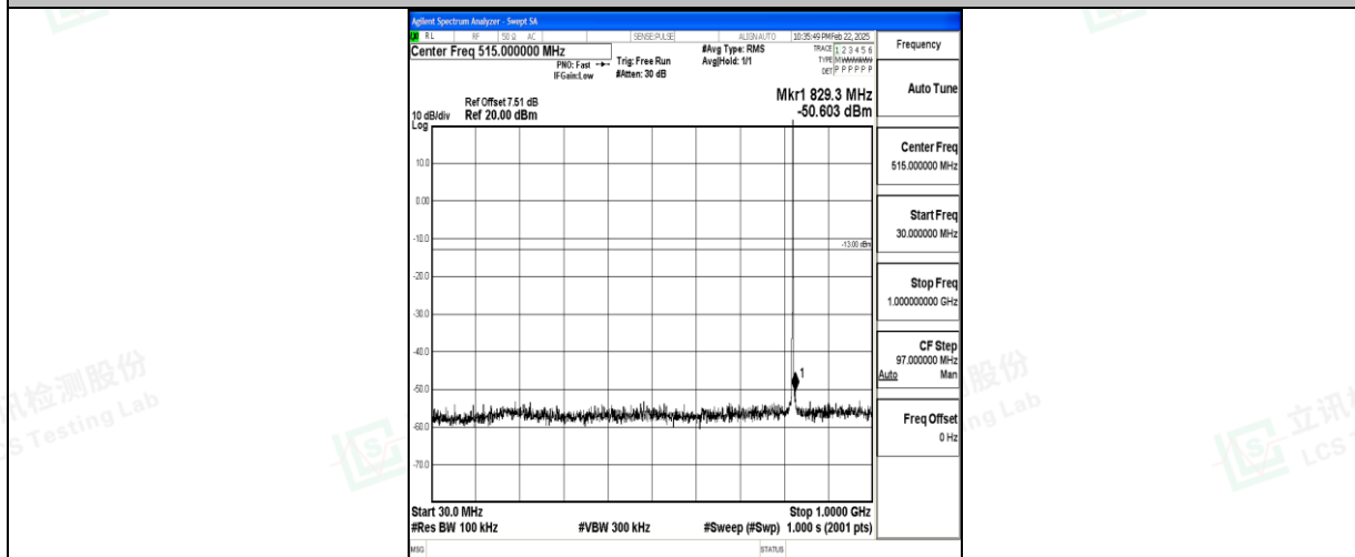
Band5_1.4MHz_16QAM_20407_1RB#0_30~1000_30~1000
