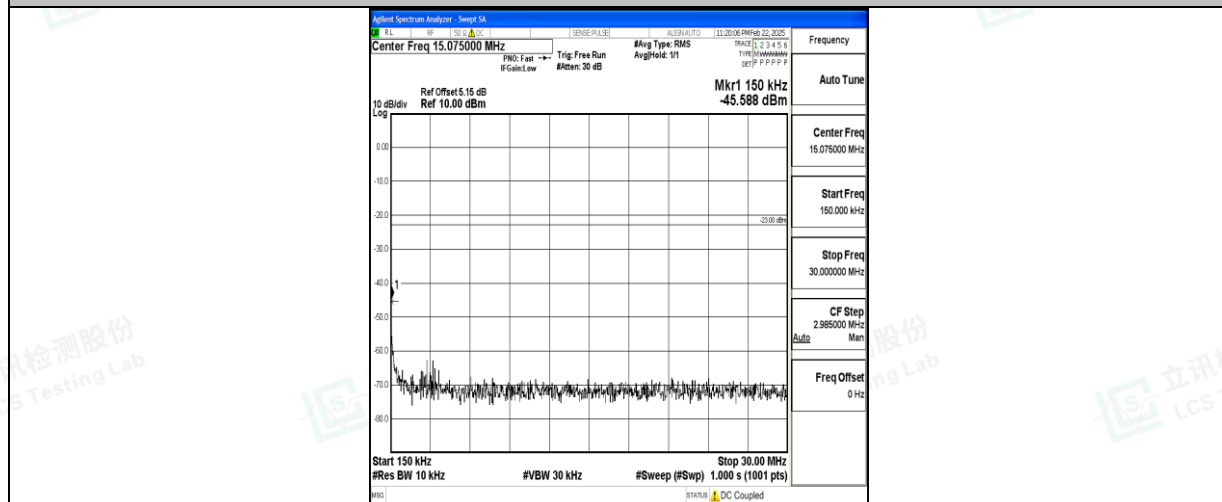
Band5_5MHz_QPSK_20425_1RB#0_0.15~30_0.15~30
