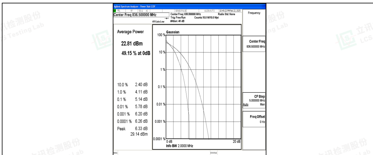
Band5-1.4MHz-QPSK-20525-6RB#0-PASS
