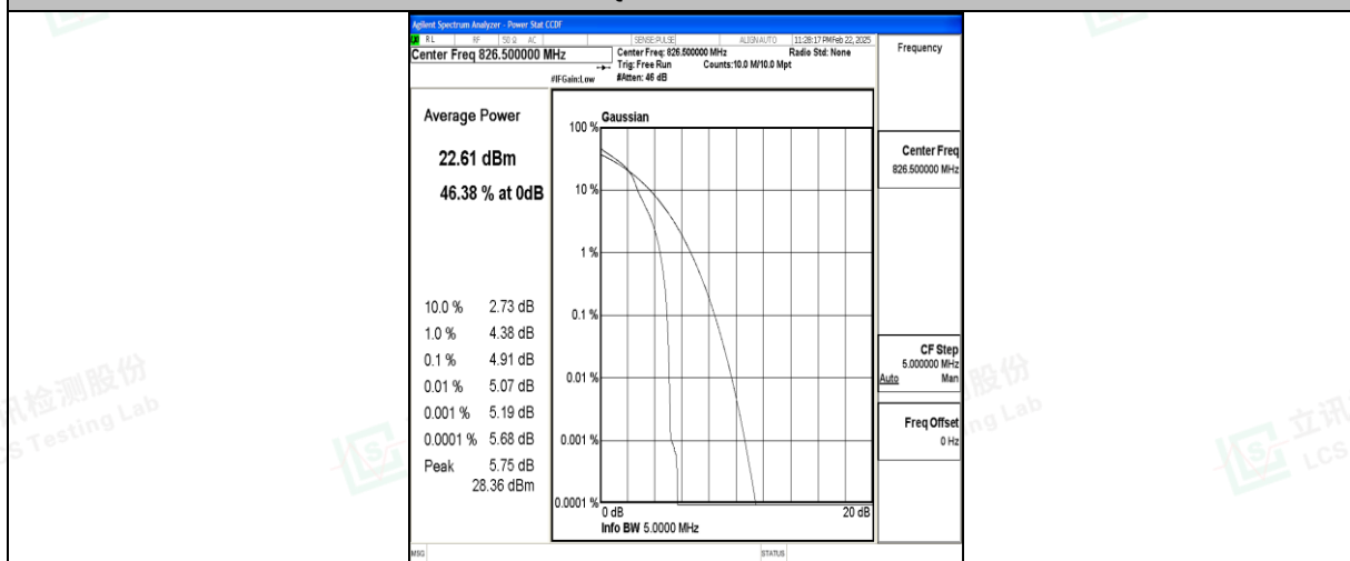
Band5-5MHz-16QAM-20425-1RB#0-PASS
