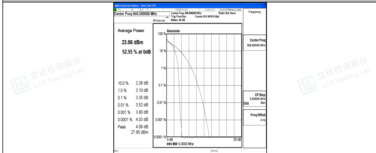
Band5-5MHz-QPSK-20625-1RB#0-PASS
