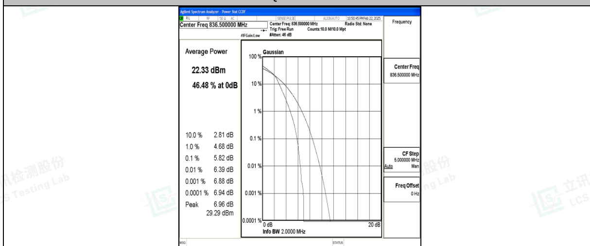
Band5-1.4MHz-16QAM-20525-6RB#0-PASS
