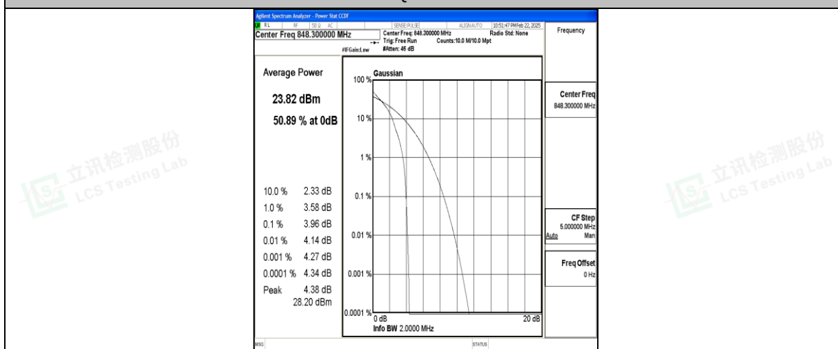
Band5-1.4MHz-QPSK-20643-1RB#0-PASS
