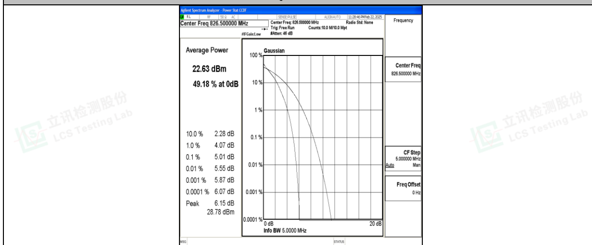
Band5-5MHz-QPSK-20425-25RB#0-PASS
