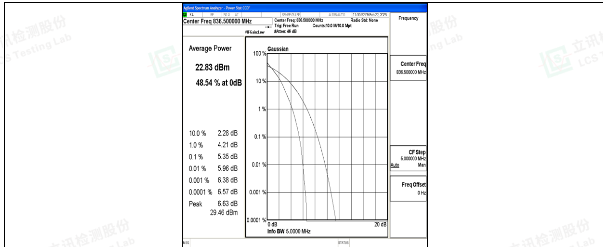
Band5-5MHz-QPSK-20525-25RB#0-PASS
