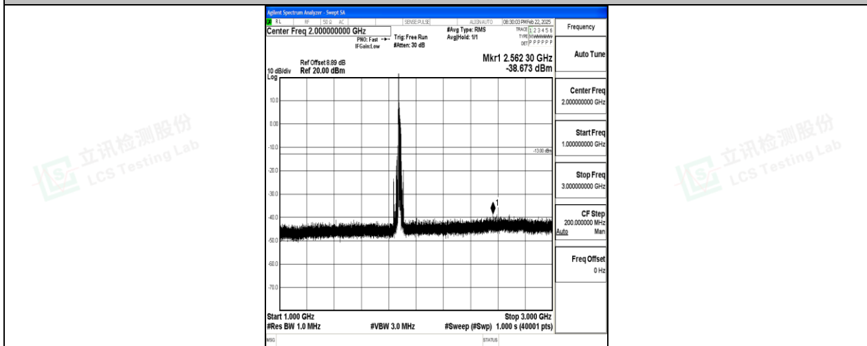
Band2_20MHz_16QAM_18900_1RB#0_1000~3000_1000~3000
