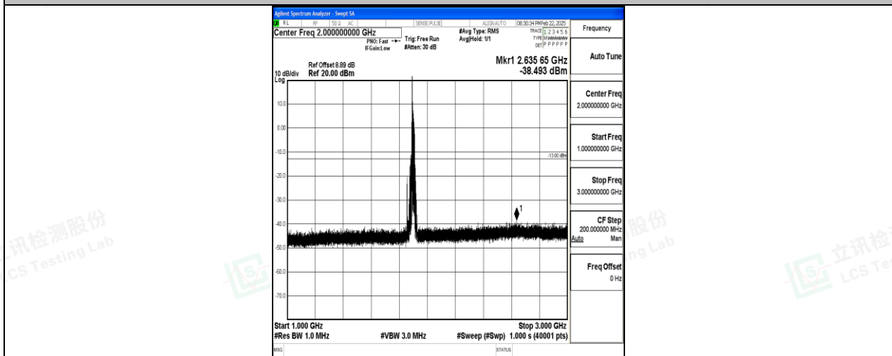
Band2_20MHz_QPSK_19100_1RB#0_1000~3000_1000~3000
