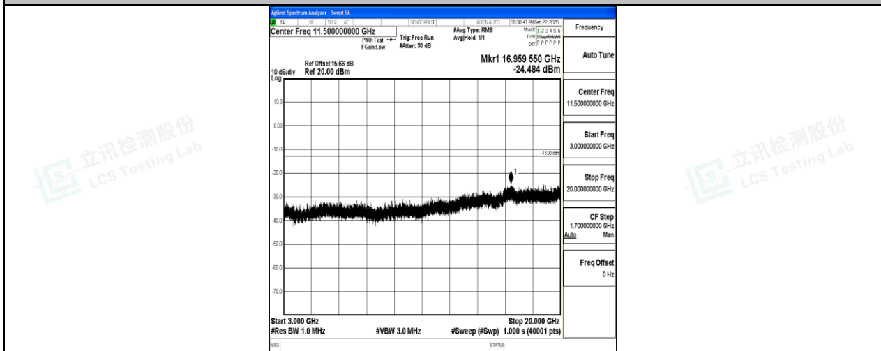
Band2_20MHz_QPSK_19100_1RB#0_3000~20000_3000~20000
