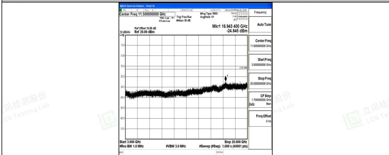
Band2_15MHz_QPSK_18900_1RB#0_3000~20000_3000~20000
