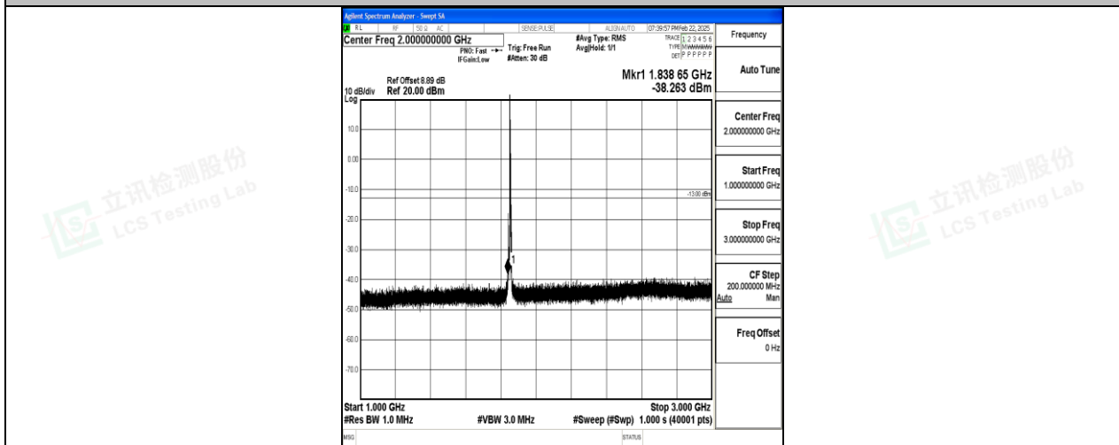
Band2_5MHz_QPSK_18625_1RB#0_1000~3000_1000~3000
