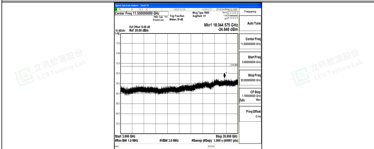
Band2_5MHz_QPSK_19175_1RB#0_3000~20000_3000~20000
