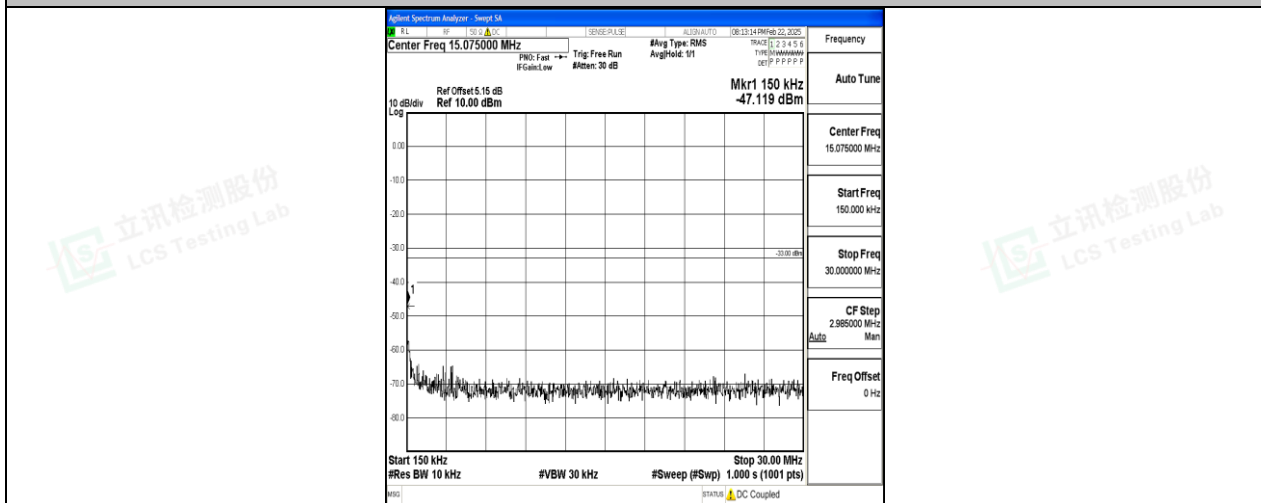
Band2_15MHz_16QAM_18675_1RB#0_0.15~30_0.15~30
