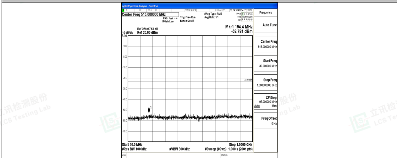
Band2_5MHz_QPSK_18625_1RB#0_30~1000_30~1000
