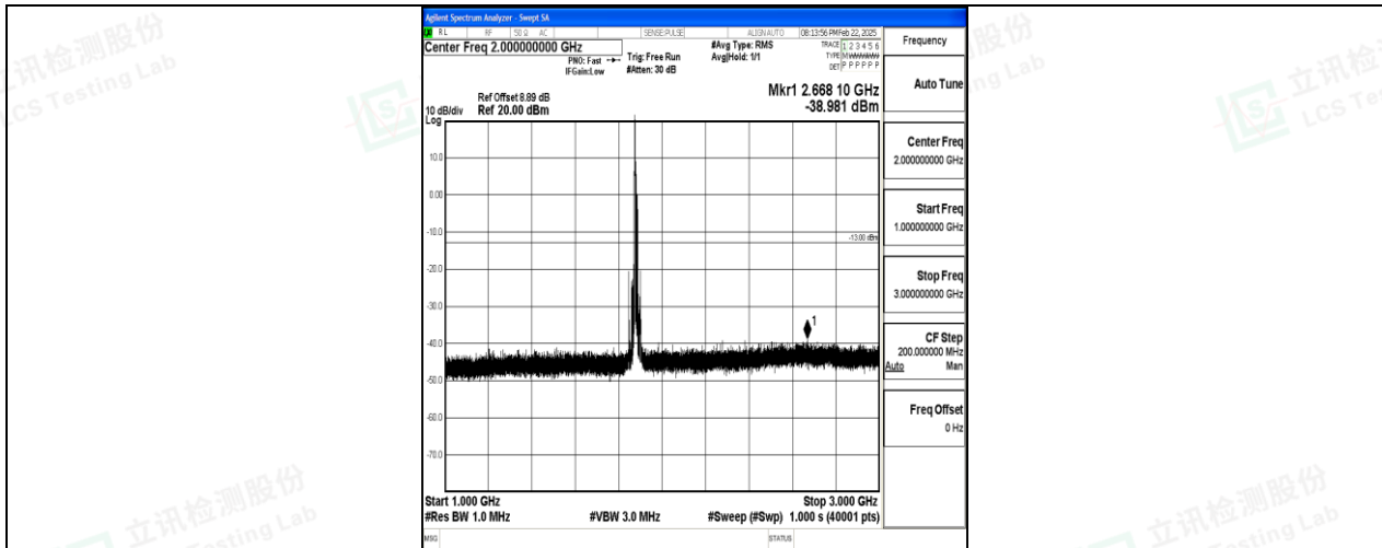
Band2_15MHz_QPSK_18900_1RB#0_1000~3000_1000~3000
