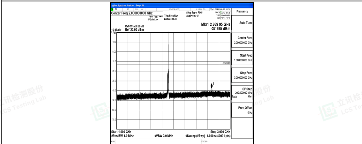
Band2_5MHz_QPSK_19175_1RB#0_1000~3000_1000~3000
