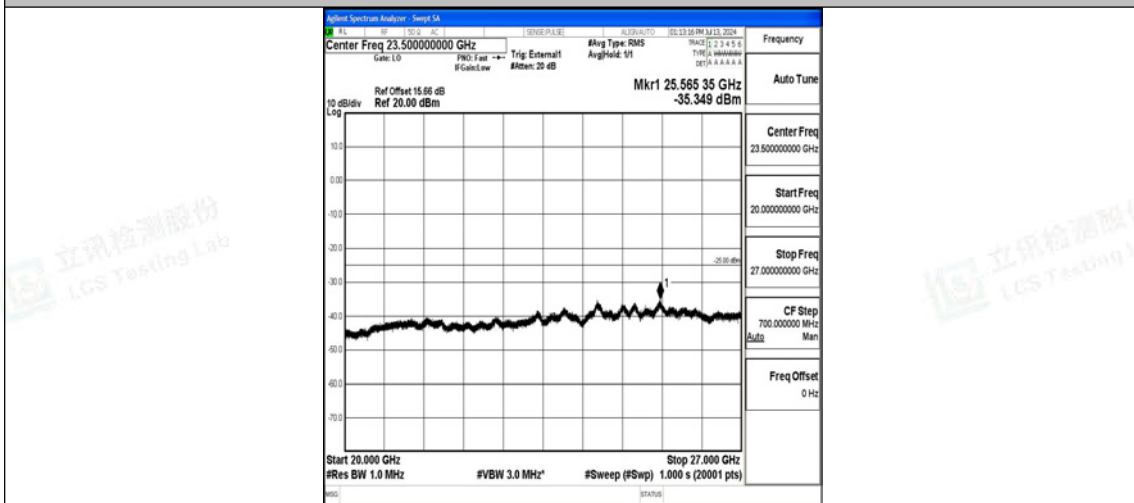
Band41_20MHz_16QAM_41490_1RB#0_20000~27000_20000~27000
