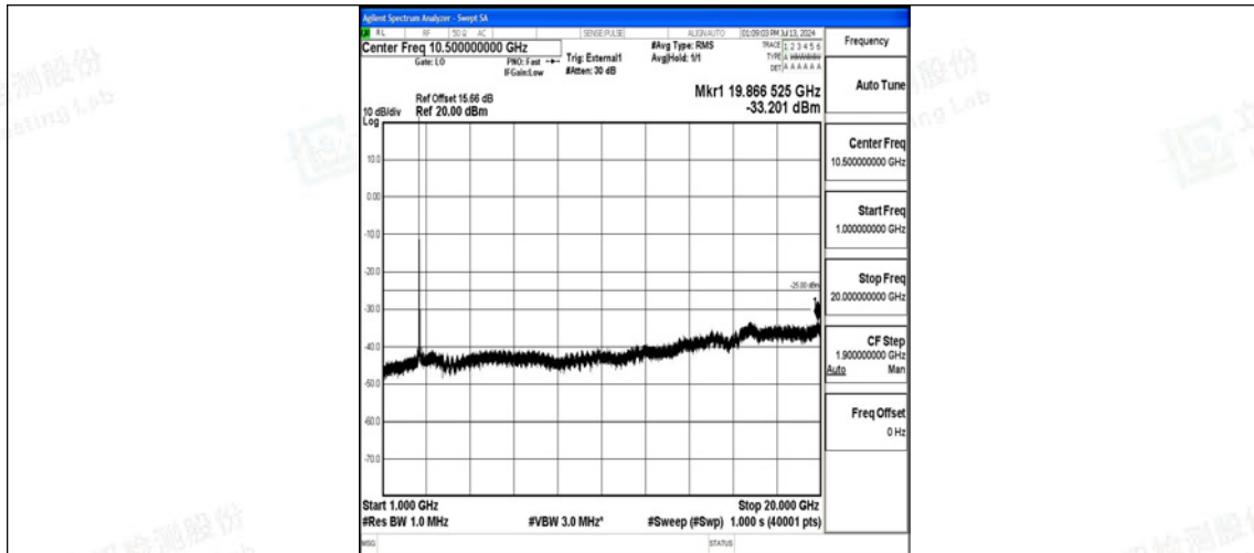
Band41_20MHz_16QAM_40620_1RB#0_1000~20000_1000~20000
