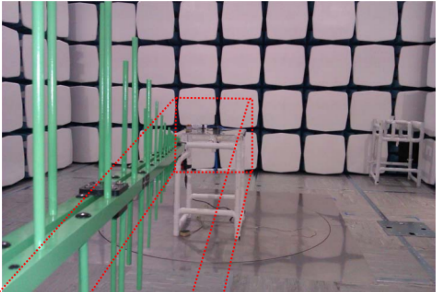
Test Setup
