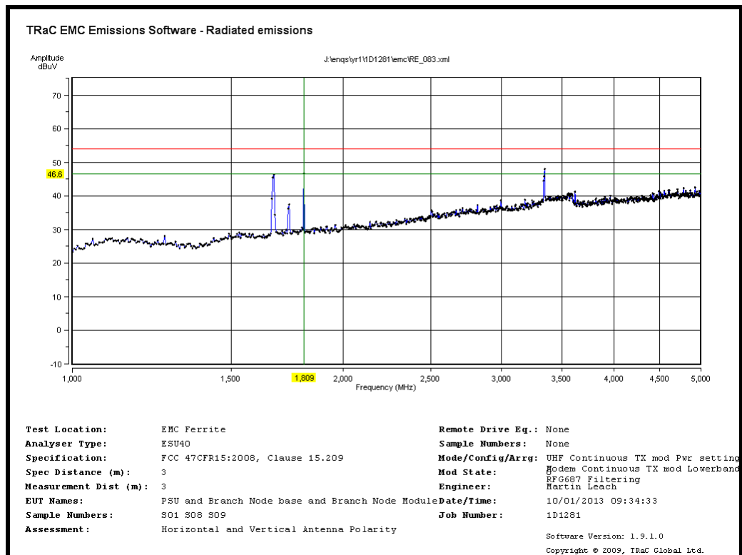
Radiated Transmitter Emissions: UHF Radio Transmit Channel 0 905.2MHz and Modem Transmit Lower Band-Mid CH4183 (RFG687 Filtering)
