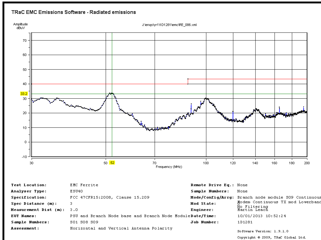
Radiated Transmitter Emissions Modem only Transmit Lower Band-Mid CH4183 (No Filtering)
