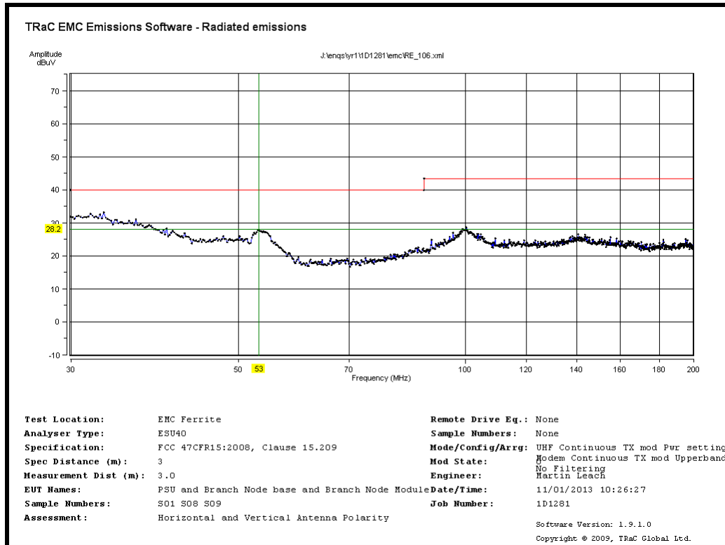
Radiated Transmitter Emissions: UHF Radio Transmit Channel 31 910.47MHz and Modem Transmit Upper Band-Mid CH9400 (No Filtering)
