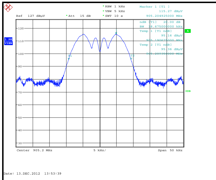
20dB Bandwidth Bottom Channel 905.20MHz
