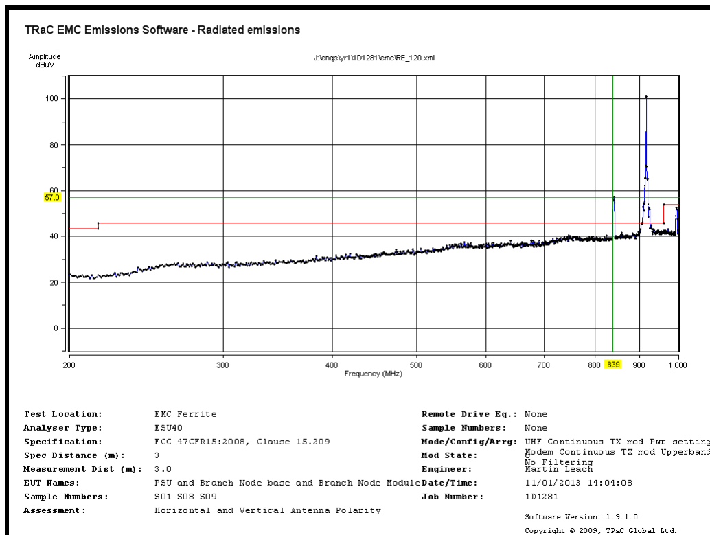
Radiated Transmitter Emissions: UHF Radio Transmit Channel 63 915.19MHz and Modem Transmit Upper Band-Top CH9538 (No Filtering)
