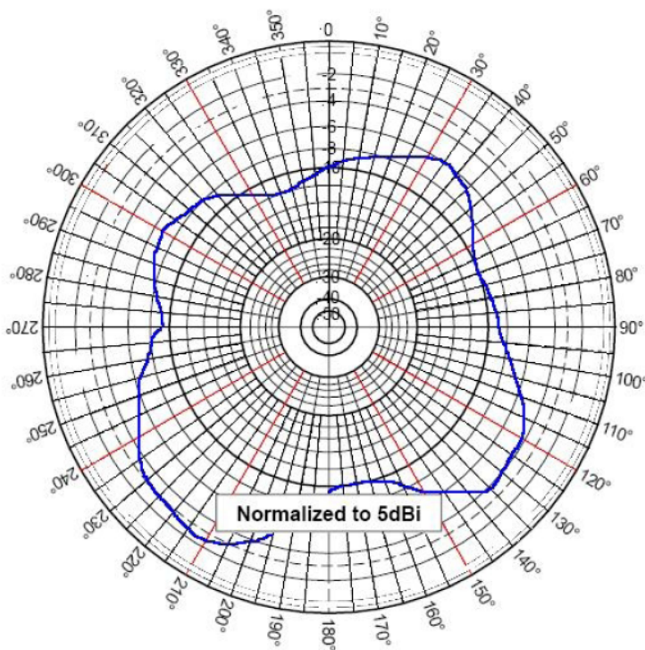
Azimuthal Pattern (X, Y or E-Plane)
