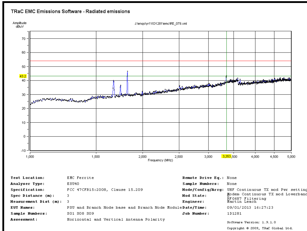
Radiated Transmitter Emissions: UHF Radio Transmit Channel 31 910.47MHz and Modem Transmit Lower Band-Mid CH4183 (RFG687 Filtering)
