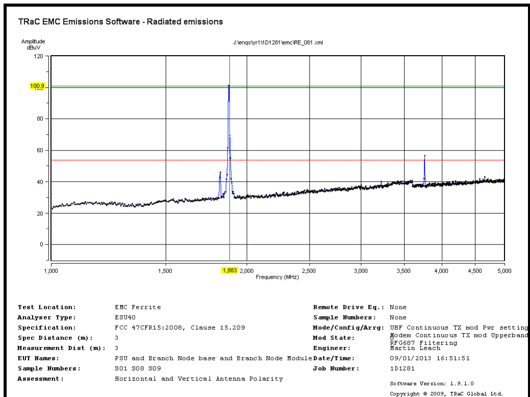
Radiated Transmitter Emissions: UHF Radio Transmit Channel 31 910.47MHz and Modem Transmit Upper Band-Mid CH9400 (RFG687 Filtering)
