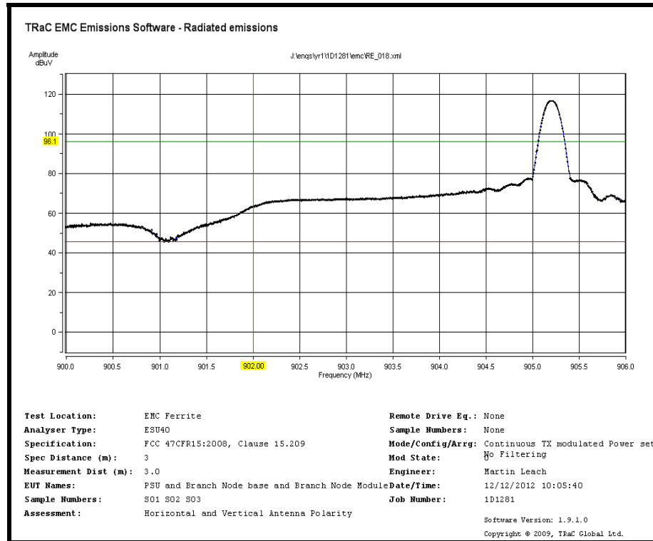
Radiated Transmitter Emissions UHF Radio only Channel 0 905.2MHz (15.209) Lower Band Edge Compliance RBW 100kHz
