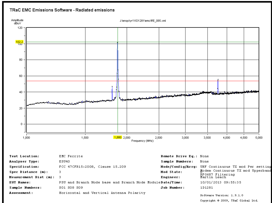
Radiated Transmitter Emissions: UHF Radio Transmit Channel 0 905.2MHz and Modem Transmit Upper Band-Mid CH9400 (RFG687 Filtering)
