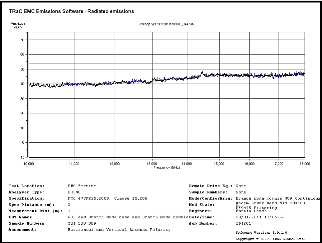
Radiated Transmitter Emissions Modem only Transmit Lower Band-Mid CH4183 (RFG445 Filtering)
