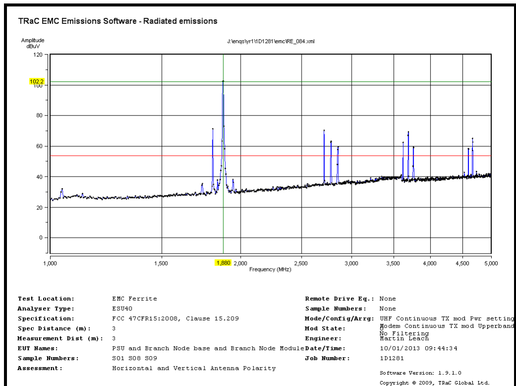
Radiated Transmitter Emissions: UHF Radio Transmit Channel 0 905.2MHz and Modem Transmit Upper Band-Mid CH9400 (No Filtering)
