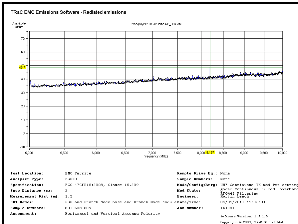
Radiated Transmitter Emissions: UHF Radio Transmit Channel 31 910.47MHz and Modem Transmit Lower Band-Mid CH4183 (RFG445 Filtering)
