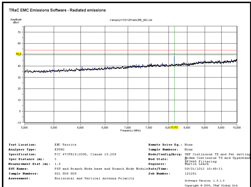
Radiated Transmitter Emissions: UHF Radio Transmit Channel 0 905.2MHz and Modem Transmit Upper Band-Mid CH9400 (RFG445 Filtering)
