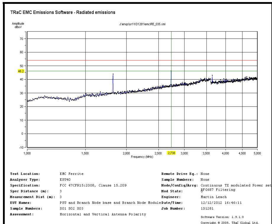
Radiated Transmitter Emissions UHF Radio only Channel 31 910.47MHz (15.209)
