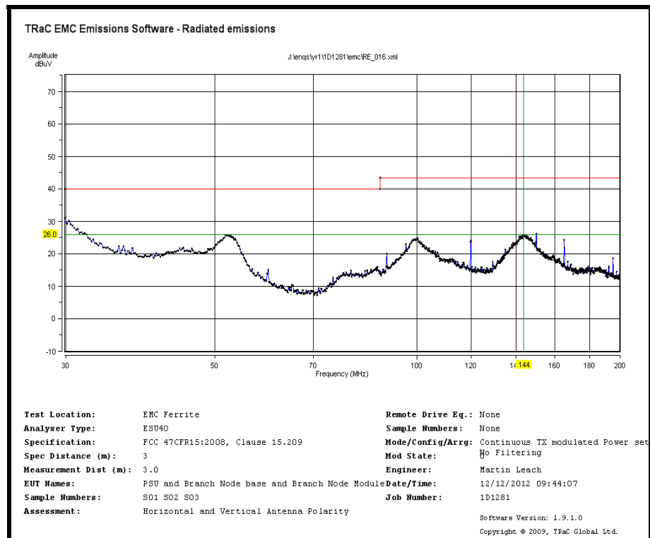
Radiated Transmitter Emissions UHF Radio only Channel 0 905.2MHz (15.209)
