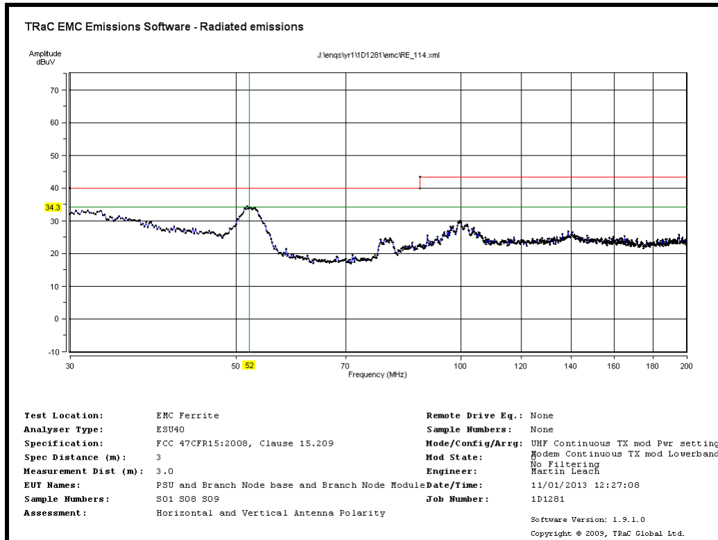
Radiated Transmitter Emissions: UHF Radio Transmit Channel 63 915.19MHz and Modem Transmit Lower Band-Mid CH4183 (No Filtering)
