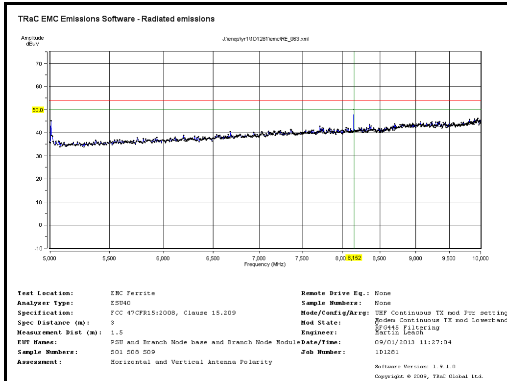
Radiated Transmitter Emissions: UHF Radio Transmit Channel 0 905.2MHz and Modem Transmit Lower Band-Mid CH4183 (RFG445 Filtering)
