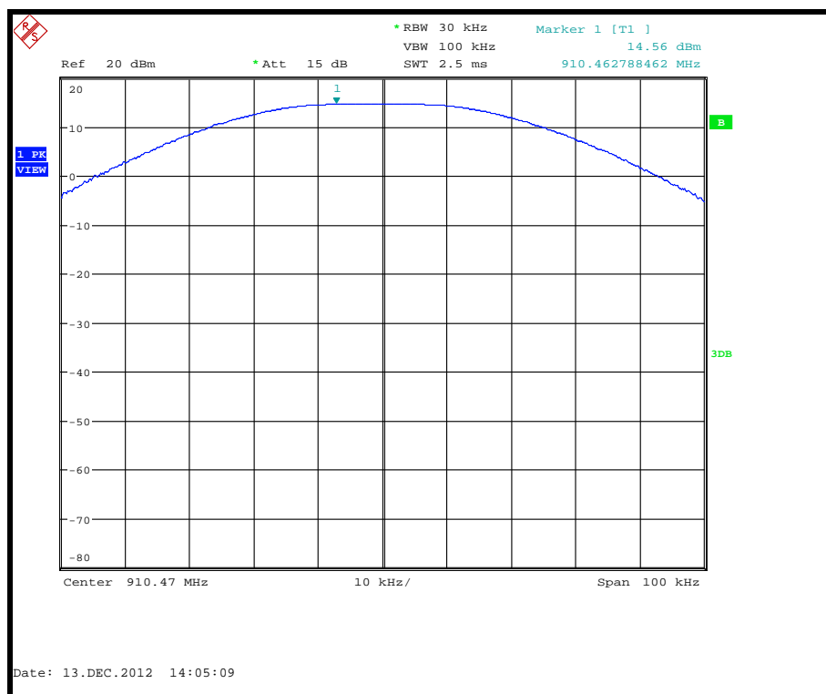
Conducted Carrier Power Middle: Channel 31 910.47MHz
