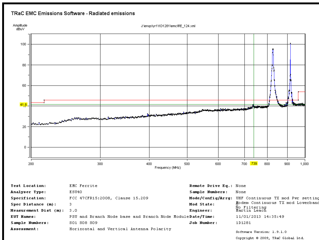
Radiated Transmitter Emissions: UHF Radio Transmit Channel 63 915.19MHz and Modem Transmit Lower Band-Bottom CH4132 (No Filtering)
