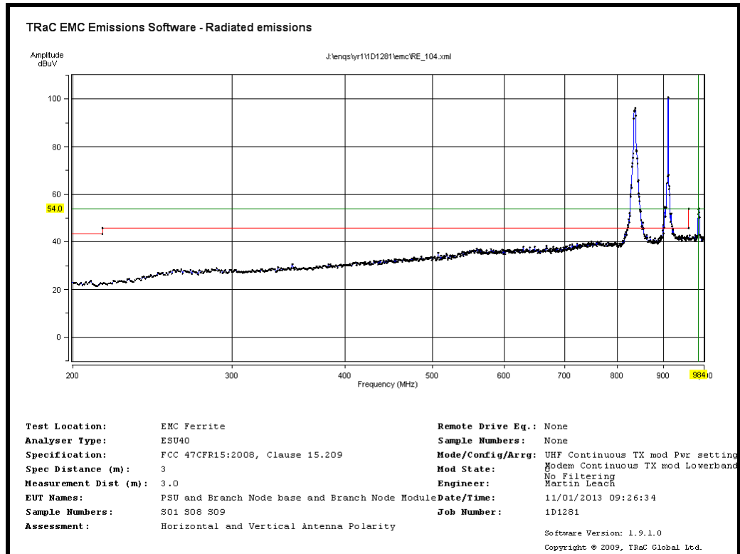
Radiated Transmitter Emissions: UHF Radio Transmit Channel 31 910.47MHz and Modem Transmit Lower Band-Mid CH4183 (No Filtering)
