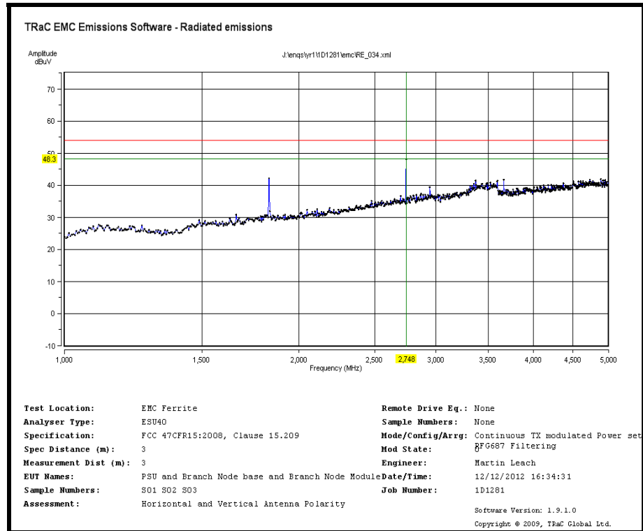
Radiated Transmitter Emissions UHF Radio only Channel 63 915.19MHz (15.209)
