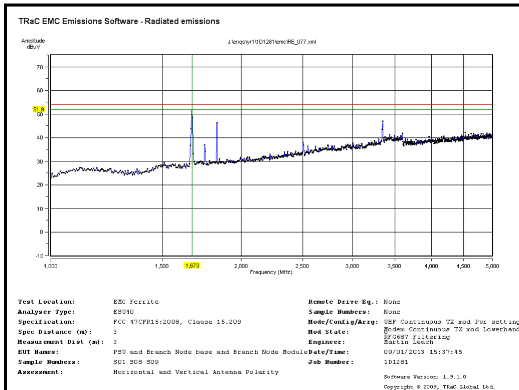
Radiated Transmitter Emissions: UHF Radio Transmit Channel 63 915.19MHz and Modem Transmit Lower Band-Mid CH4183 (RFG687 Filtering)
