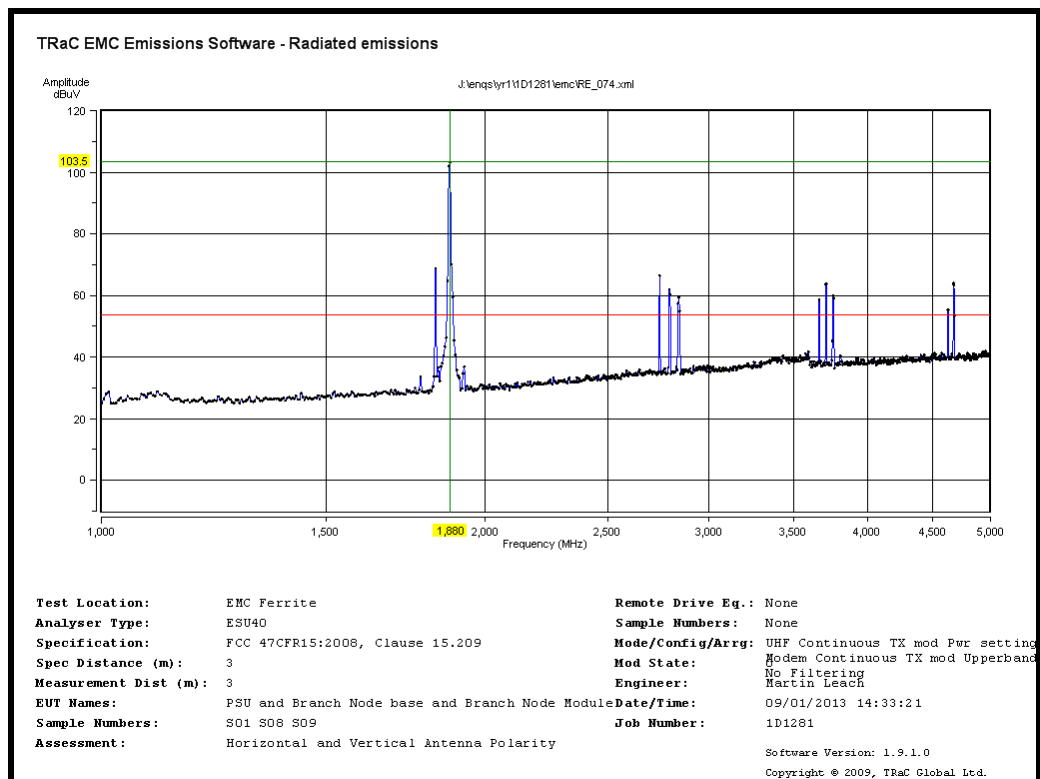
Radiated Transmitter Emissions: UHF Radio Transmit Channel 63 915.19MHz and Modem Transmit Upper Band-Mid CH9400 (No Filtering)
