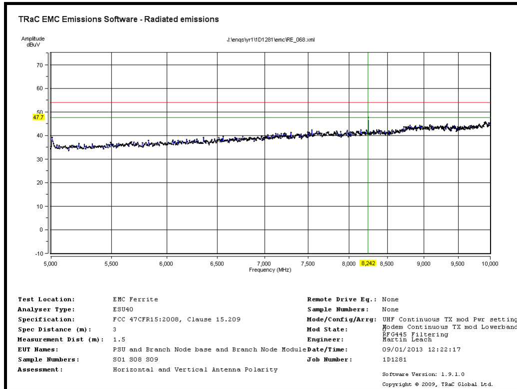
Radiated Transmitter Emissions: UHF Radio Transmit Channel 63 915.19MHz and Modem Transmit Lower Band-Mid CH4183 (RFG445 Filtering)
