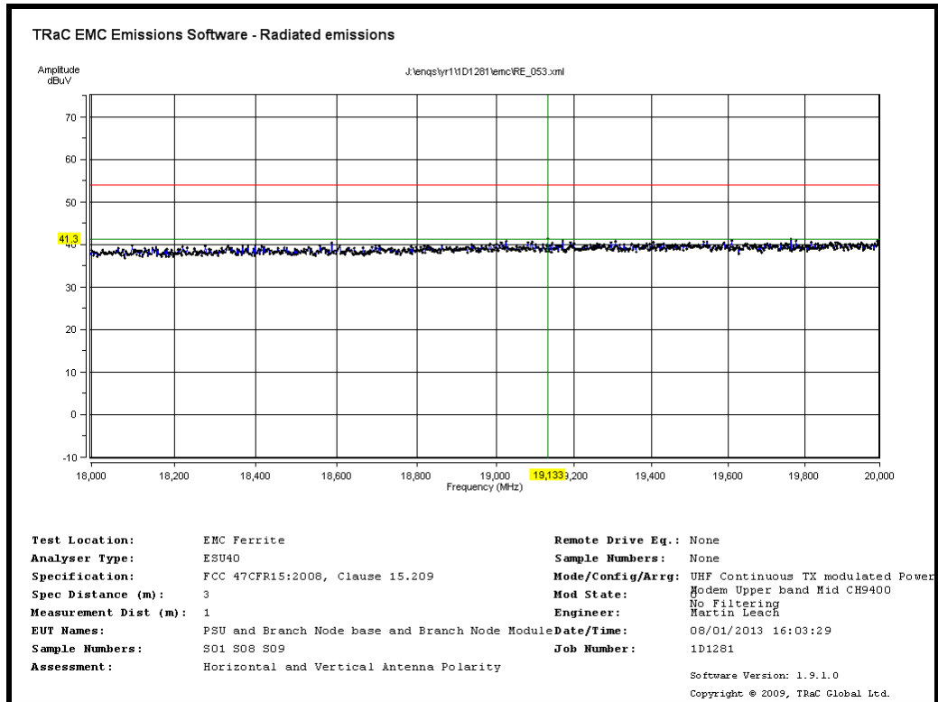
Radiated Transmitter Emissions: UHF Radio Transmitter Channel 31 910.47MHz and Modem Transmit Upper Band-Mid CH9400 (No Filtering)
