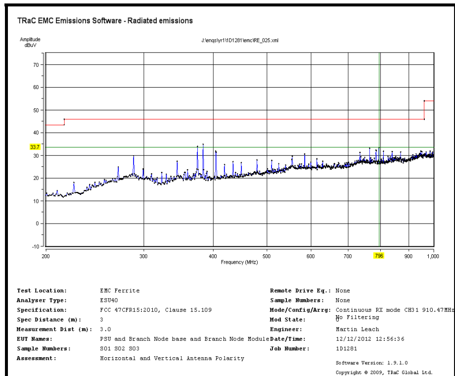
Radiated RX Mode Emissions (15.109)
