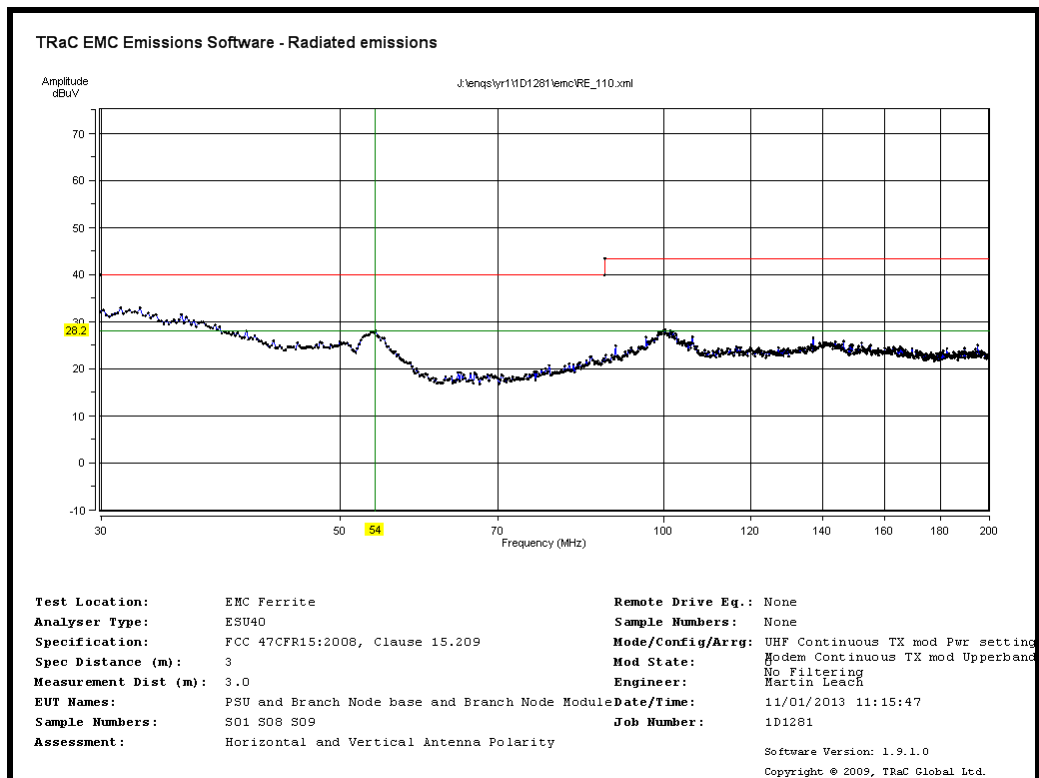
Radiated Transmitter Emissions: UHF Radio Transmitter Channel 63 915.19MHz and Modem Transmit Upper Band-Mid CH9400 (No Filtering)
