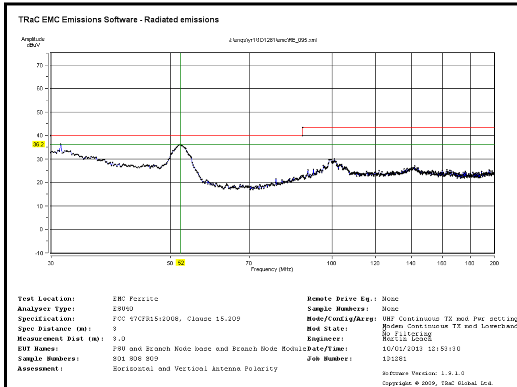
Radiated Transmitter Emissions: UHF Radio Transmit Channel 0 905.2MHz and Modem Transmit Lower Band-Mid CH4183 (No Filtering)
