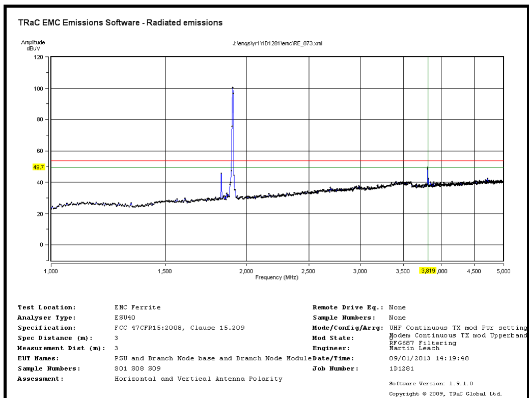
Radiated Transmitter Emissions: UHF Radio Transmit Channel 63 915.19MHz and Modem Transmit Upper Band-Top CH9538 (RFG687 Filtering)
