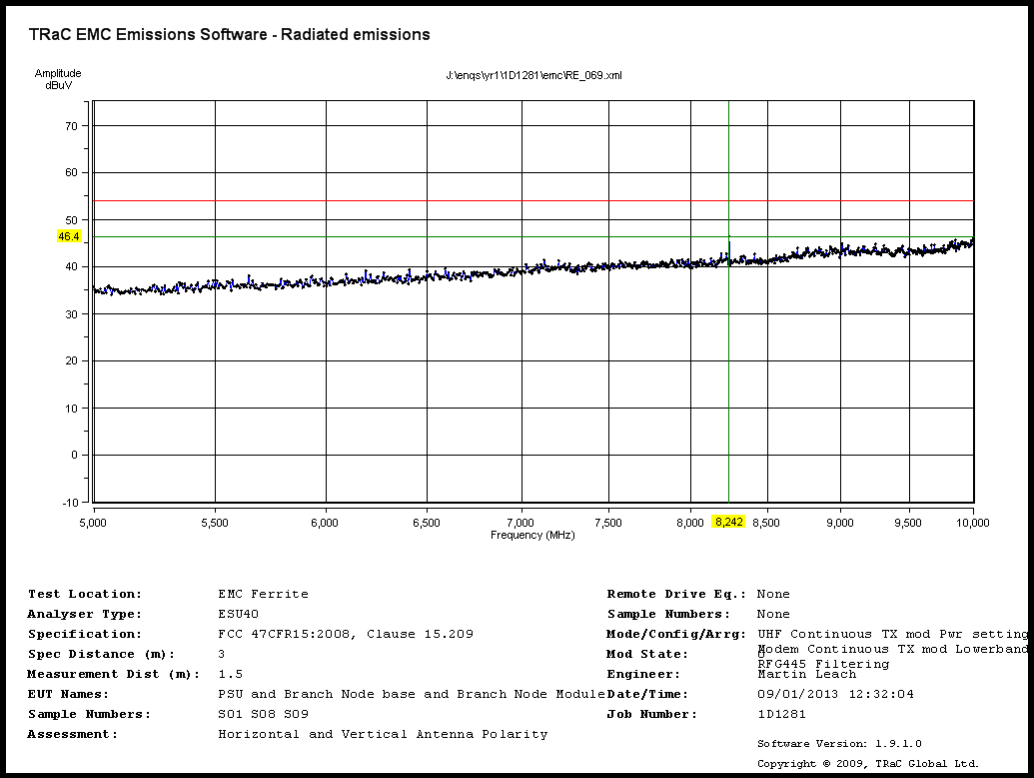
Radiated Transmitter Emissions: UHF Radio Transmit Channel 63 915.19MHz and Modem Transmit Lower Band-Bottom CH4132 (RFG445 Filtering)
