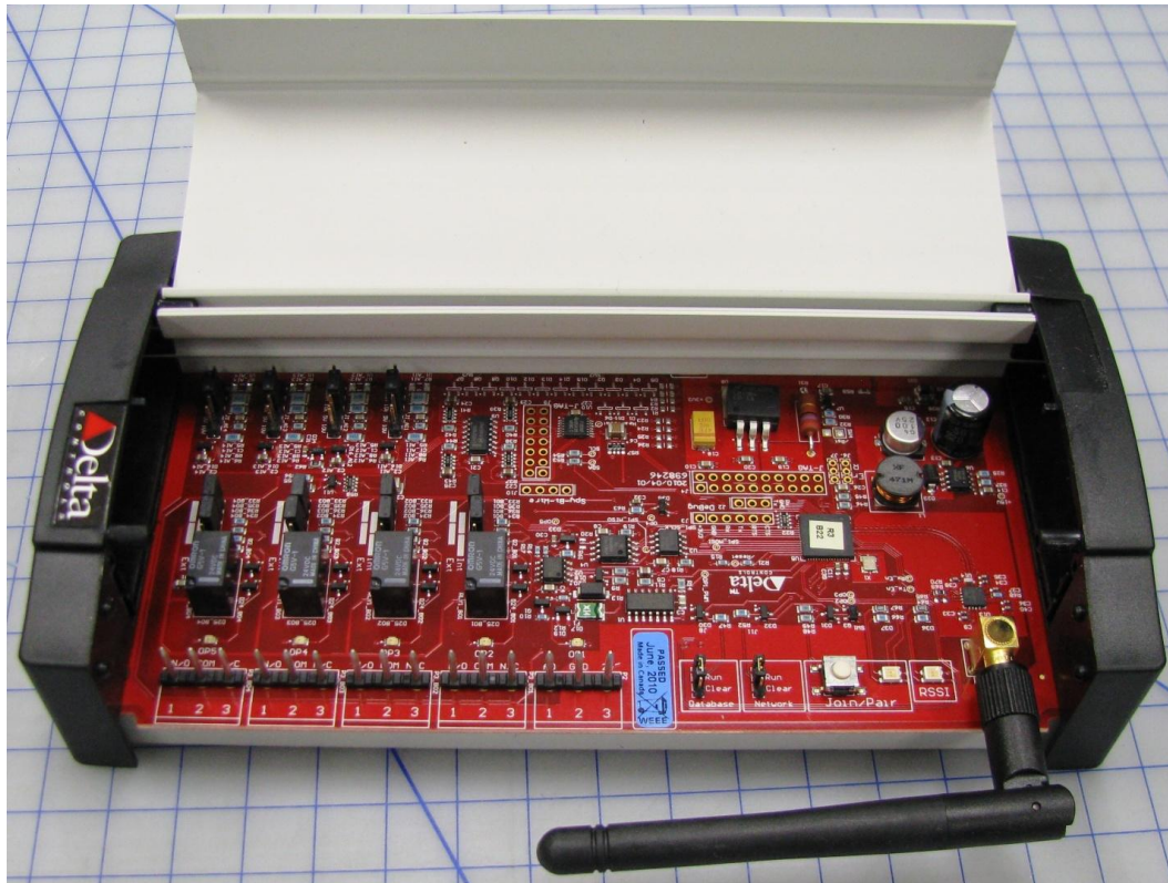
Figure 5: Opened View
