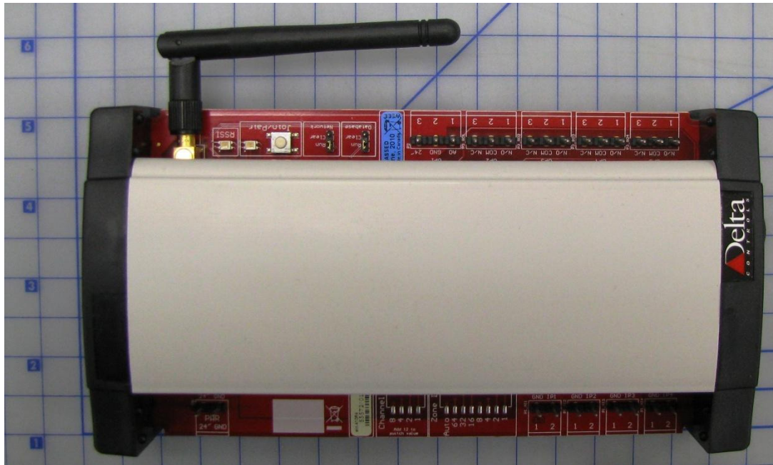
Figure 1: Top View
