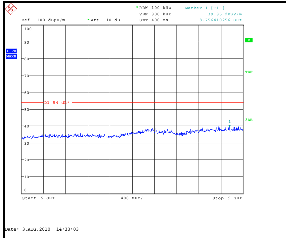
Radiated spurious emissions 5 GHz to 9 GHz
