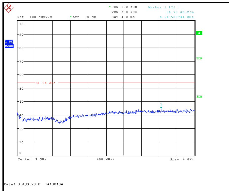
Radiated spurious emissions 1 GHz to 5 GHz
