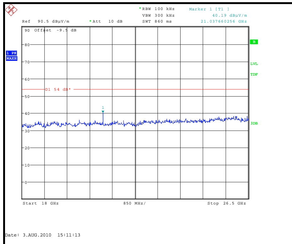
Radiated spurious emissions 18 GHz to 26.5GHz
