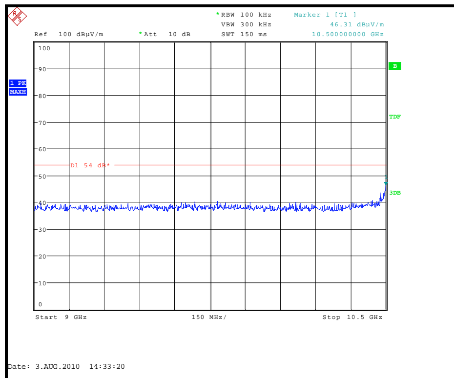
Radiated spurious emissions 9 GHz to 10.500 GHz
