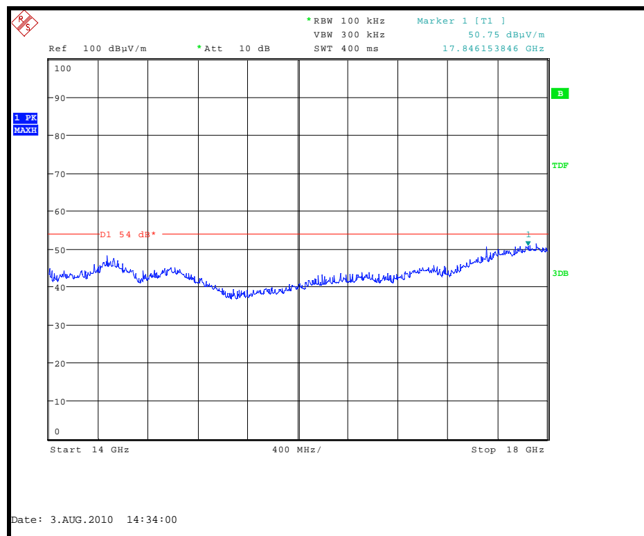
Radiated spurious emissions 14 GHz to 18 GHz
