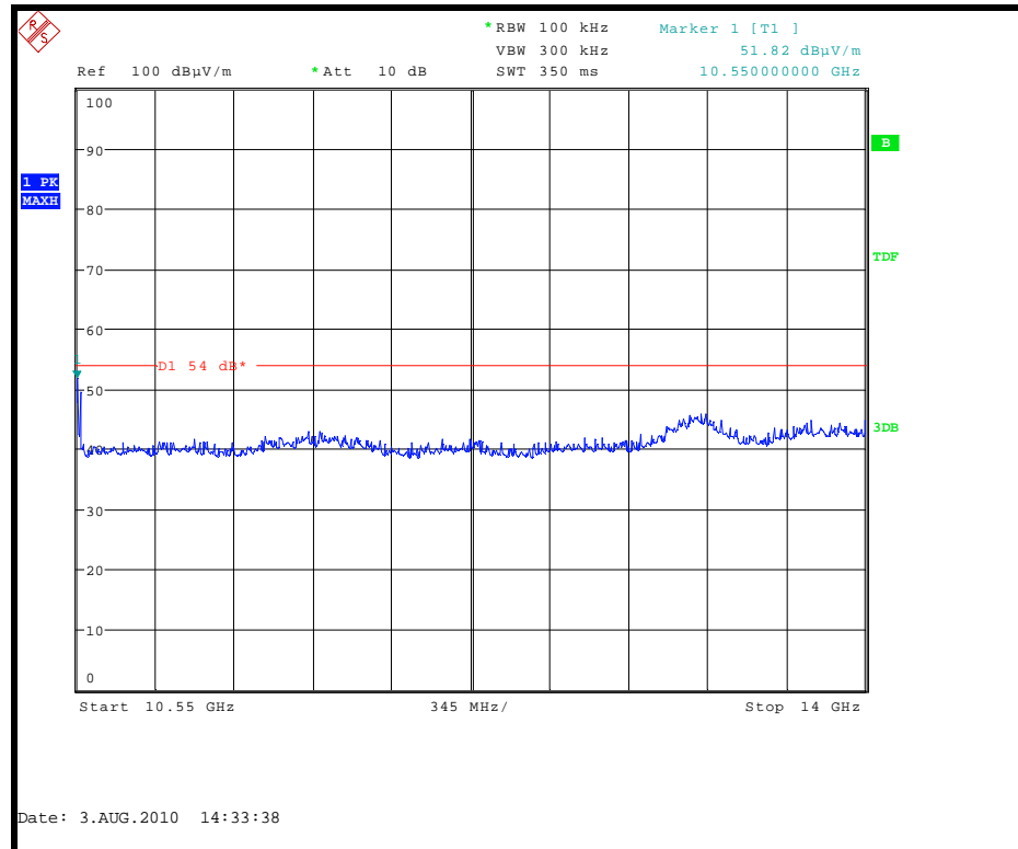
Radiated spurious emissions 10.550 GHz to 14 GHz
