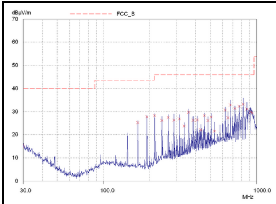
Radiated spurious emissions 30 MHz to 1 GHz
