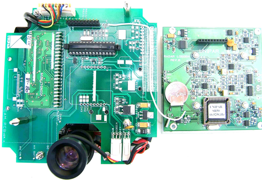
TOP VIEW OF SENTINEL WITH RADAR PCB REMOVED
