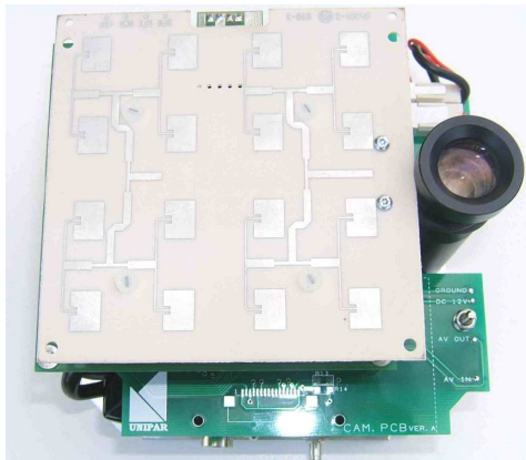
TOP VIEW OF SENTINEL COMPLETE AND OUT OF ITS HOUSING.
