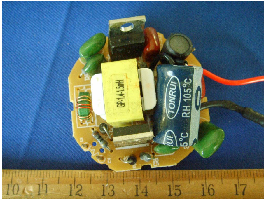
EUT –Components View (GU242627)
