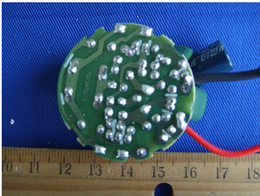
EUT–Solder View (G261527)
