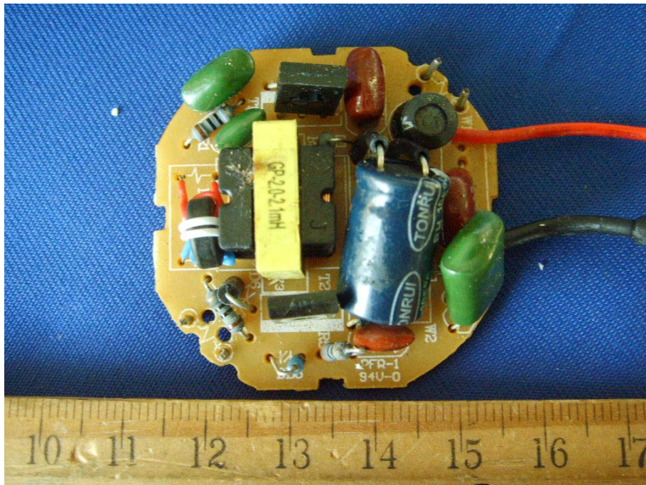
EUT –Components View (GU241327)
