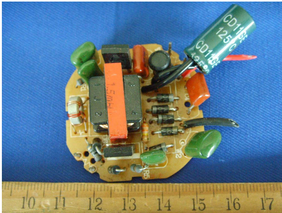
EUT –Components View (G262327)
