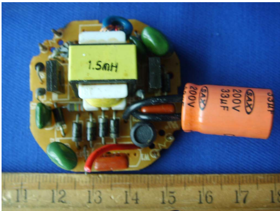
EUT –Components View (G262627)
