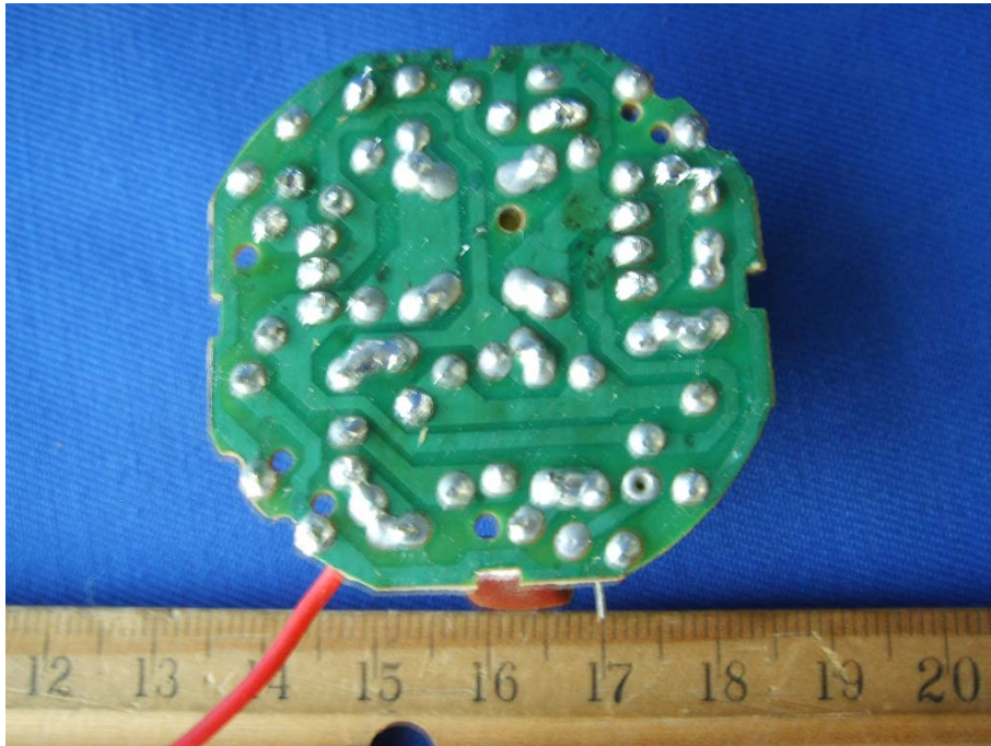
EUT-Solder View (G261827)
