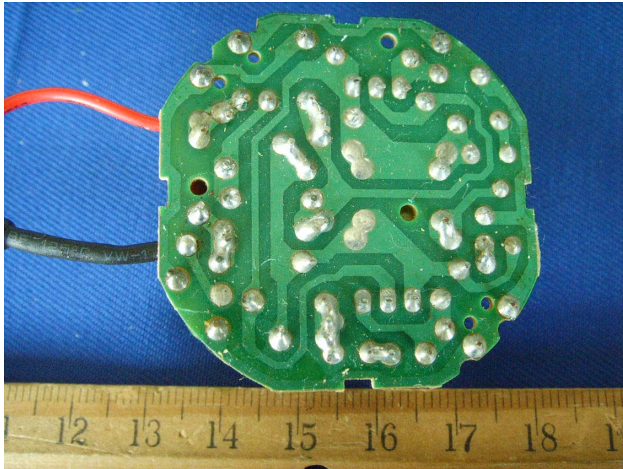
EUT-Solder View (G242627)
