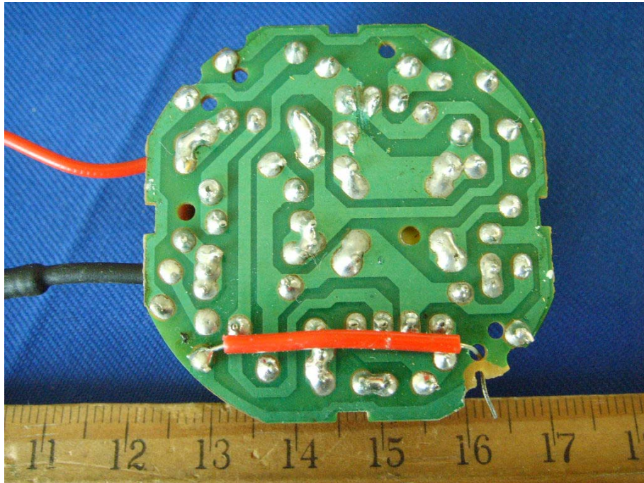
EUT-Solder View (G241827)
