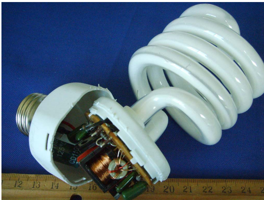
EUT – Uncovered View (G262327)
