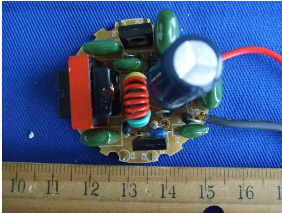
EUT –Components View (G261527)
