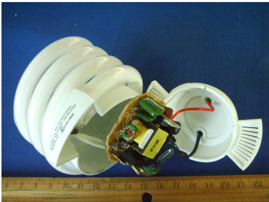
EUT – Uncovered View (GU242627)
