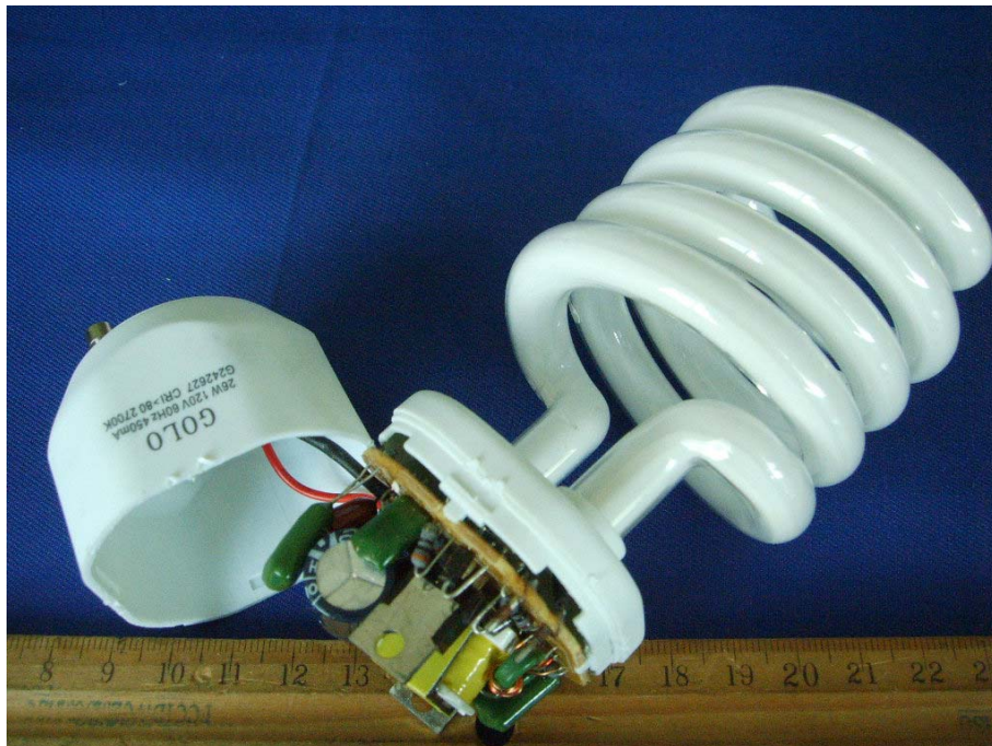
EUT – Uncovered View (G242627)
