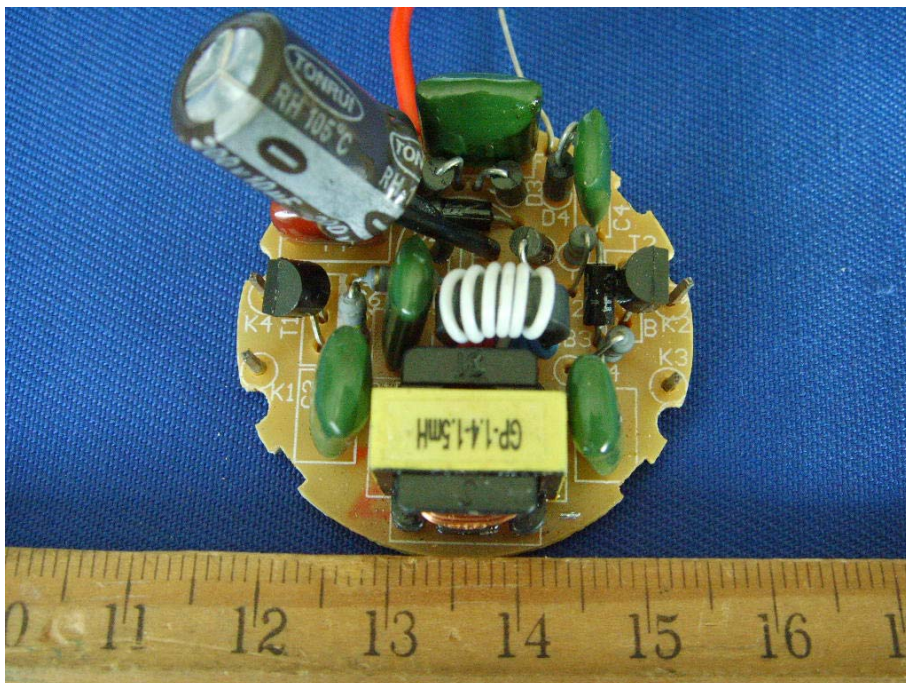
EUT –Components View (G261327)
