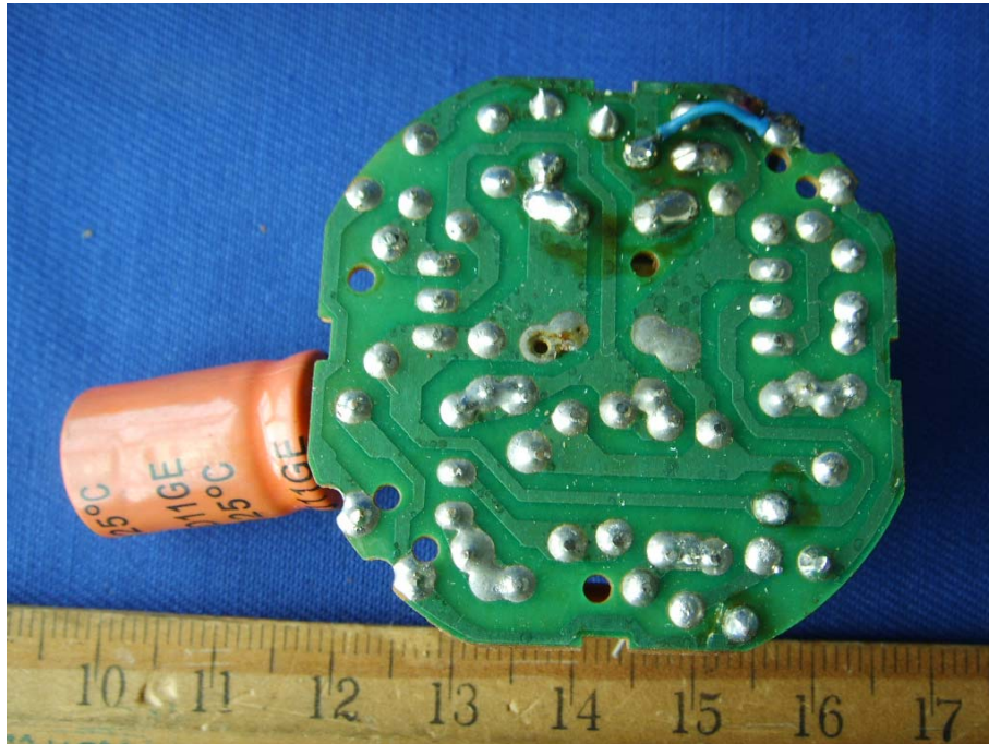
EUT-Solder View (G262627)
