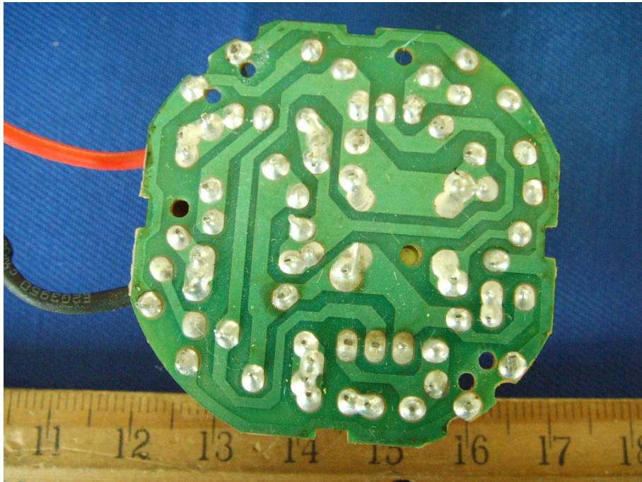
EUT-Solder View (GU241827)
