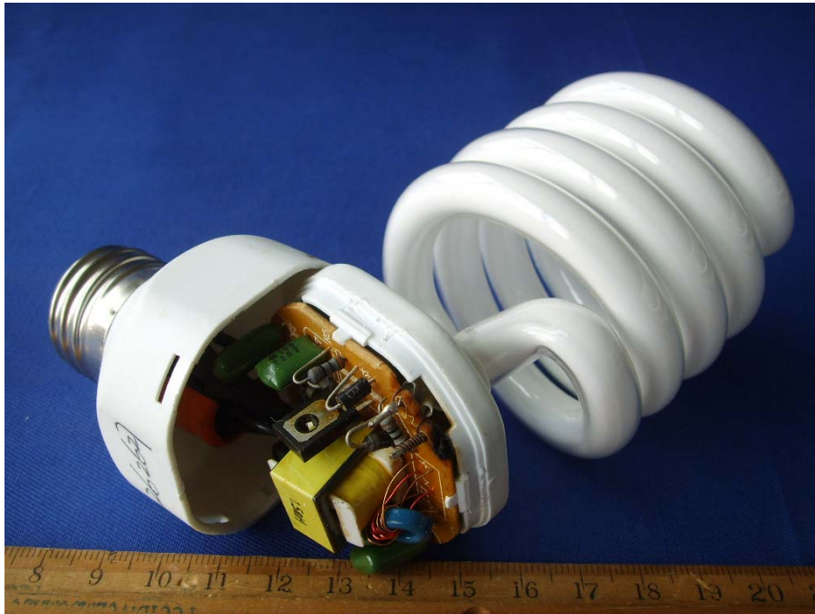
EUT – Uncovered View (G262627)
