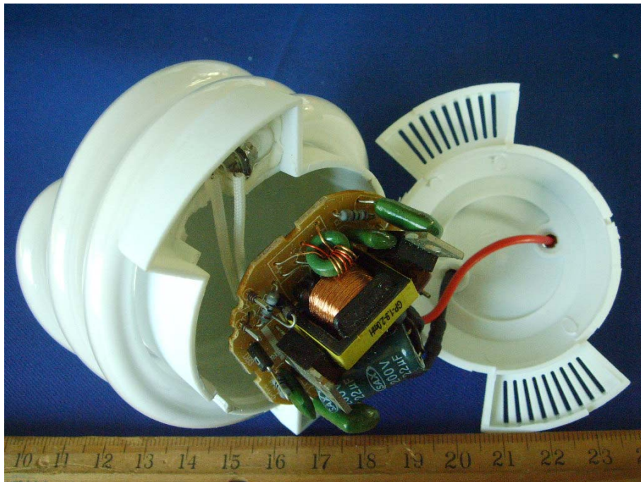
EUT – Uncovered View (GU241827)
