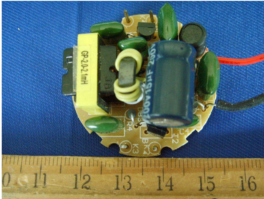
EUT –Components View (G241327)
