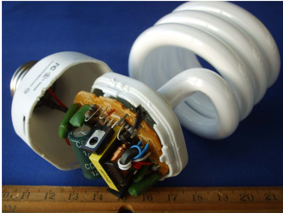
EUT – Uncovered View (G261827)
