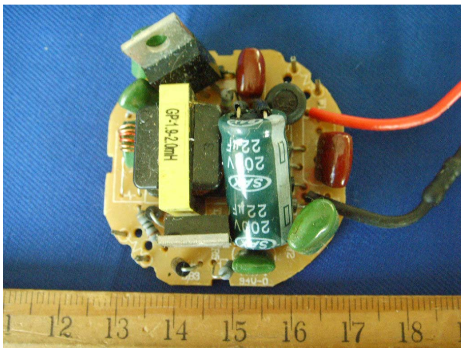
EUT –Components View (GU241827)
