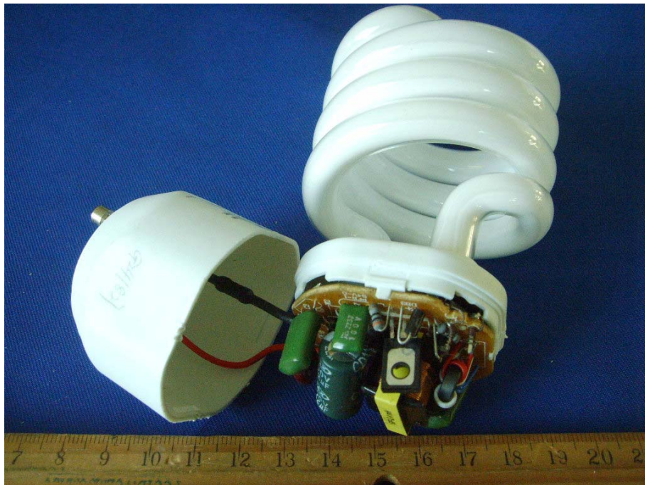
EUT – Uncovered View (G241827)
