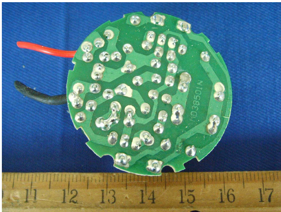
EUT–Solder View (G241327)
