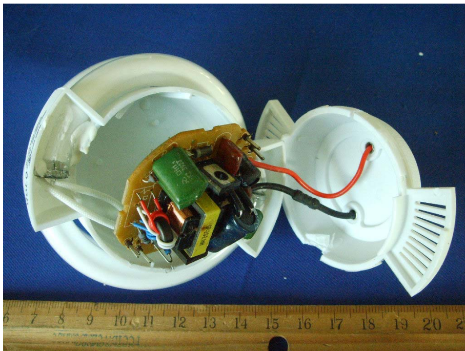
EUT – Uncovered View (GU241327)
