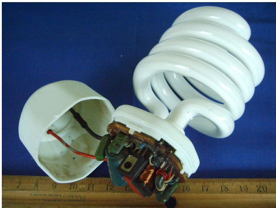
EUT – Uncovered View (G242327)
