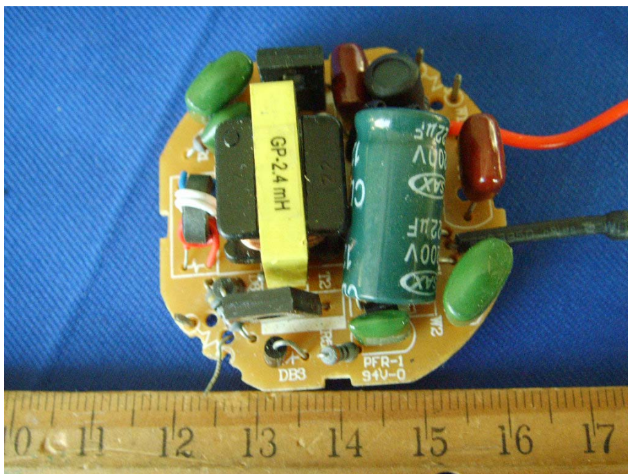
EUT –Components View (G241827)
