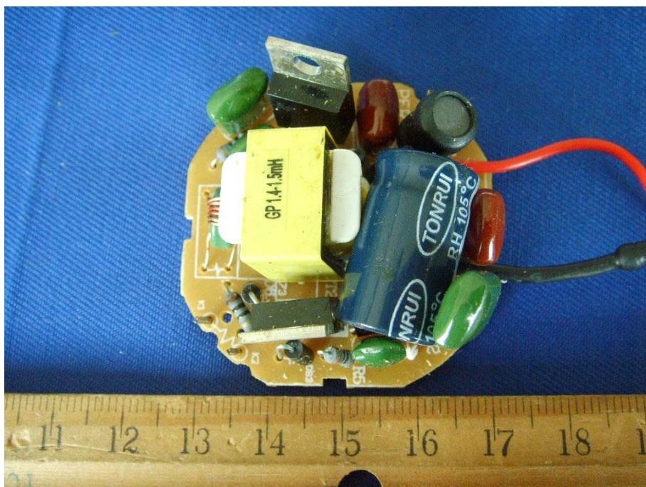
EUT –Components View (G242627)
