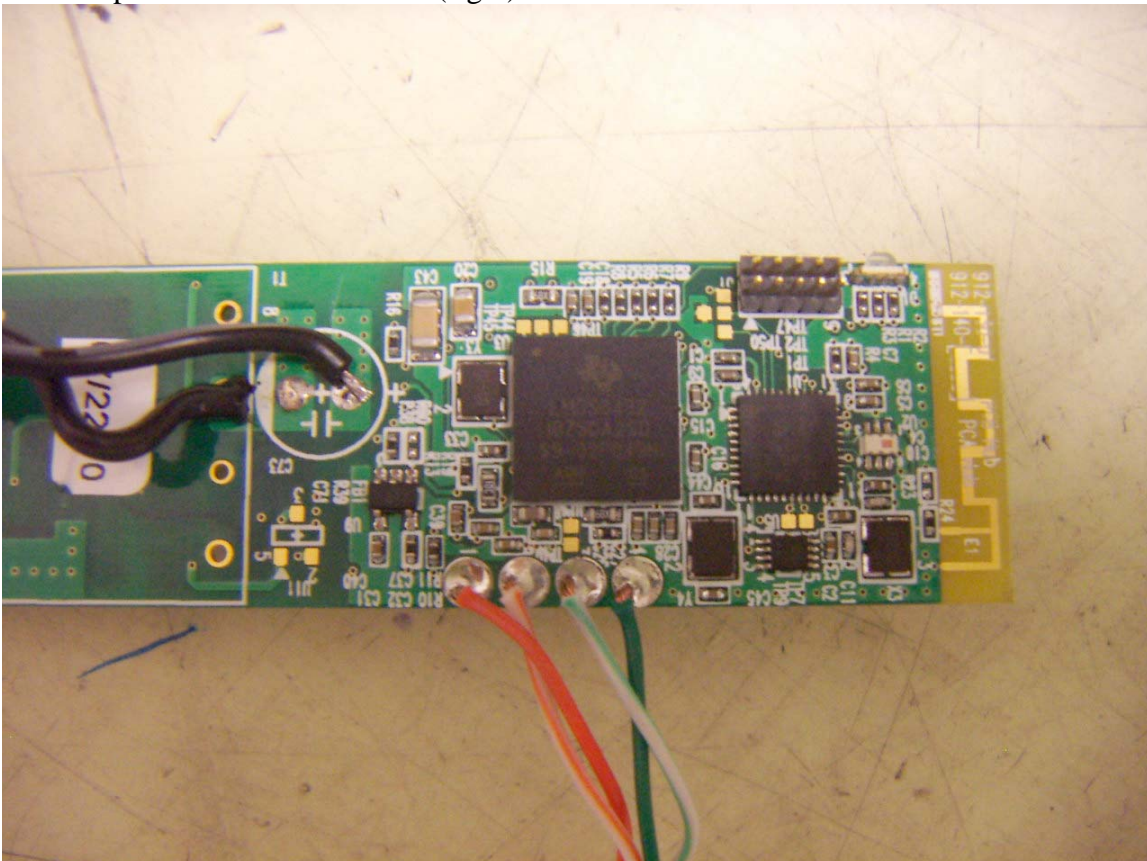
Detail top PCB and PCB antenna (right)
