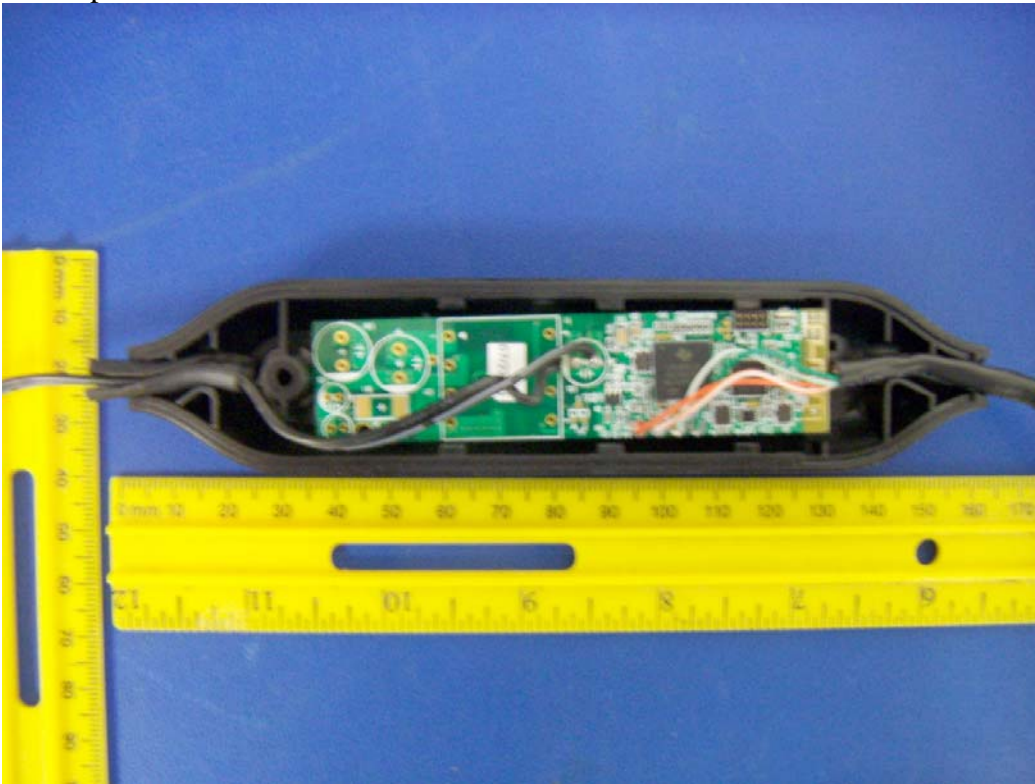
Detail top PCB and PCB antenna (right)
