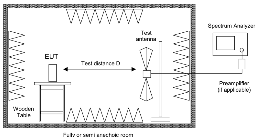
Picture 17: Test setup for radiated emission measurement (> 1 GHz)
