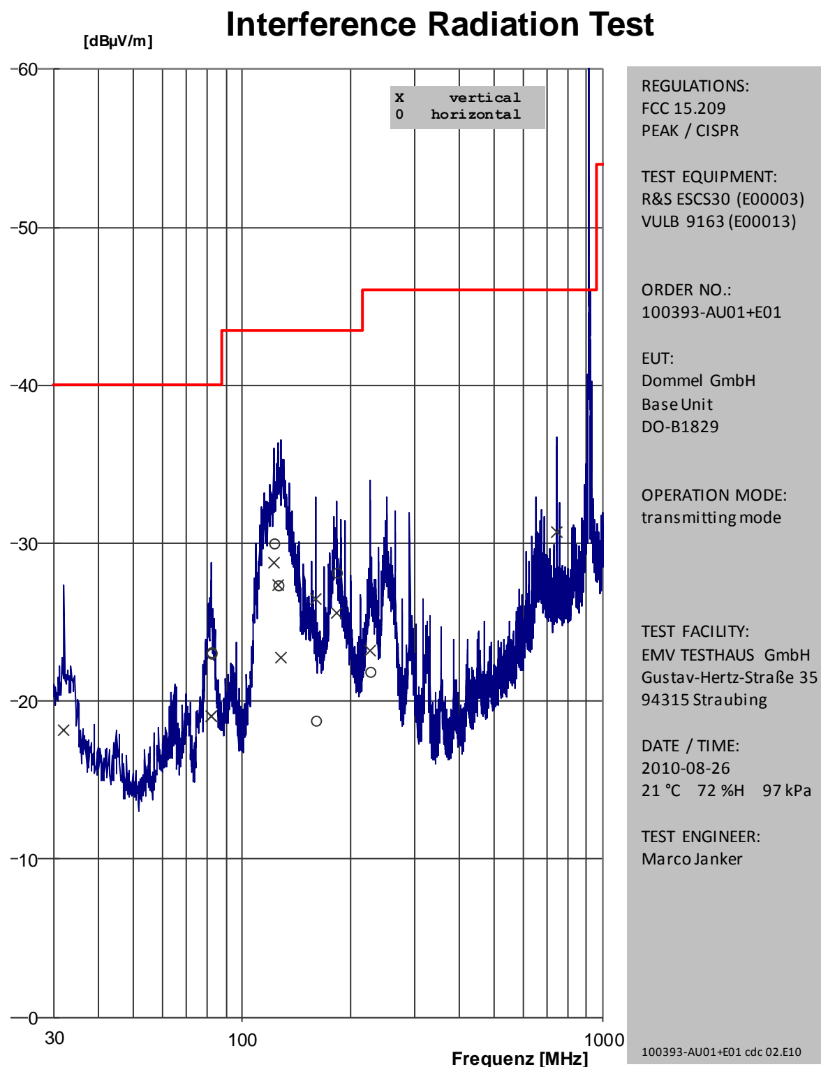
Picture 13: Radiated emission 30 MHz – 1000MHz (TX mode)
