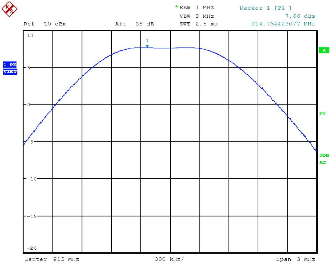
Picture 7: Conducted output power chart
