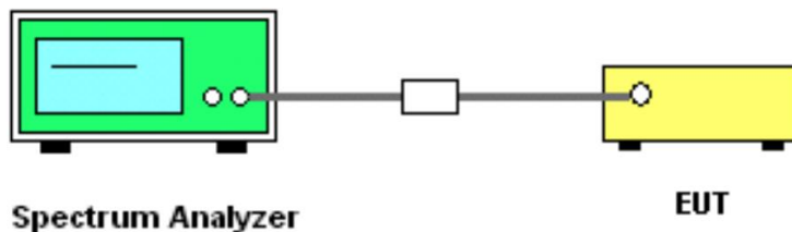
Picture 6: Test setup for conducted output power measurement
