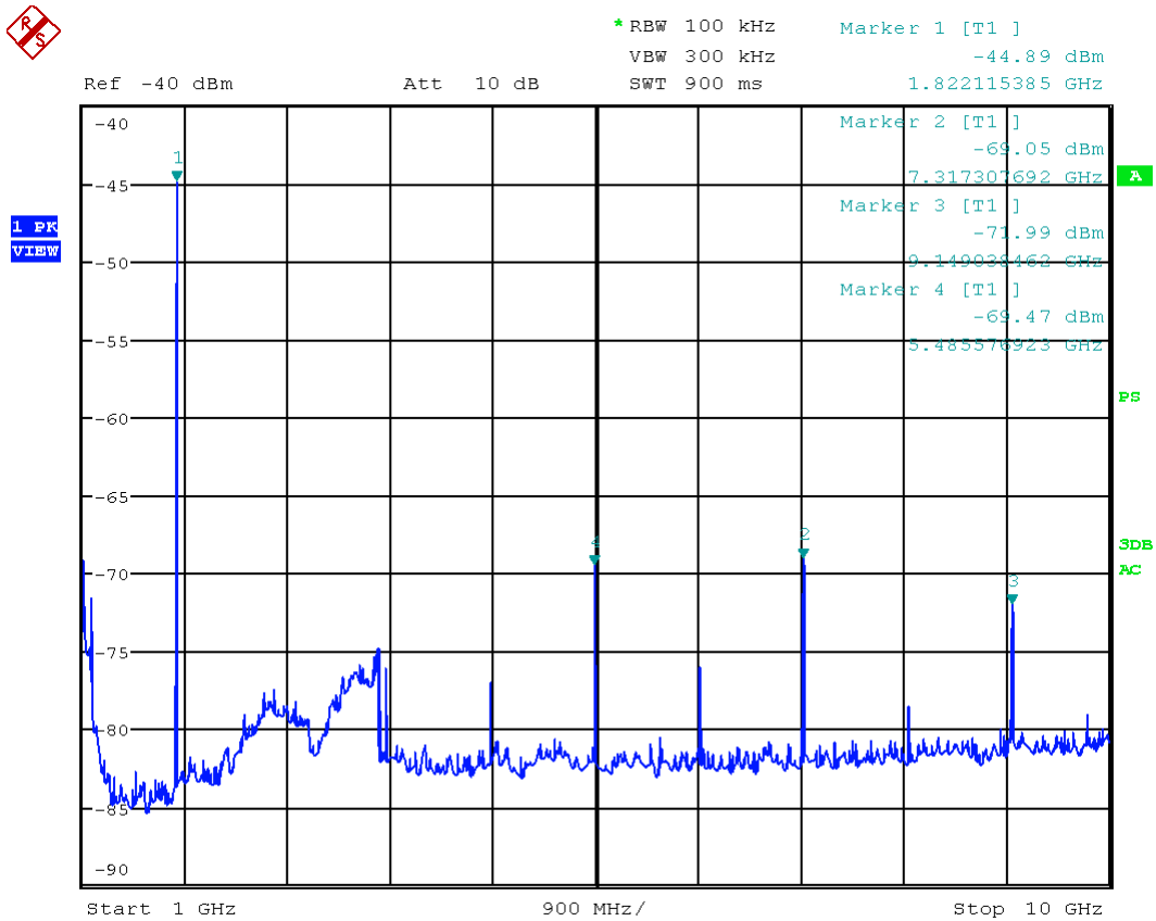
Picture 18: Radiated emission > 1 GHz (pre-scan)
