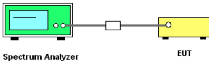
Picture 8: Test setup for power spectral density measurement
