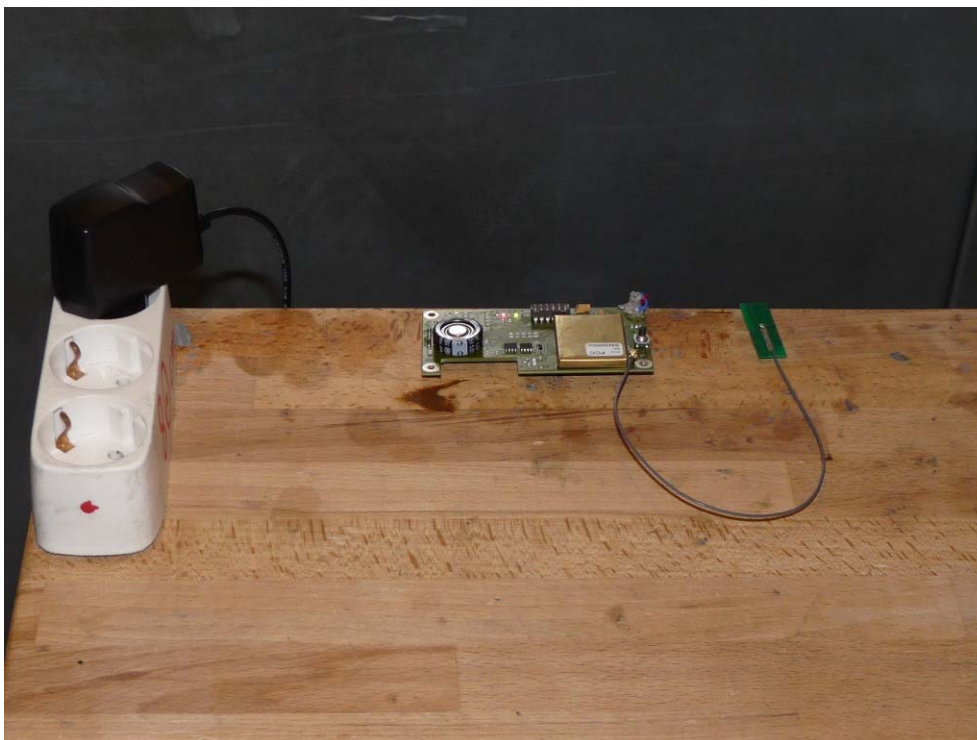
Photo 1: Test setup for conducted emissions (AC mains)
