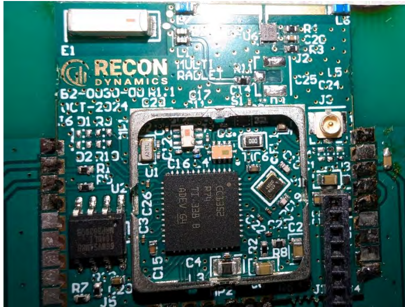
Photograph 59: Close-up View of Front of Module with RF Shield Removed (EUT for All Testing Except Internal 900Mhz Antenna)
