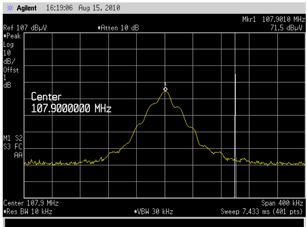
107.9MHZ Test Plot
