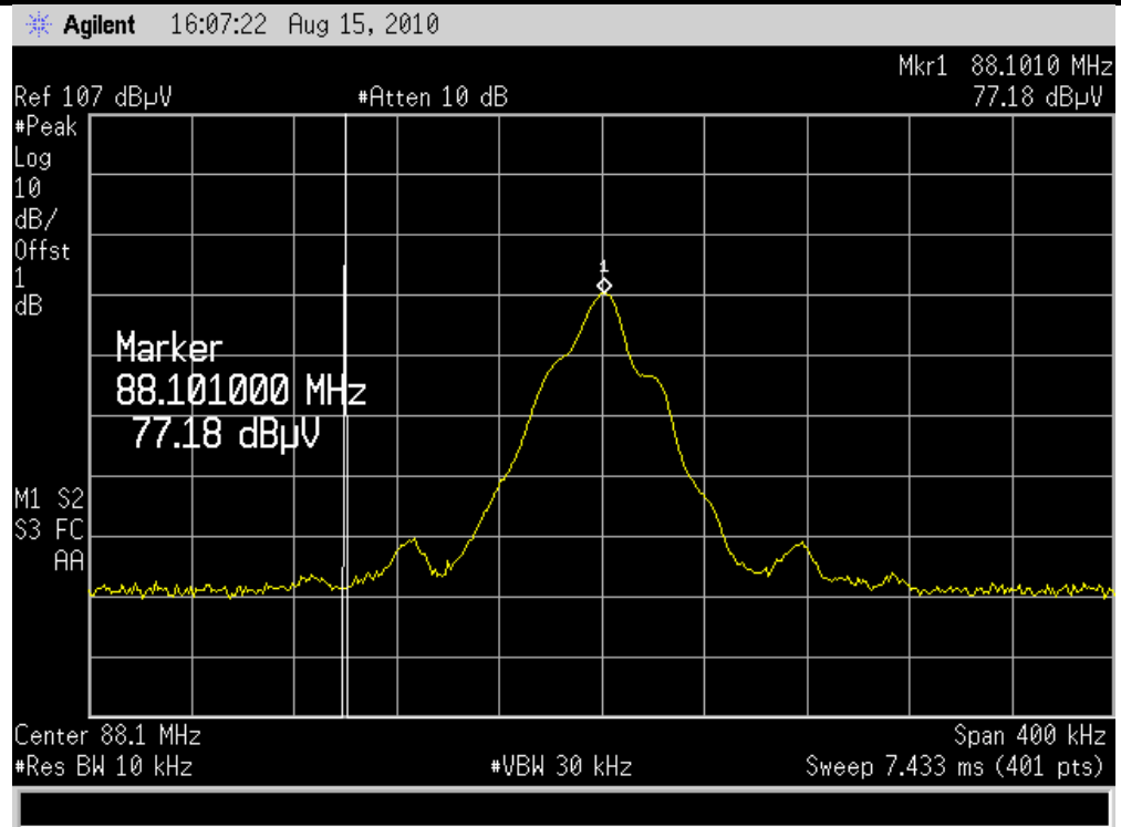
88.1MHZ Test Plot
