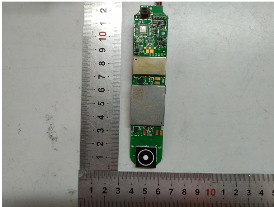
EUT – PCB2 Label View
