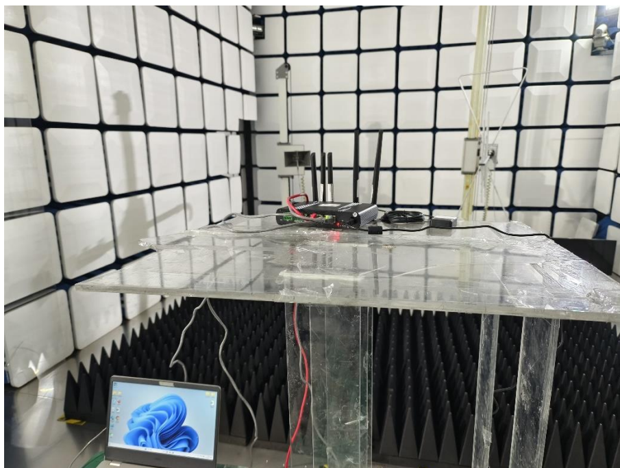
Close-up_SRD
