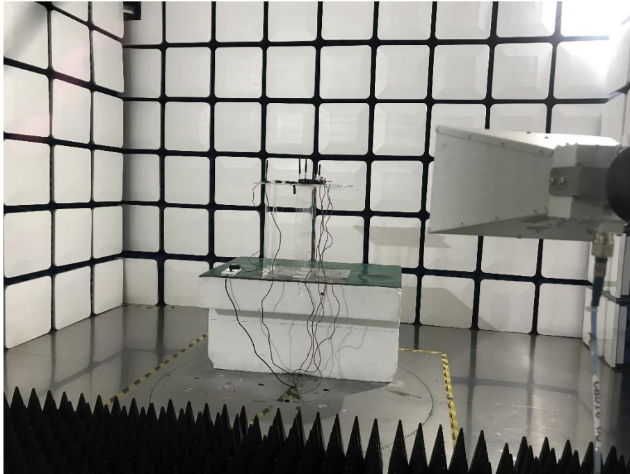
Above 1GHz_WWAN
