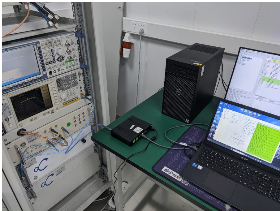
Conducted Test-SRD
