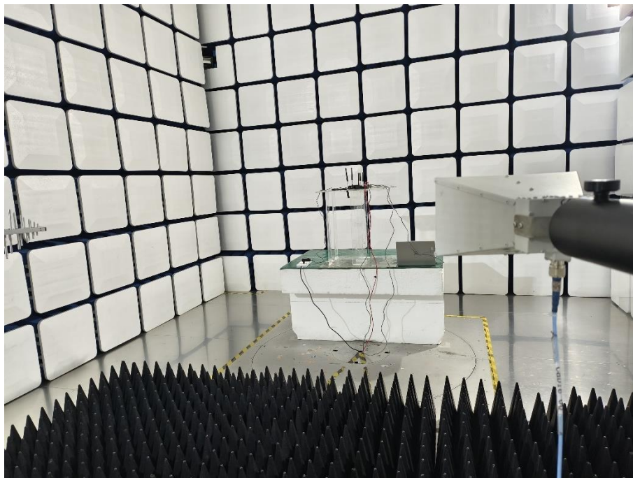
Above 1GHz_SRD
