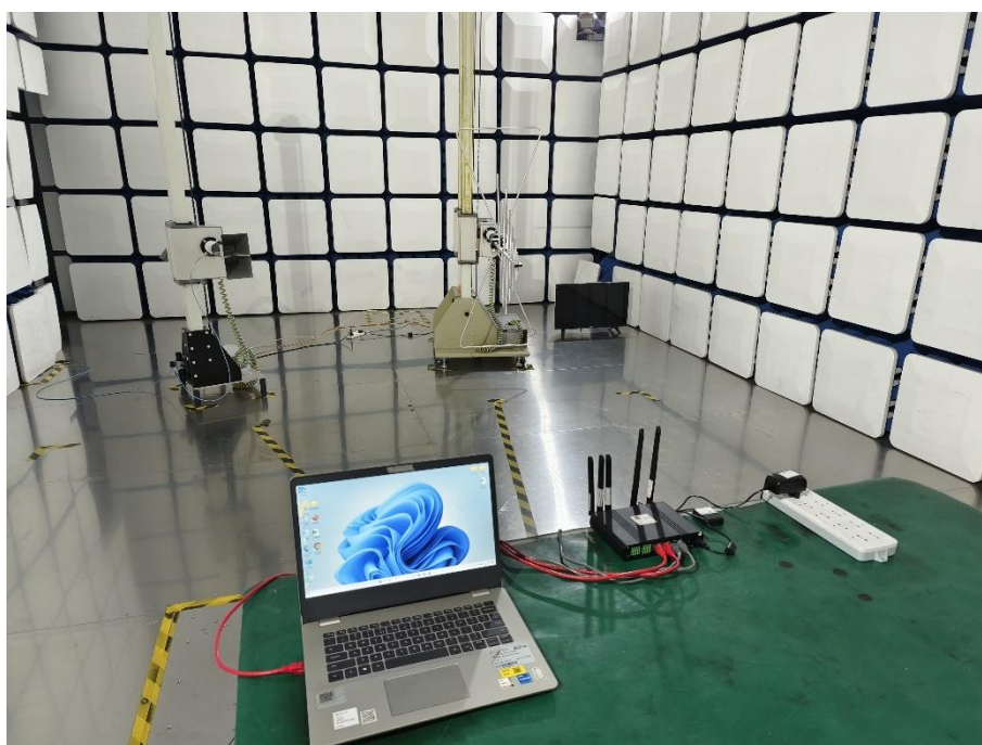
Close-up_SRD
