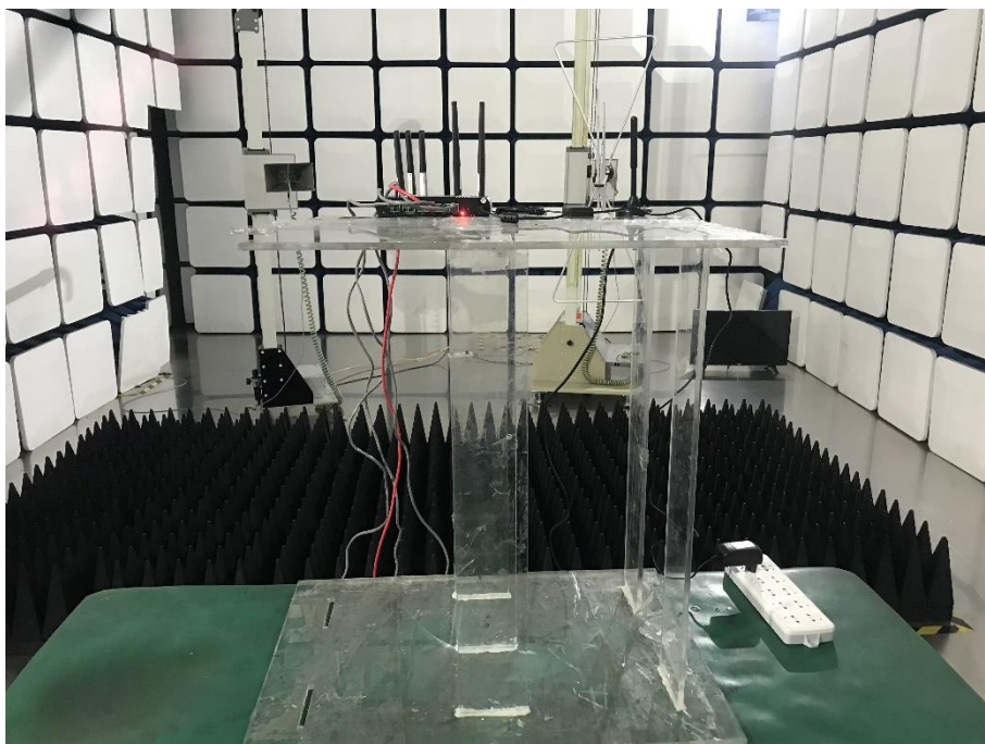
Close-up_WWAN
