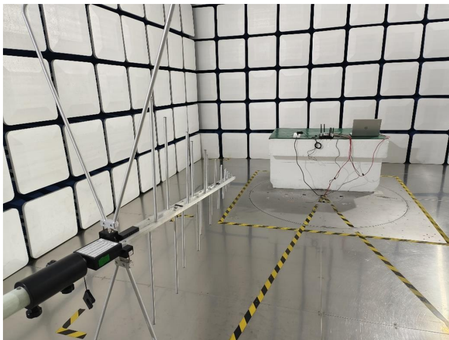
30MHz-1GHz_SRD
