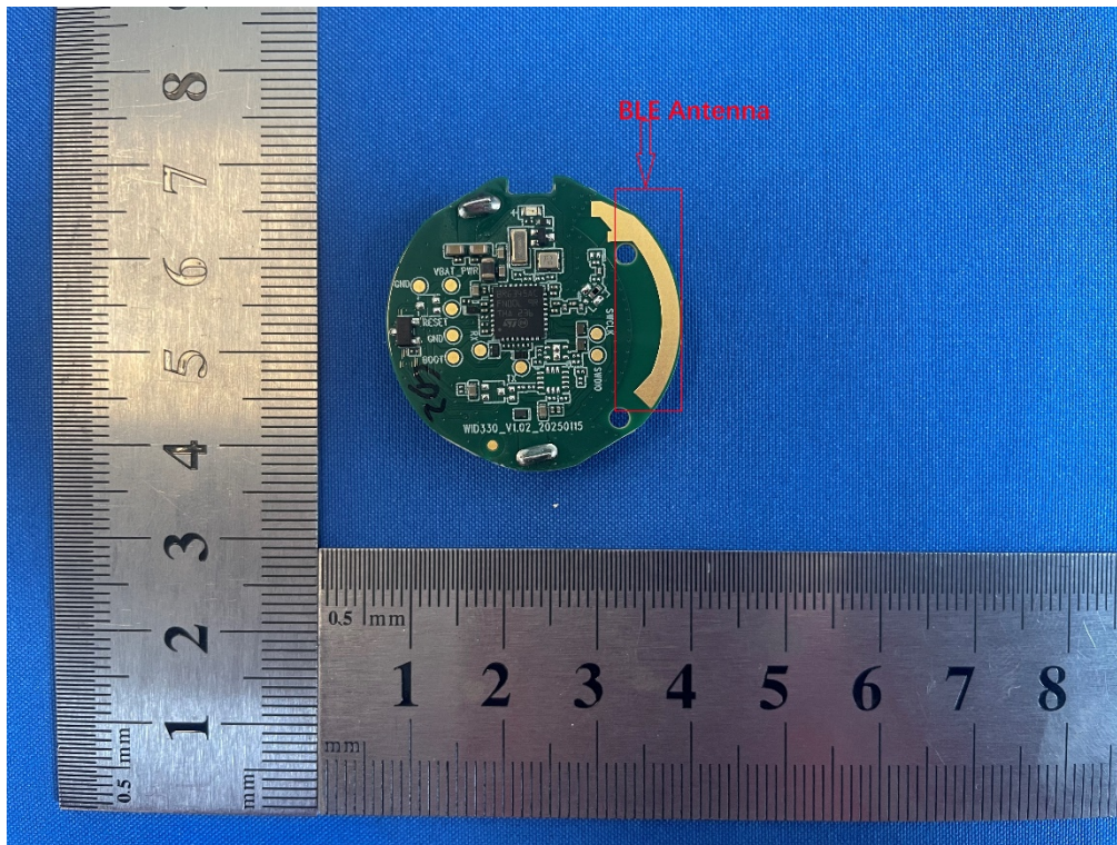
Photo 7: Internal View for BLE Antenna
