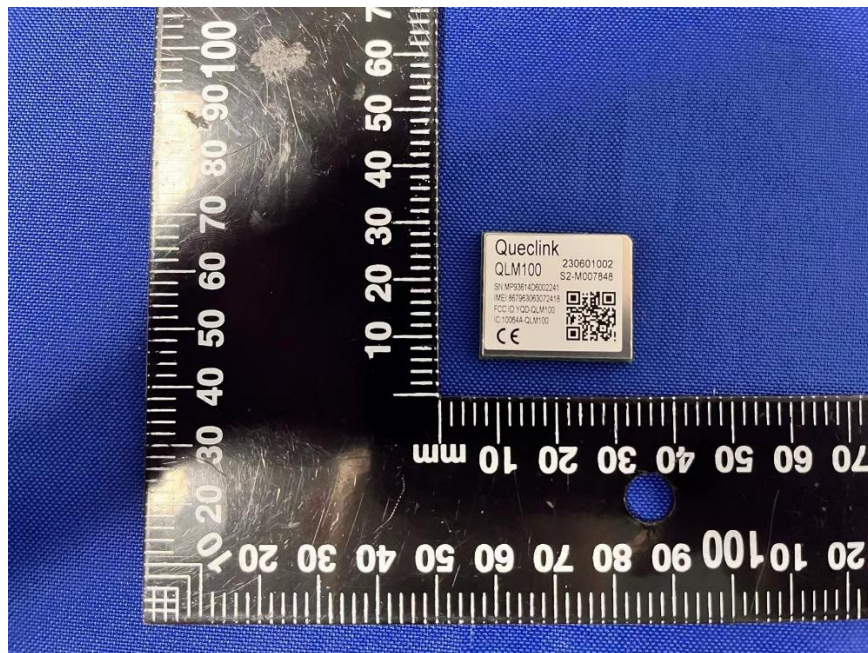
FRONT VIEW OF EUT(With Label)
