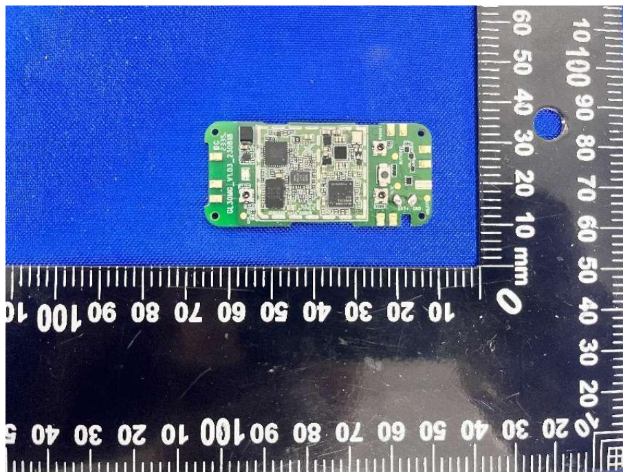
MAIN BOARD TOP VIEW (WITHOUT SHIELDING)(external GPS)
