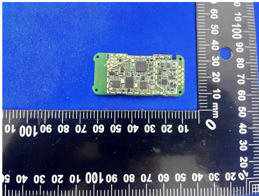
MAIN BOARD REAR VIEW (WITHOUT SHIELDING)((built-in GPS)
