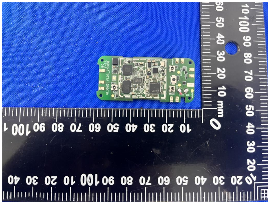
MAIN BOARD TOP VIEW (WITHOUT SHIELDING)(built-in GPS)
