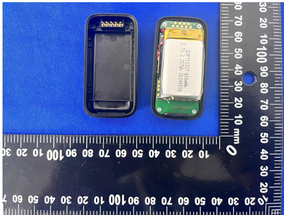
EUT UNCOVER VIEW 1(built-in GPS)
