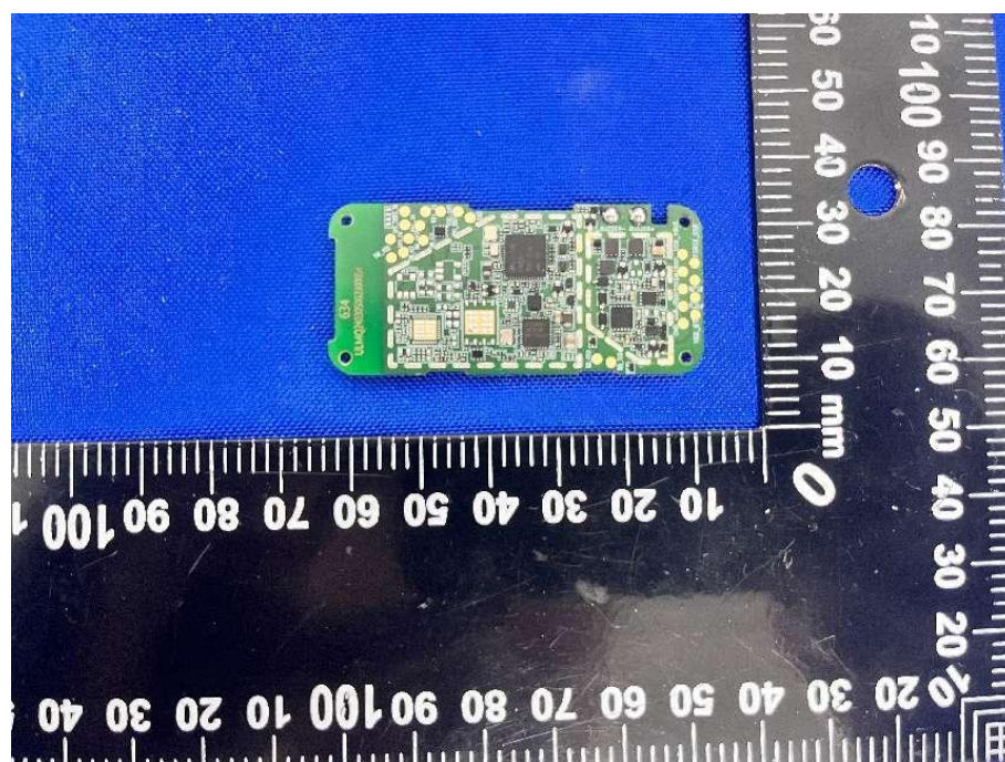
MAIN BOARD REAR VIEW (WITHOUT SHIELDING)(external GPS)
