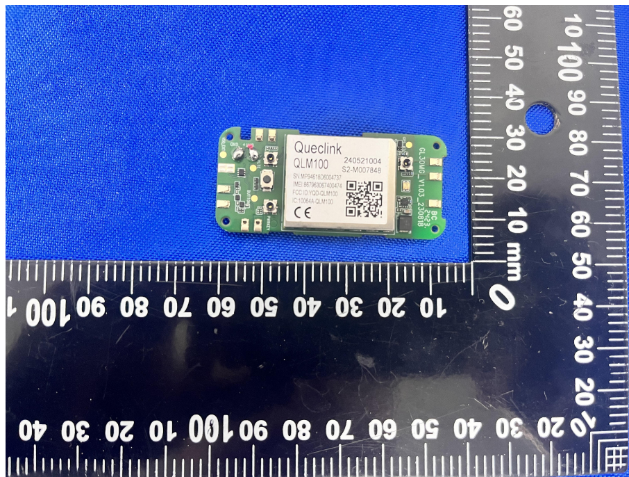
MAIN BOARD TOP VIEW (WITH SHIELDING)(built-in GPS)
