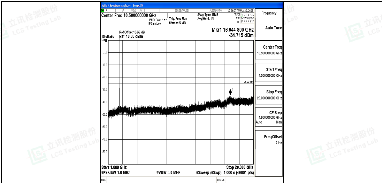
Band7_10MHz_16QAM_20800_1RB#0_1000~20000_1000~20000
