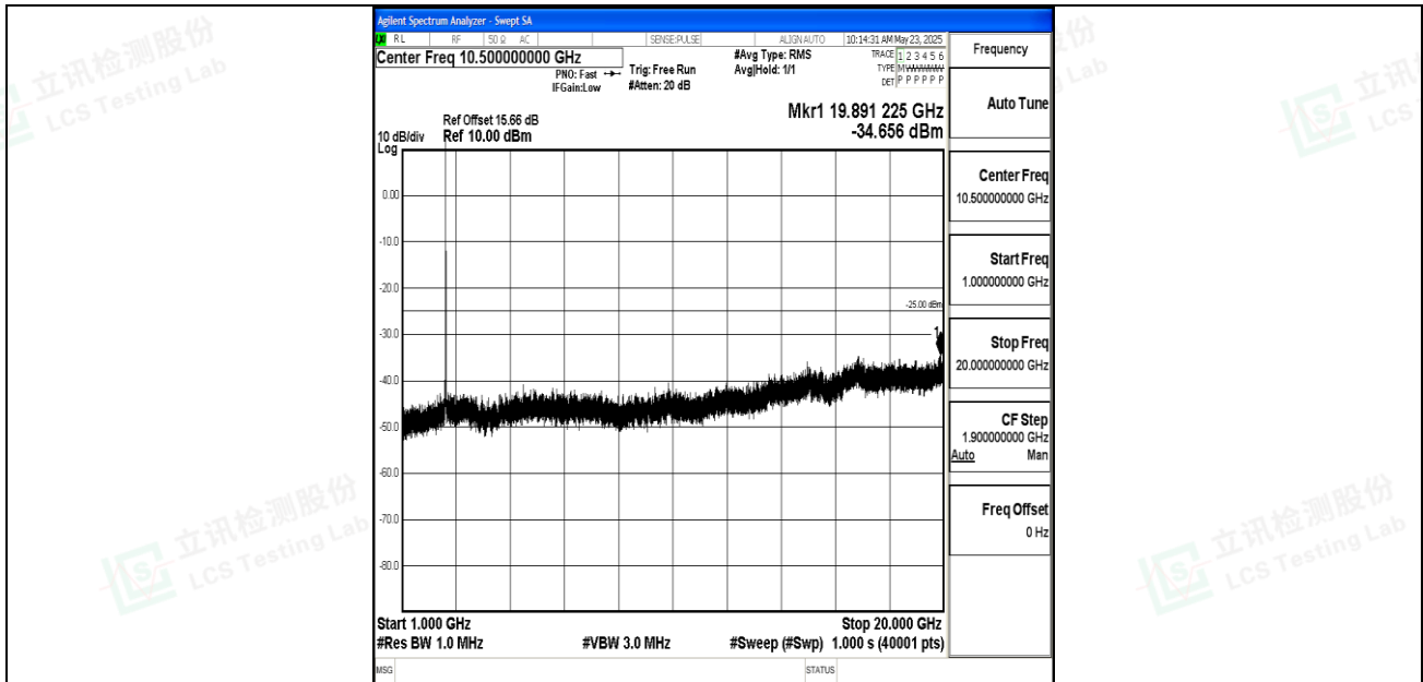
Band7_20MHz_16QAM_21100_1RB#0_1000~20000_1000~20000
