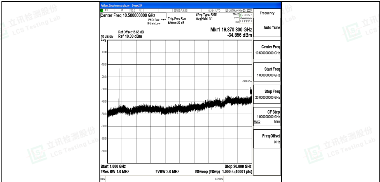
Band7_15MHz_16QAM_21100_1RB#0_1000~20000_1000~20000
