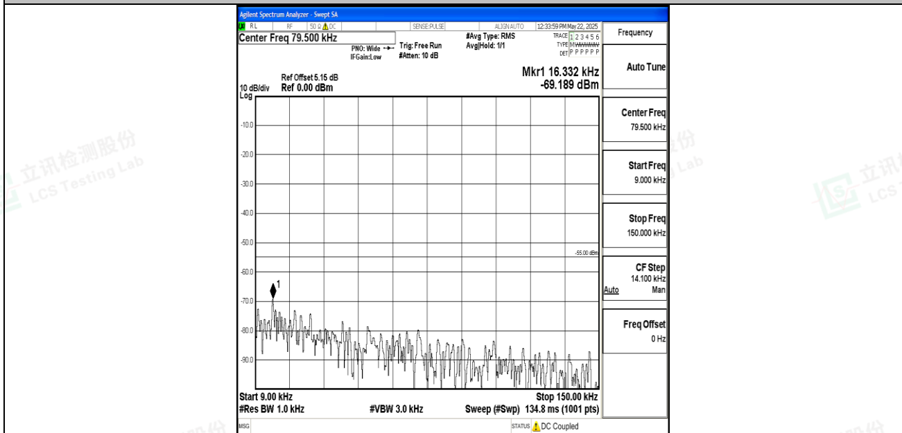
Band7_5MHz_16QAM_21425_1RB#0_0.009~0.15_0.009~0.15
