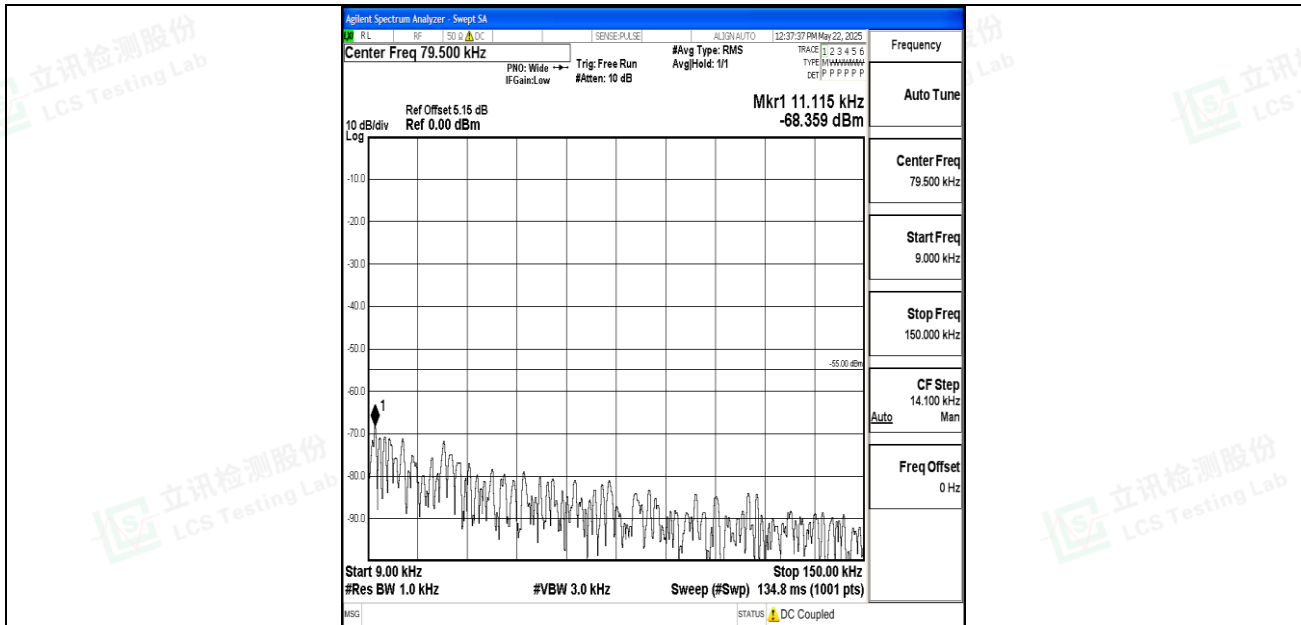
Band7_10MHz_QPSK_21400_1RB#0_0.009~0.15_0.009~0.15
