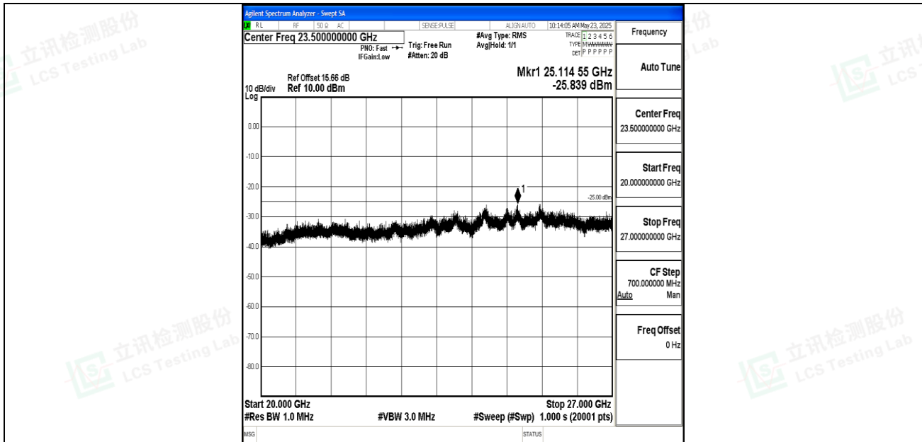
Band7_20MHz_QPSK_21100_1RB#0_20000~27000_20000~27000
