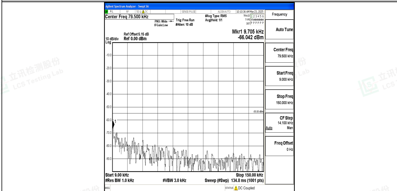
Band7_15MHz_16QAM_21100_1RB#0_0.009~0.15_0.009~0.15
