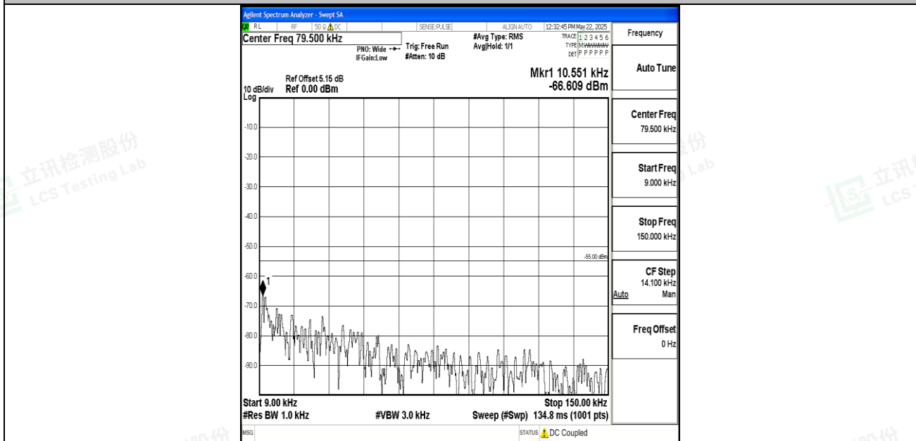
Band7_5MHz_16QAM_21100_1RB#0_0.009~0.15_0.009~0.15
