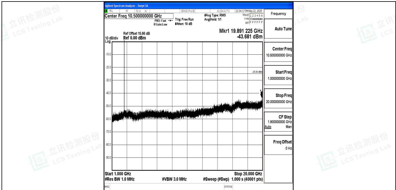
Band7_5MHz_16QAM_21425_1RB#0_1000~20000_1000~20000
