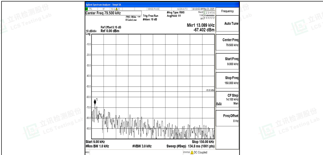
Band7_15MHz_QPSK_21100_1RB#0_0.009~0.15_0.009~0.15
