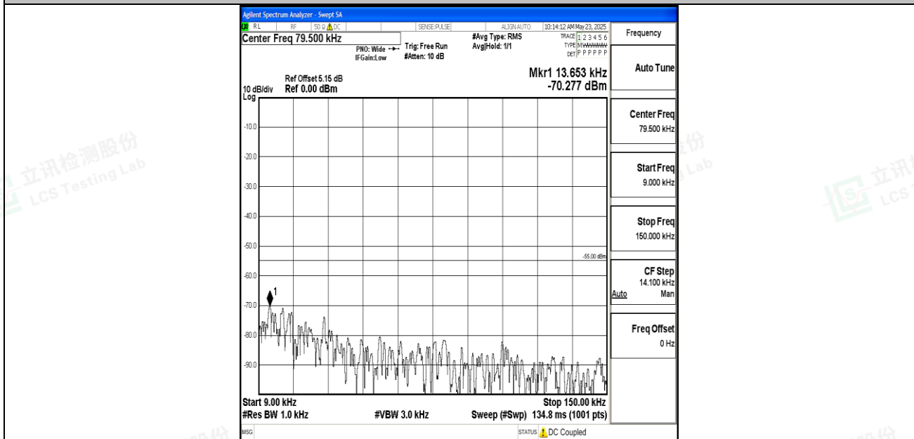
Band7_20MHz_16QAM_21100_1RB#0_0.009~0.15_0.009~0.15
