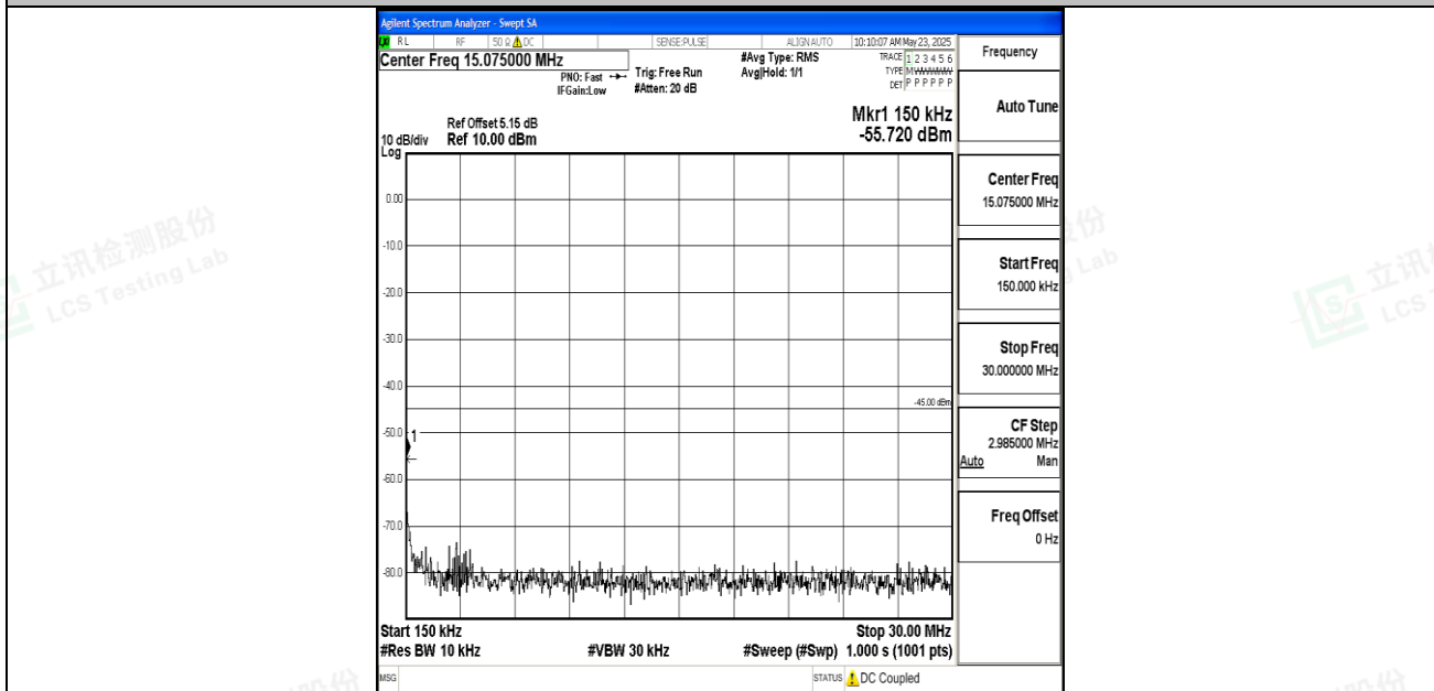
Band7_15MHz_QPSK_21100_1RB#0_0.15~30_0.15~30
