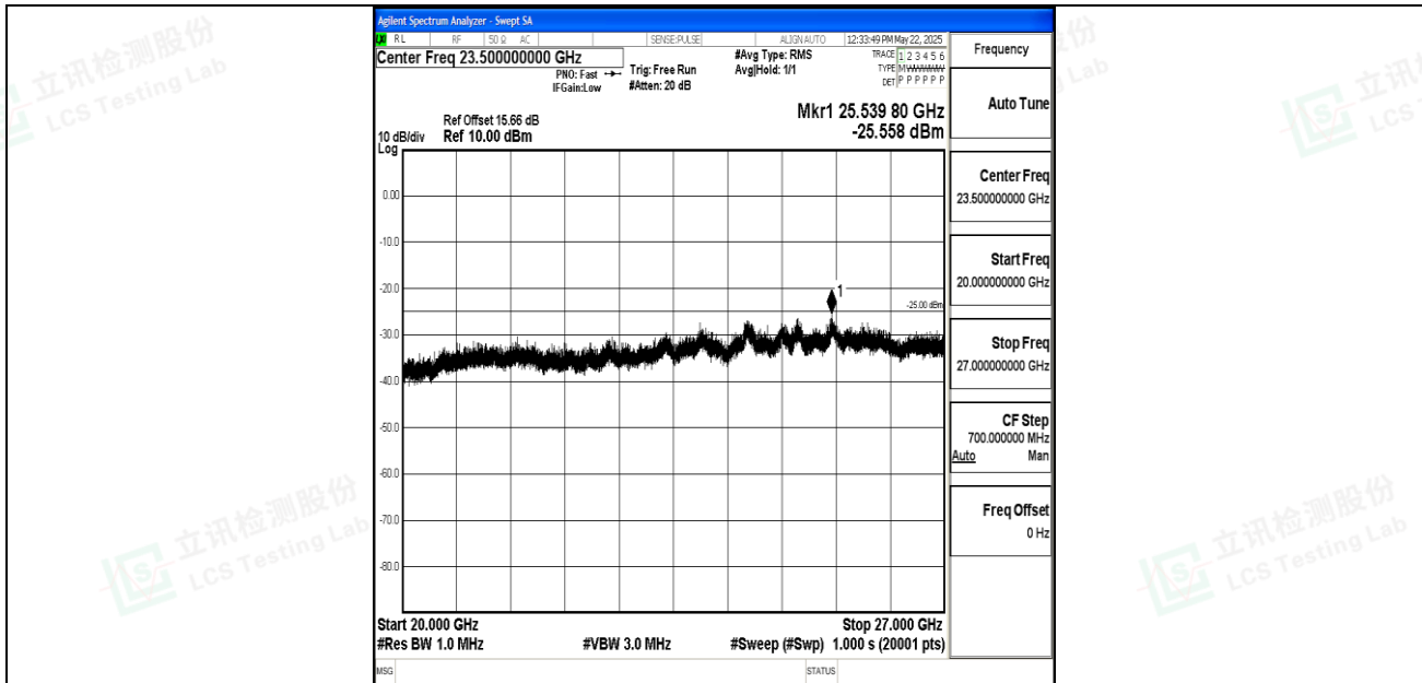
Band7_5MHz_QPSK_21425_1RB#0_20000~27000_20000~27000
