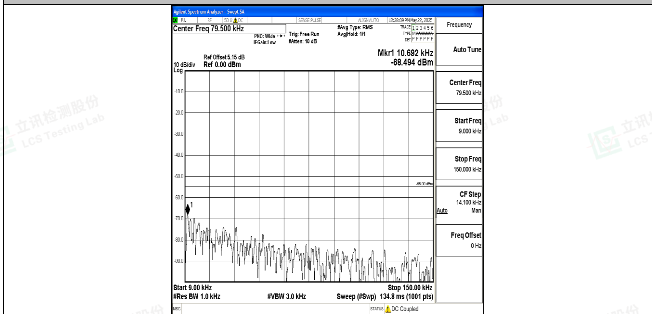
Band7_10MHz_16QAM_21400_1RB#0_0.009~0.15_0.009~0.15
