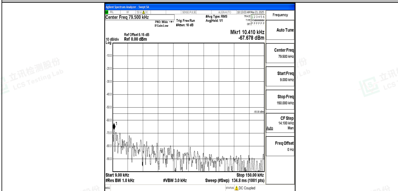
Band7_20MHz_16QAM_20850_1RB#0_0.009~0.15_0.009~0.15
