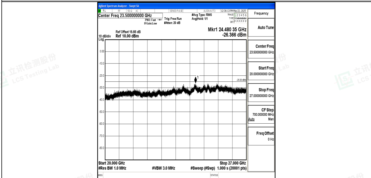
Band7_10MHz_16QAM_20800_1RB#0_20000~27000_20000~27000
