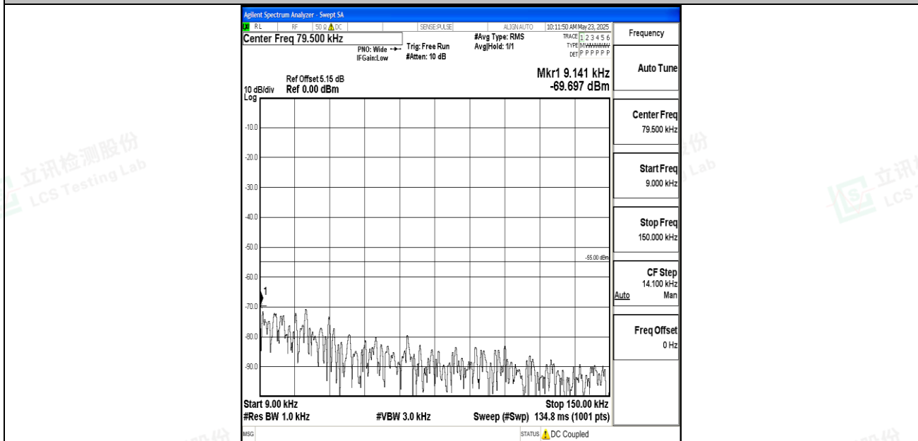
Band7_15MHz_16QAM_21375_1RB#0_0.009~0.15_0.009~0.15
