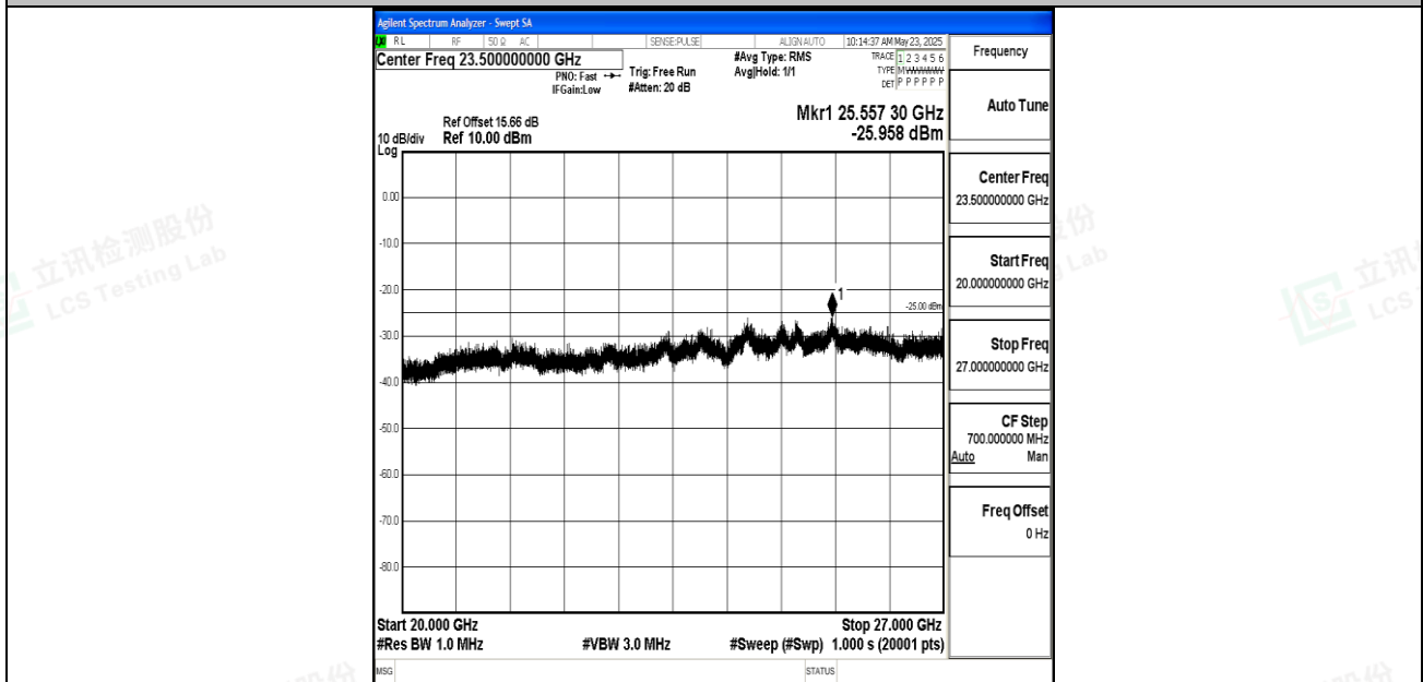
Band7_20MHz_16QAM_21100_1RB#0_20000~27000_20000~27000
