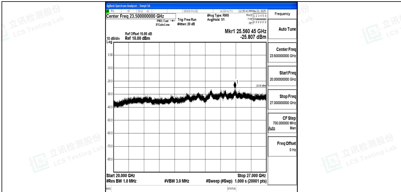
Band7_10MHz_QPSK_20800_1RB#0_20000~27000_20000~27000
