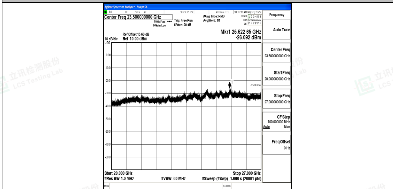
Band7_15MHz_16QAM_21375_1RB#0_20000~27000_20000~27000
