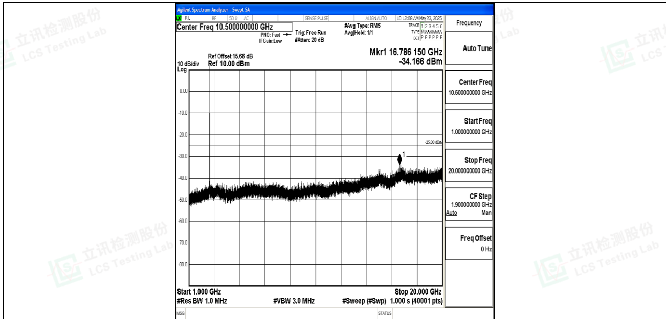
Band7_15MHz_16QAM_21375_1RB#0_1000~20000_1000~20000
