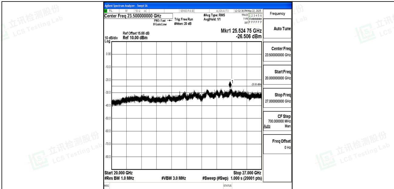
Band7_5MHz_QPSK_21100_1RB#0_20000~27000_20000~27000
