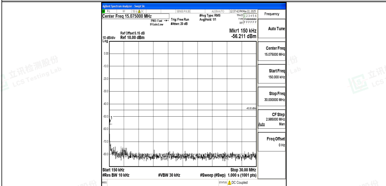
Band7_10MHz_QPSK_21400_1RB#0_0.15~30_0.15~30
