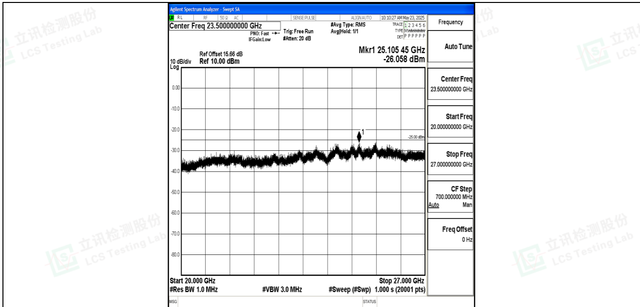
Band7_15MHz_QPSK_21100_1RB#0_20000~27000_20000~27000
