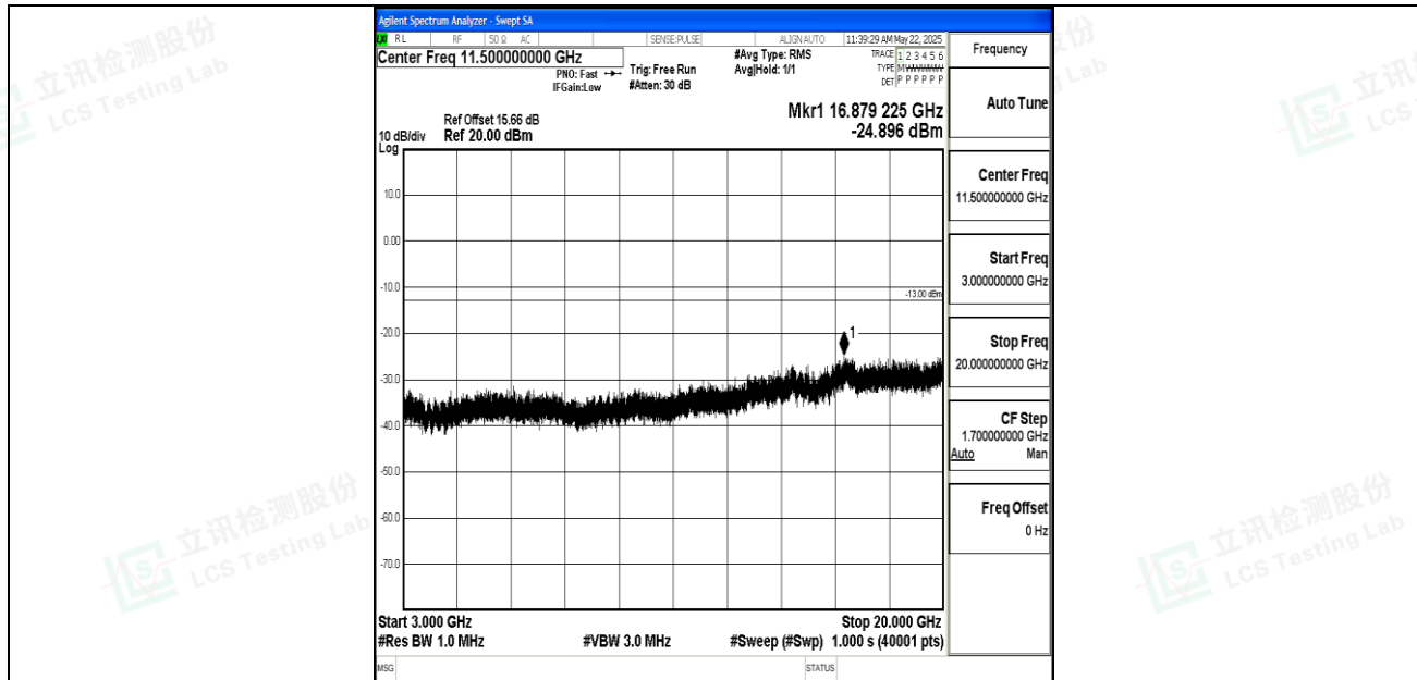
Band2_20MHz_16QAM_18900_1RB#0_3000~20000_3000~20000
