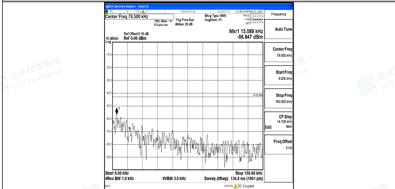
Band2_20MHz_QPSK_18900_1RB#0_0.009~0.15_0.009~0.15
