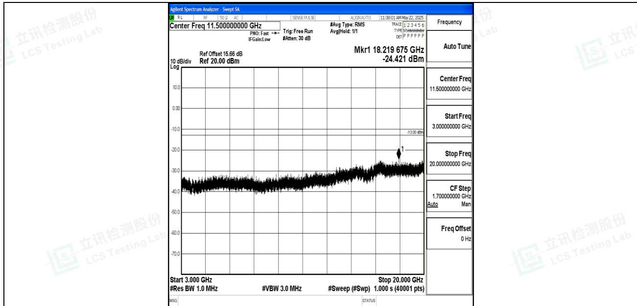
Band2_20MHz_16QAM_18700_1RB#0_3000~20000_3000~20000
