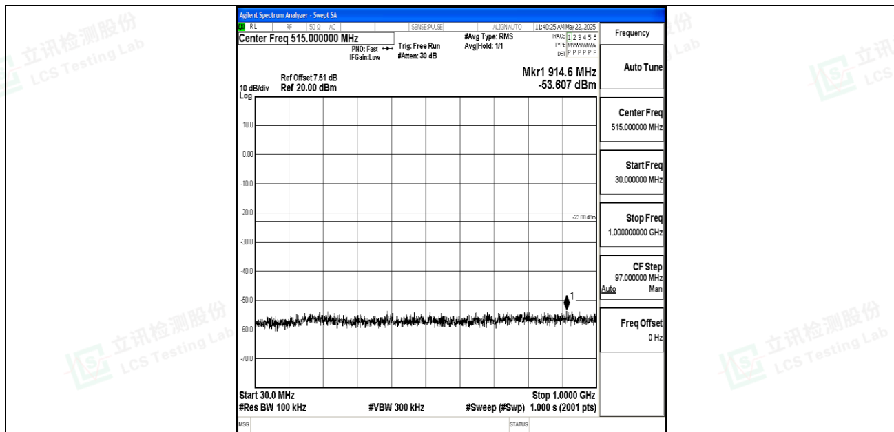
Band2_20MHz_16QAM_19100_1RB#0_30~1000_30~1000
