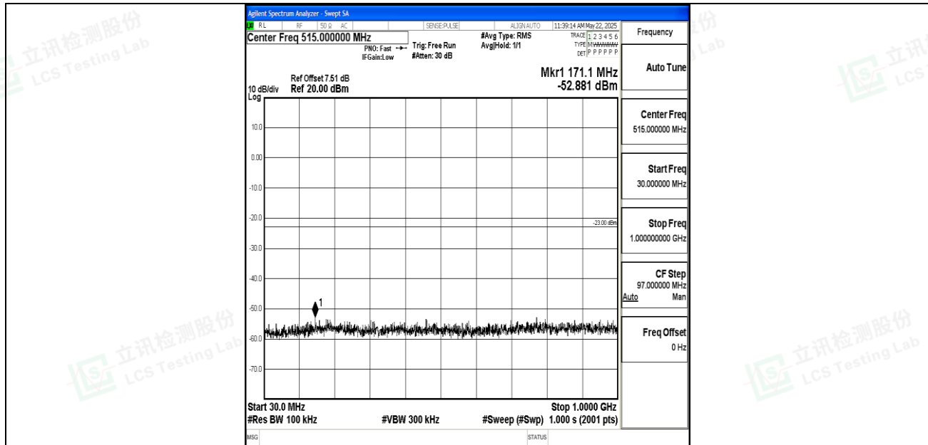
Band2_20MHz_16QAM_18900_1RB#0_30~1000_30~1000
