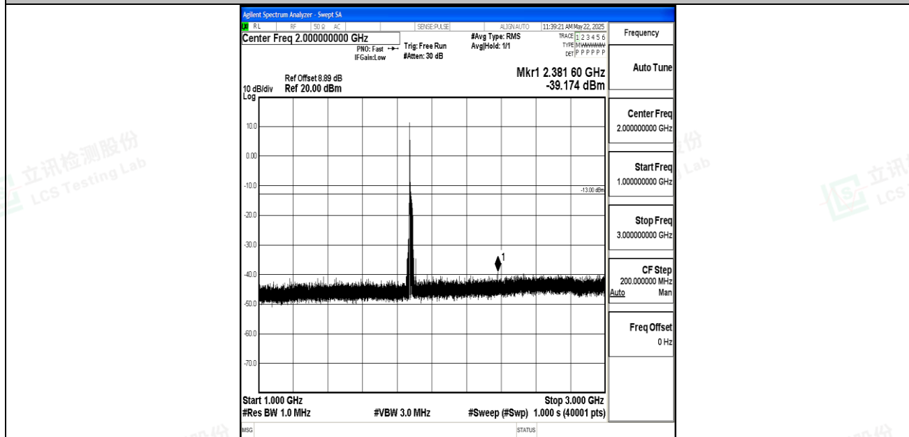
Band2_20MHz_16QAM_18900_1RB#0_1000~3000_1000~3000
