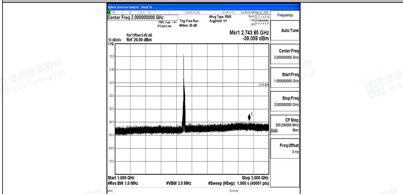
Band2_20MHz_16QAM_19100_1RB#0_1000~3000_1000~3000
