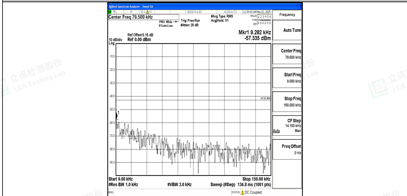
Band2_20MHz_QPSK_19100_1RB#0_0.009~0.15_0.009~0.15
