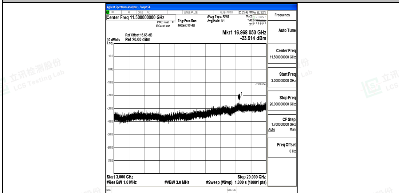
Band2_5MHz_QPSK_18900_1RB#0_3000~20000_3000~20000
