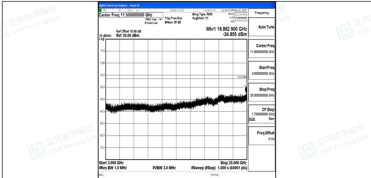
Band2_10MHz_16QAM_18900_1RB#0_3000~20000_3000~20000
