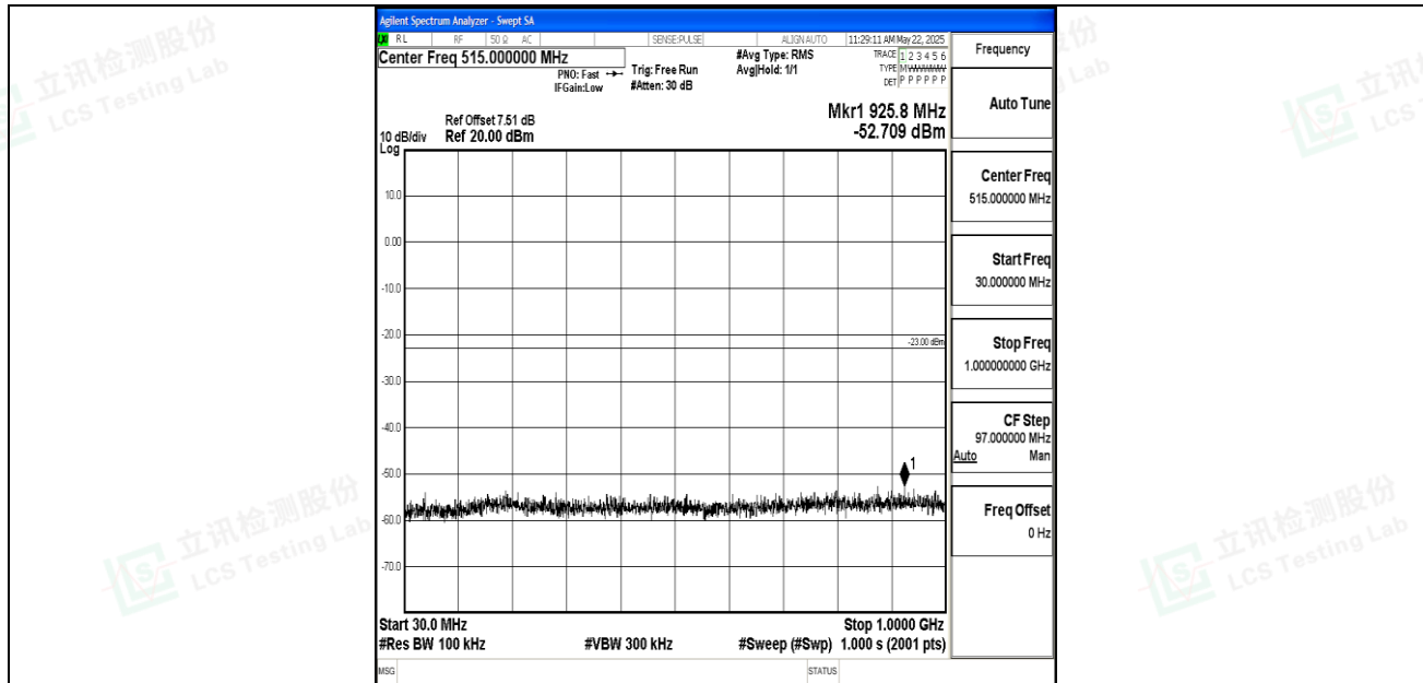
Band2_10MHz_16QAM_18650_1RB#0_30~1000_30~1000
