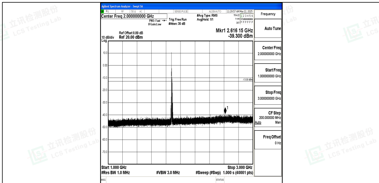
Band2_10MHz_QPSK_18900_1RB#0_1000~3000_1000~3000
