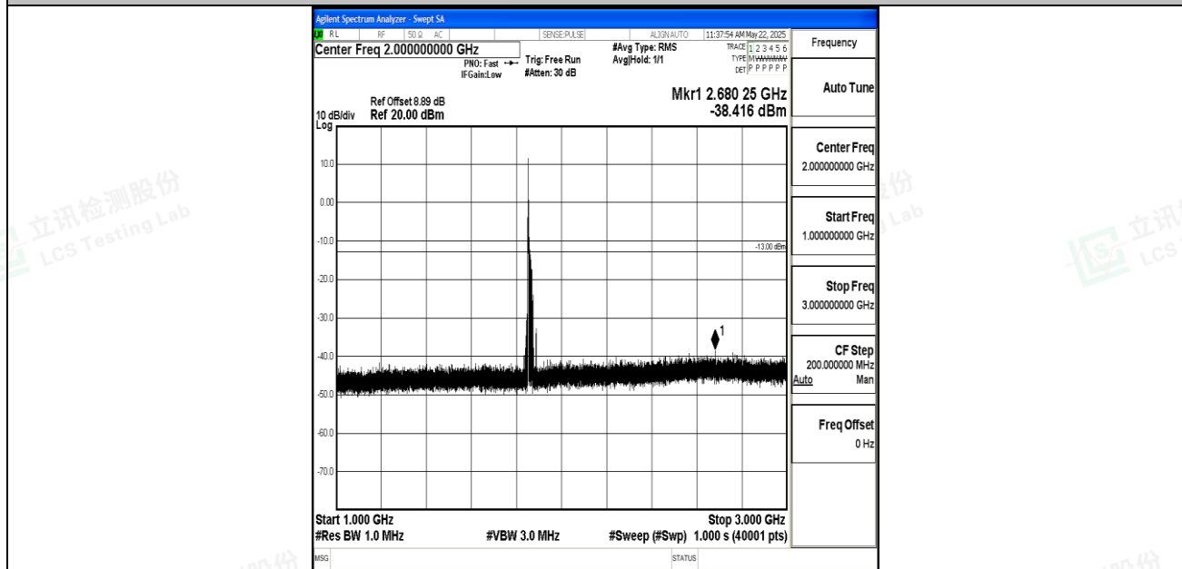
Band2_20MHz_16QAM_18700_1RB#0_1000~3000_1000~3000
