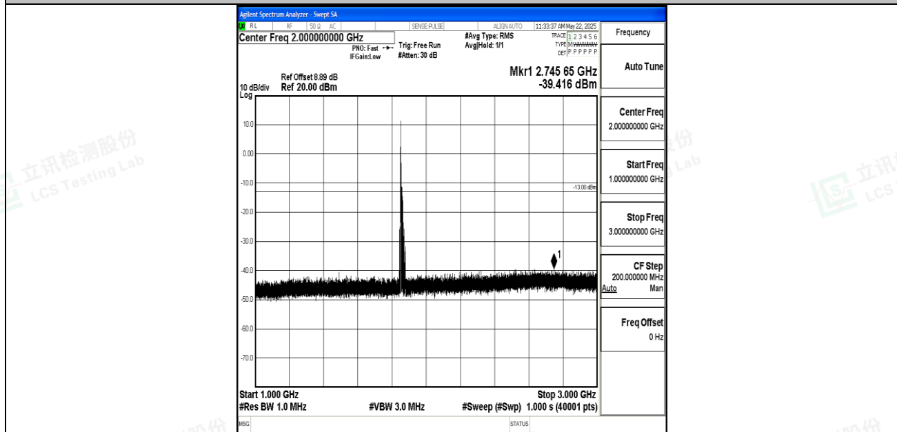
Band2_15MHz_16QAM_18675_1RB#0_1000~3000_1000~3000
