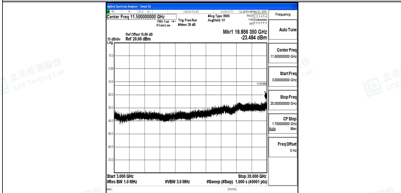
Band2_10MHz_QPSK_18650_1RB#0_3000~20000_3000~20000
