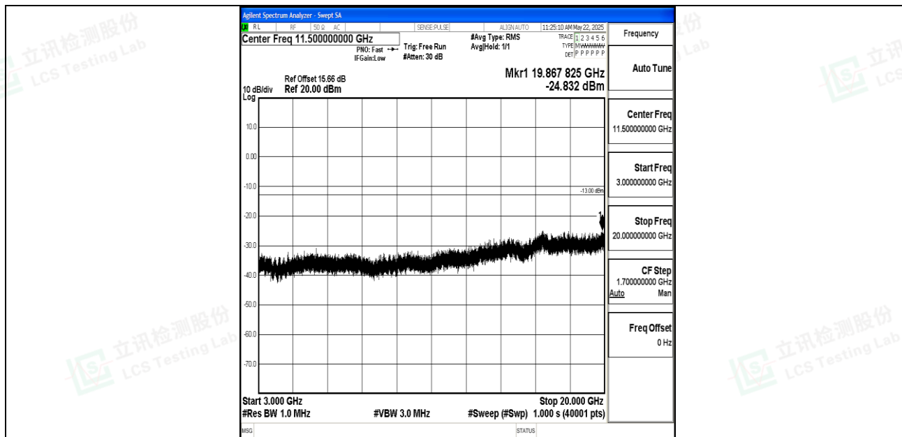
Band2_5MHz_16QAM_18625_1RB#0_3000~20000_3000~20000
