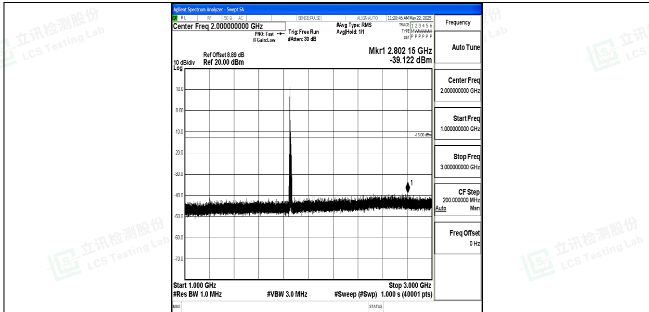
Band2_10MHz_QPSK_18650_1RB#0_1000~3000_1000~3000
