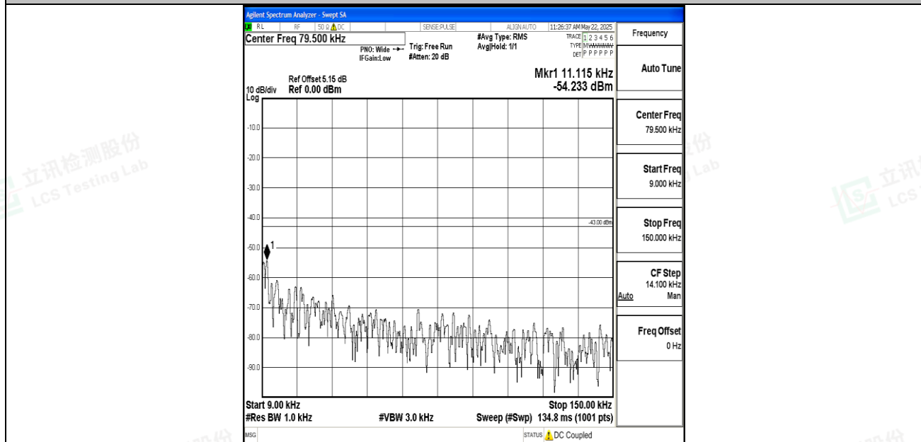
Band2_5MHz_QPSK_19175_1RB#0_0.009~0.15_0.009~0.15
