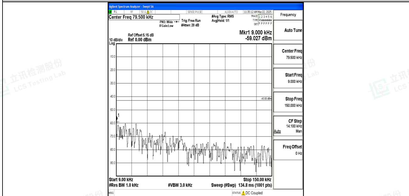
Band2_15MHz_QPSK_19125_1RB#0_0.009~0.15_0.009~0.15
