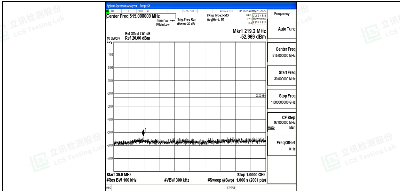
Band2_10MHz_16QAM_18900_1RB#0_30~1000_30~1000
