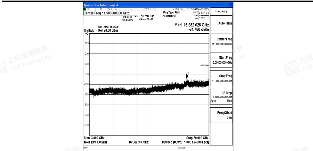
Band2_10MHz_QPSK_18900_1RB#0_3000~20000_3000~20000
