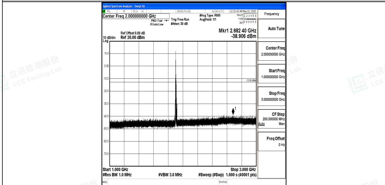
Band2_10MHz_16QAM_19150_1RB#0_1000~3000_1000~3000
