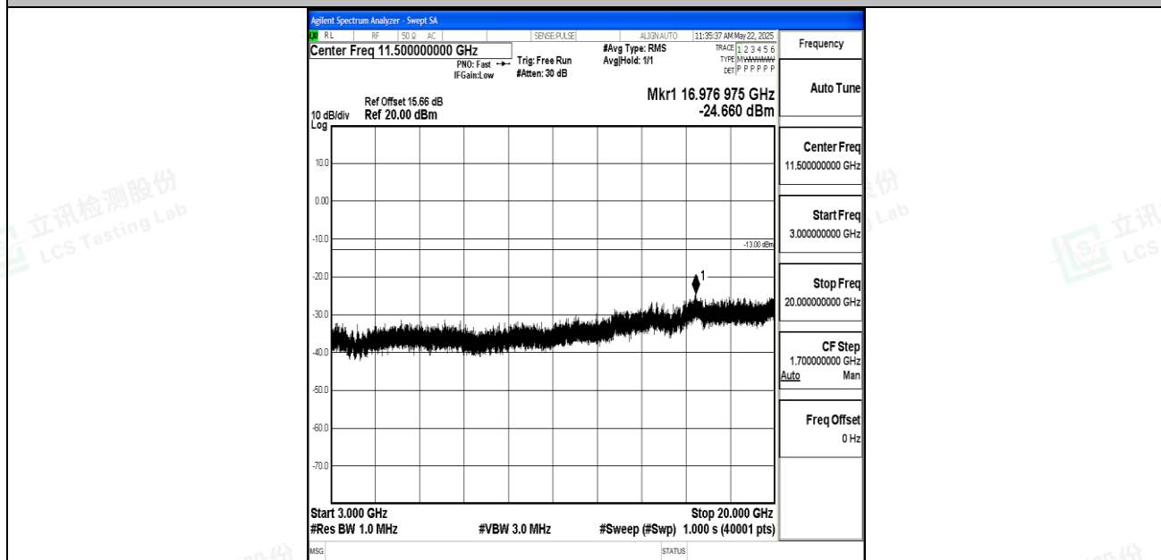
Band2_15MHz_QPSK_19125_1RB#0_3000~20000_3000~20000
