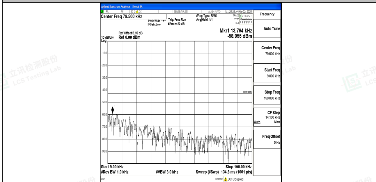
Band2_5MHz_QPSK_18900_1RB#0_0.009~0.15_0.009~0.15
