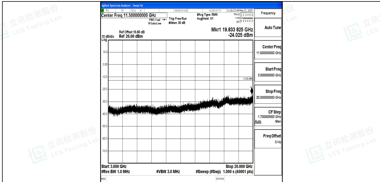
Band2_5MHz_16QAM_18900_1RB#0_3000~20000_3000~20000
