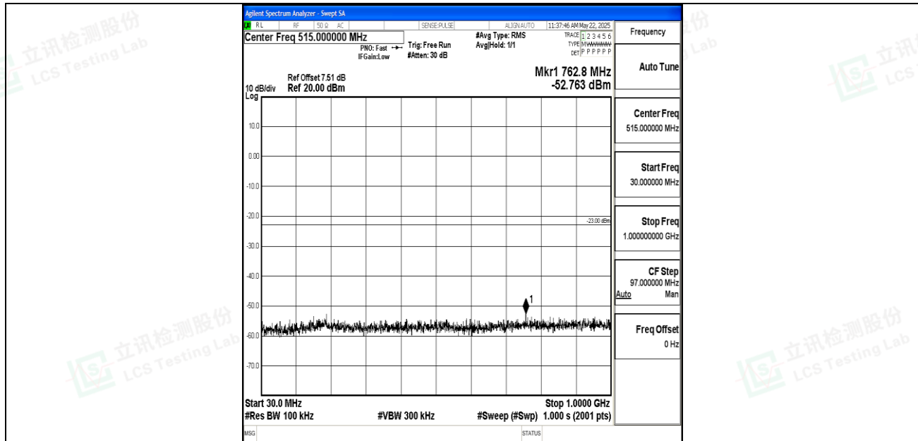
Band2_20MHz_16QAM_18700_1RB#0_30~1000_30~1000
