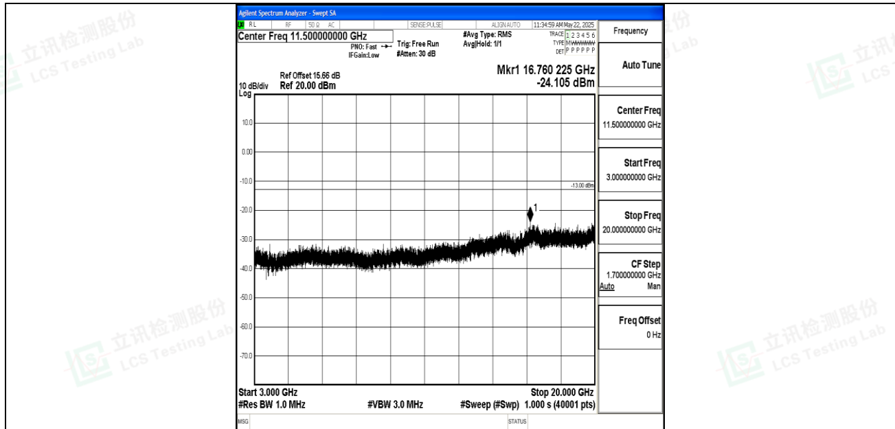
Band2_15MHz_16QAM_18900_1RB#0_3000~20000_3000~20000
