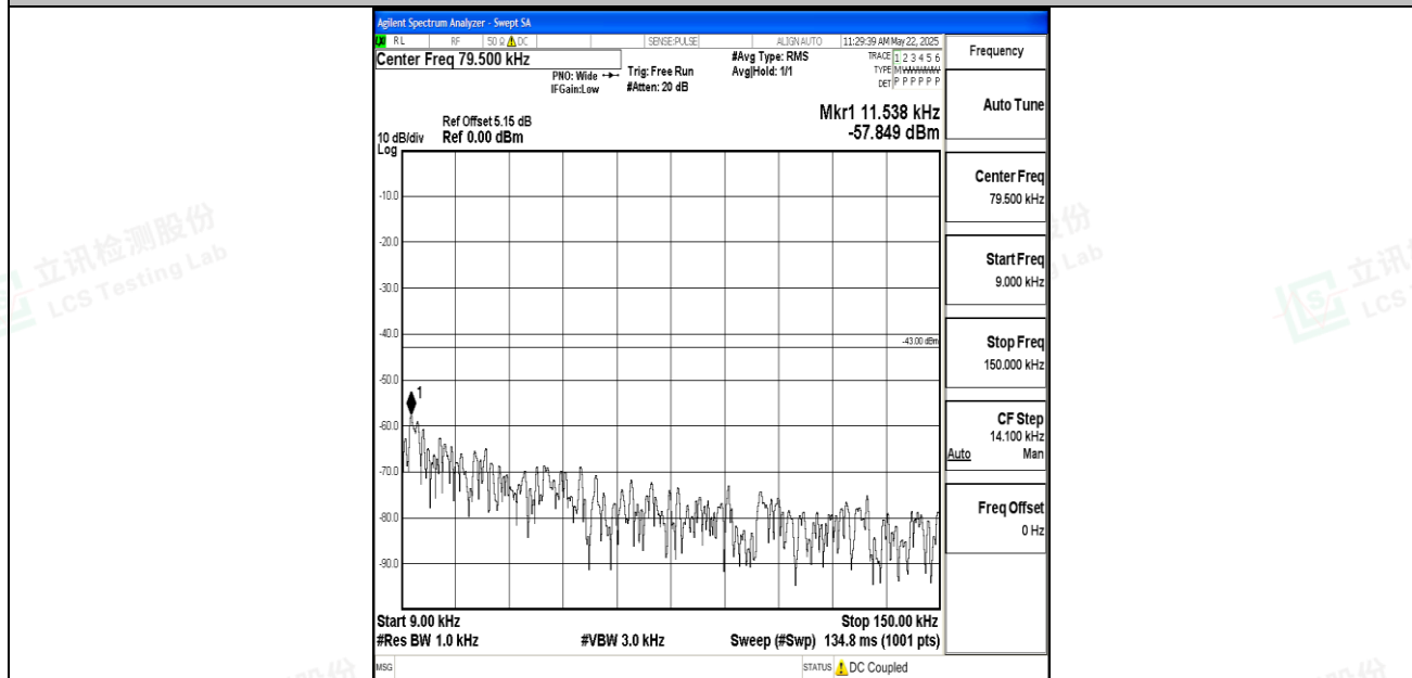
Band2_10MHz_QPSK_18900_1RB#0_0.009~0.15_0.009~0.15
