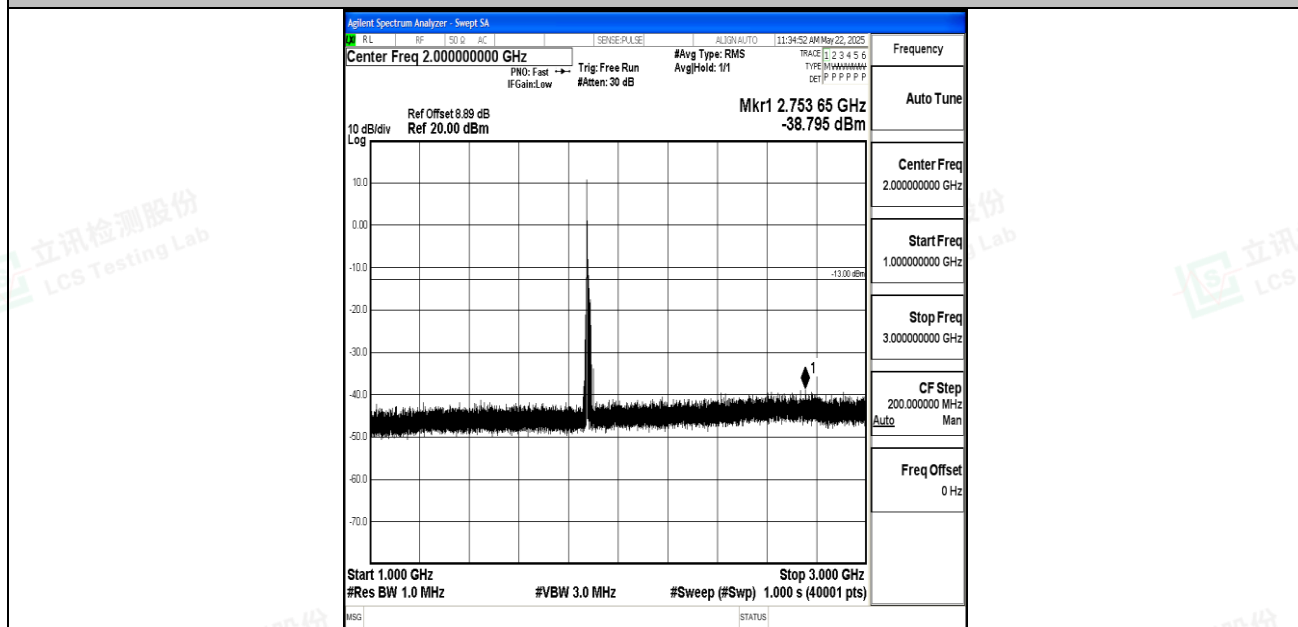
Band2_15MHz_16QAM_18900_1RB#0_1000~3000_1000~3000
