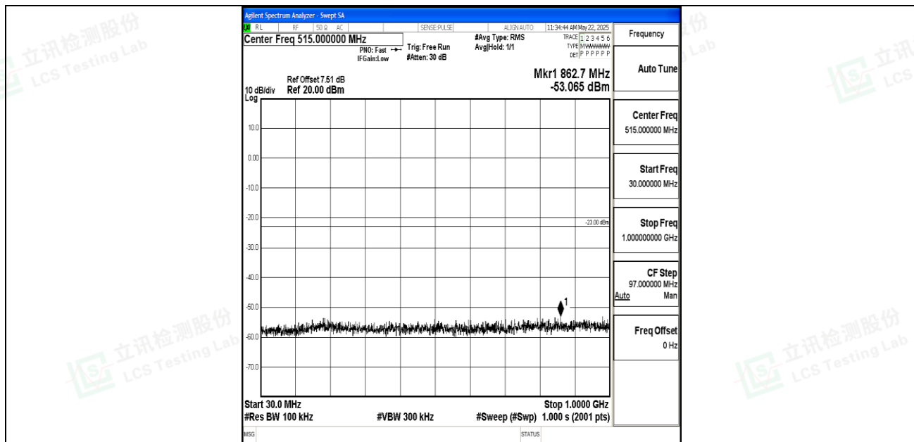
Band2_15MHz_16QAM_18900_1RB#0_30~1000_30~1000
