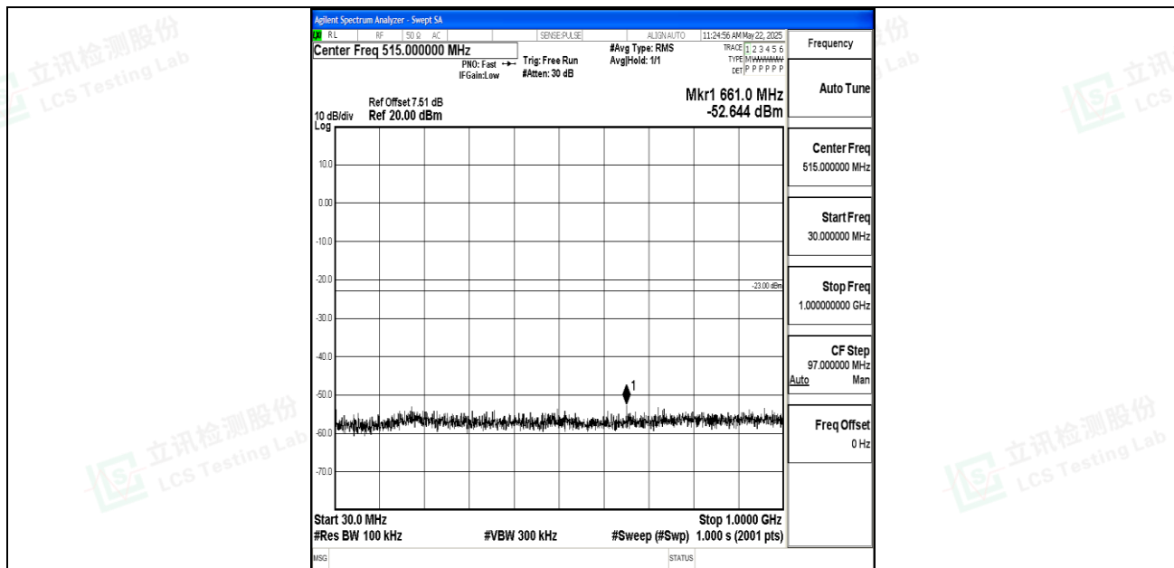
Band2_5MHz_16QAM_18625_1RB#0_30~1000_30~1000
