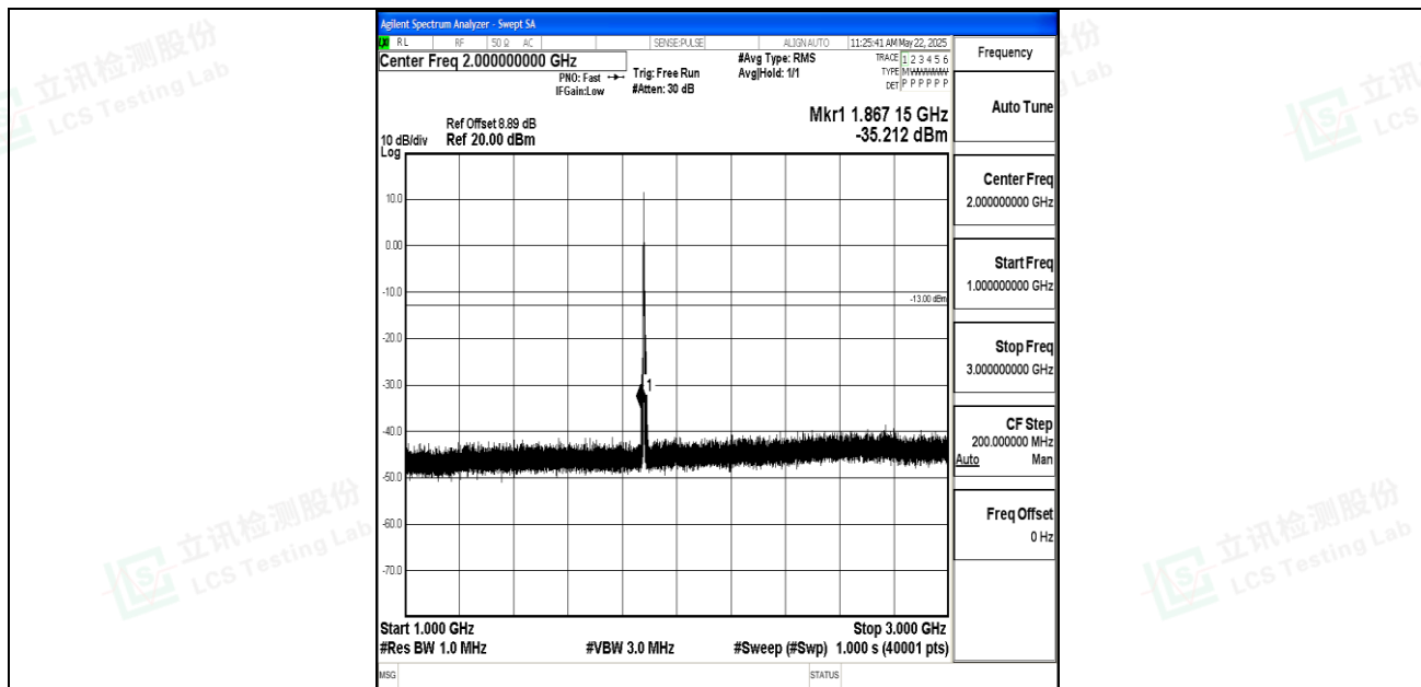
Band2_5MHz_QPSK_18900_1RB#0_1000~3000_1000~3000
