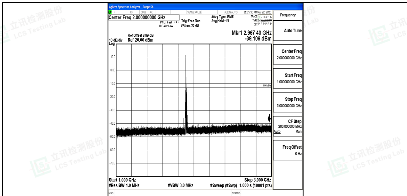
Band2_15MHz_QPSK_19125_1RB#0_1000~3000_1000~3000
