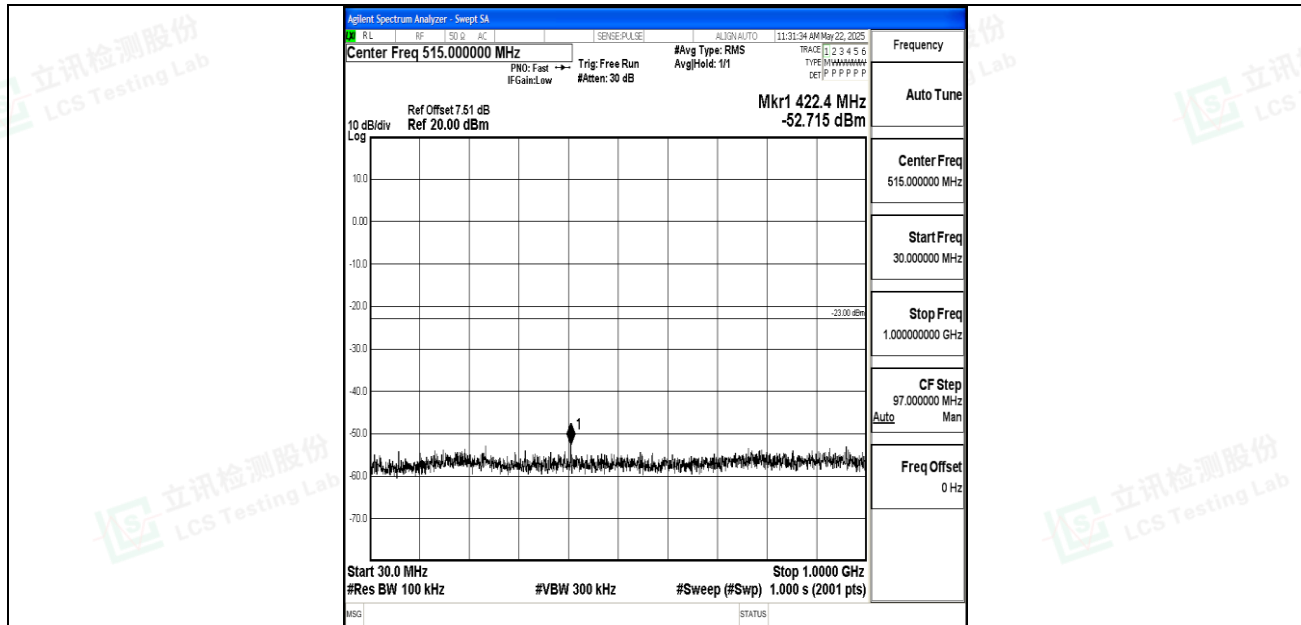
Band2_10MHz_16QAM_19150_1RB#0_30~1000_30~1000
