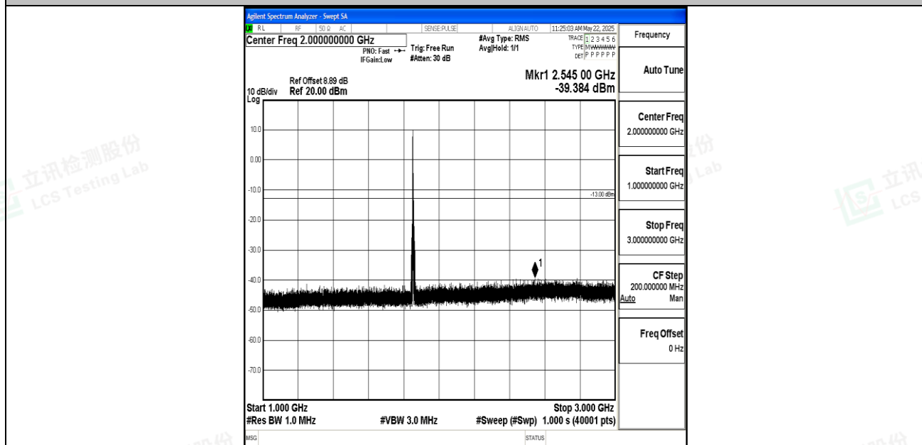
Band2_5MHz_16QAM_18625_1RB#0_1000~3000_1000~3000
