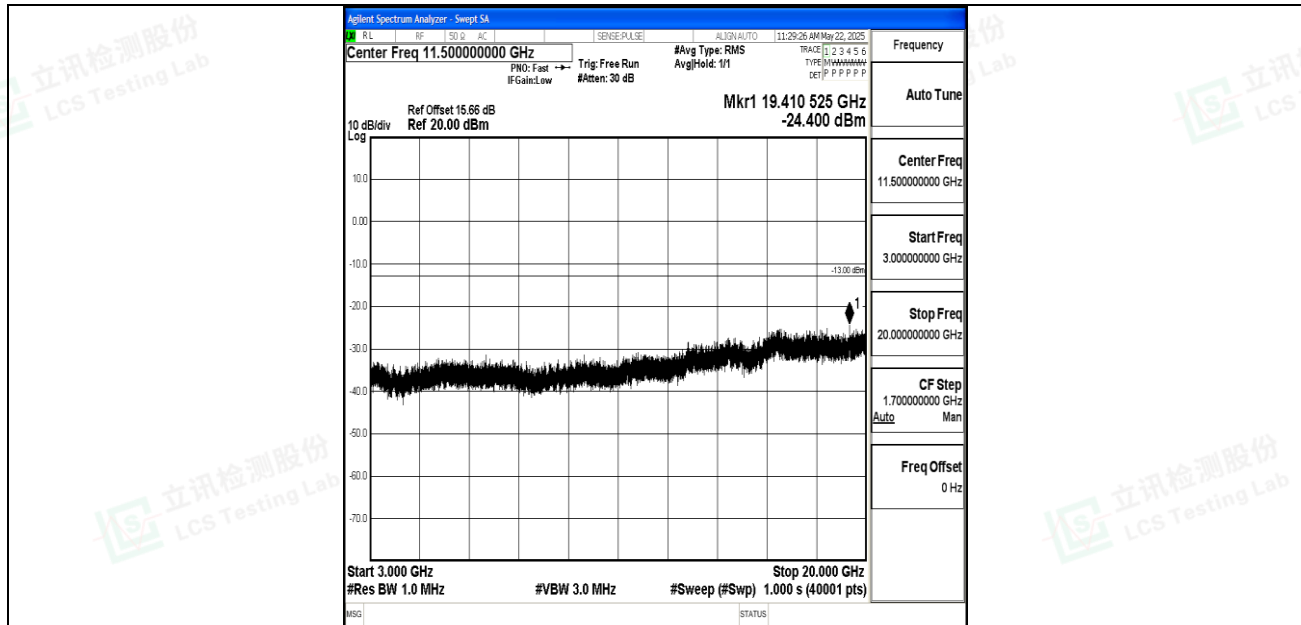
Band2_10MHz_16QAM_18650_1RB#0_3000~20000_3000~20000
