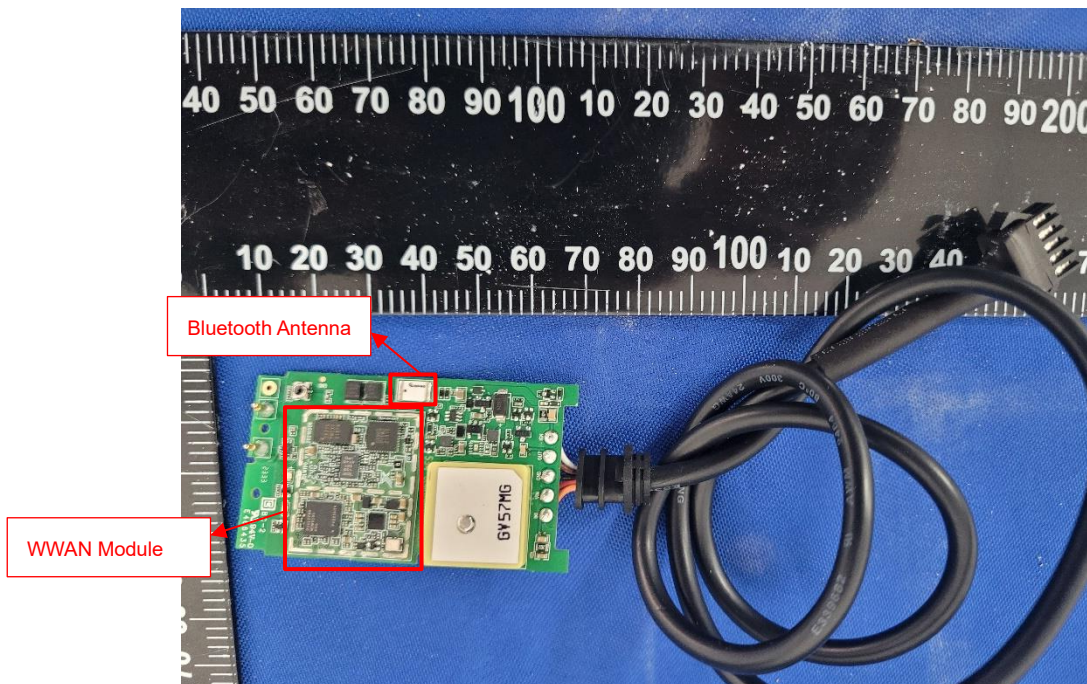
MAIN BOARD TOP VIEW (WITHOUT SHIELDING)
