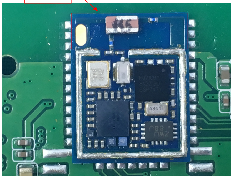
Antenna for BT/BLE
