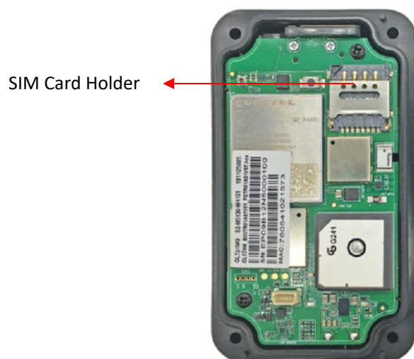
Figure 6. GL521MG SIM Card Holder
