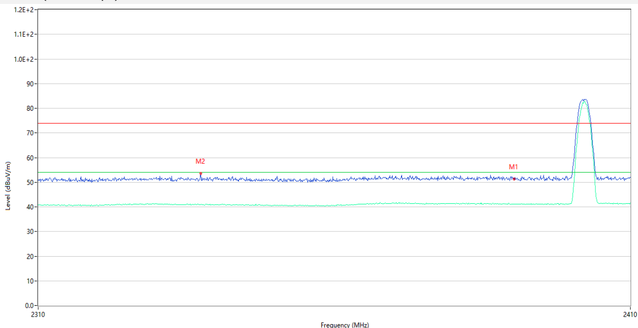
GFSK (BLE 1Mbps) LOW CHANNEL, ANT H
