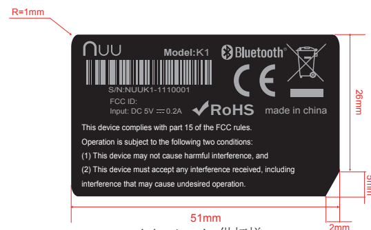
1:1 artwork. 供打样
