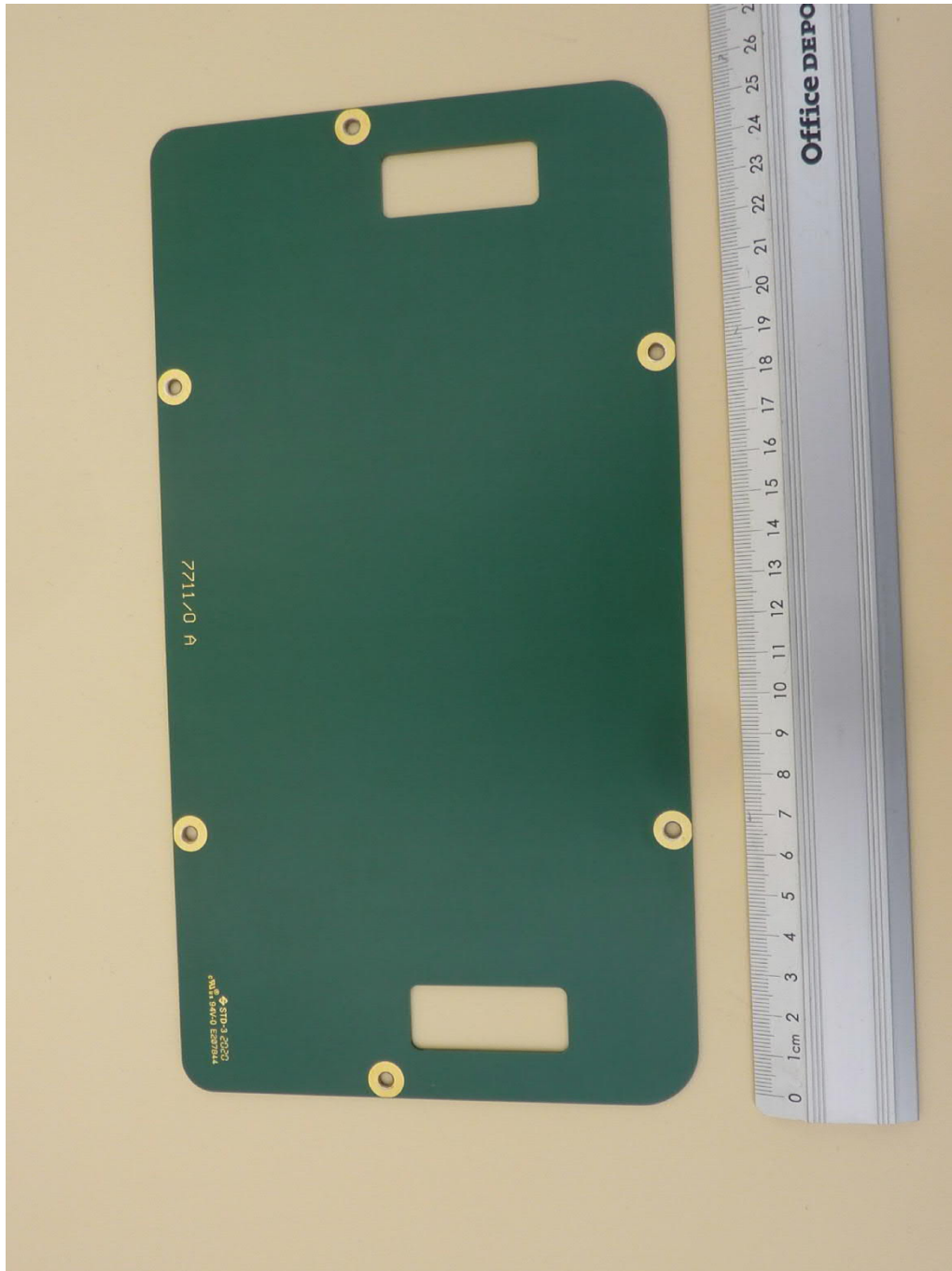
TN-UHF-Q180L300-NA-CDS, shield, bottom view
