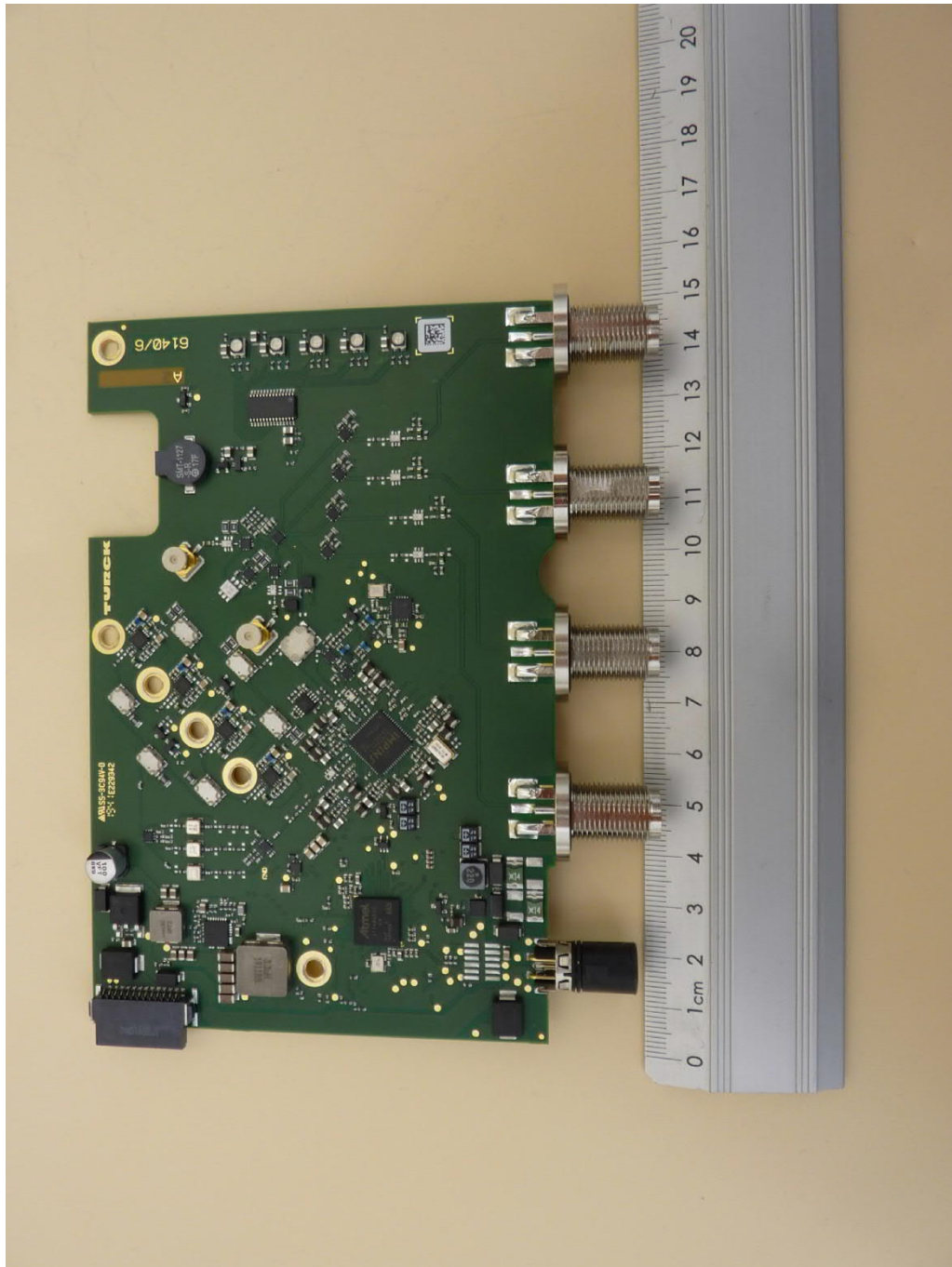
TN-UHF-Q180L300-NA-CDS, rf PCB, top view
