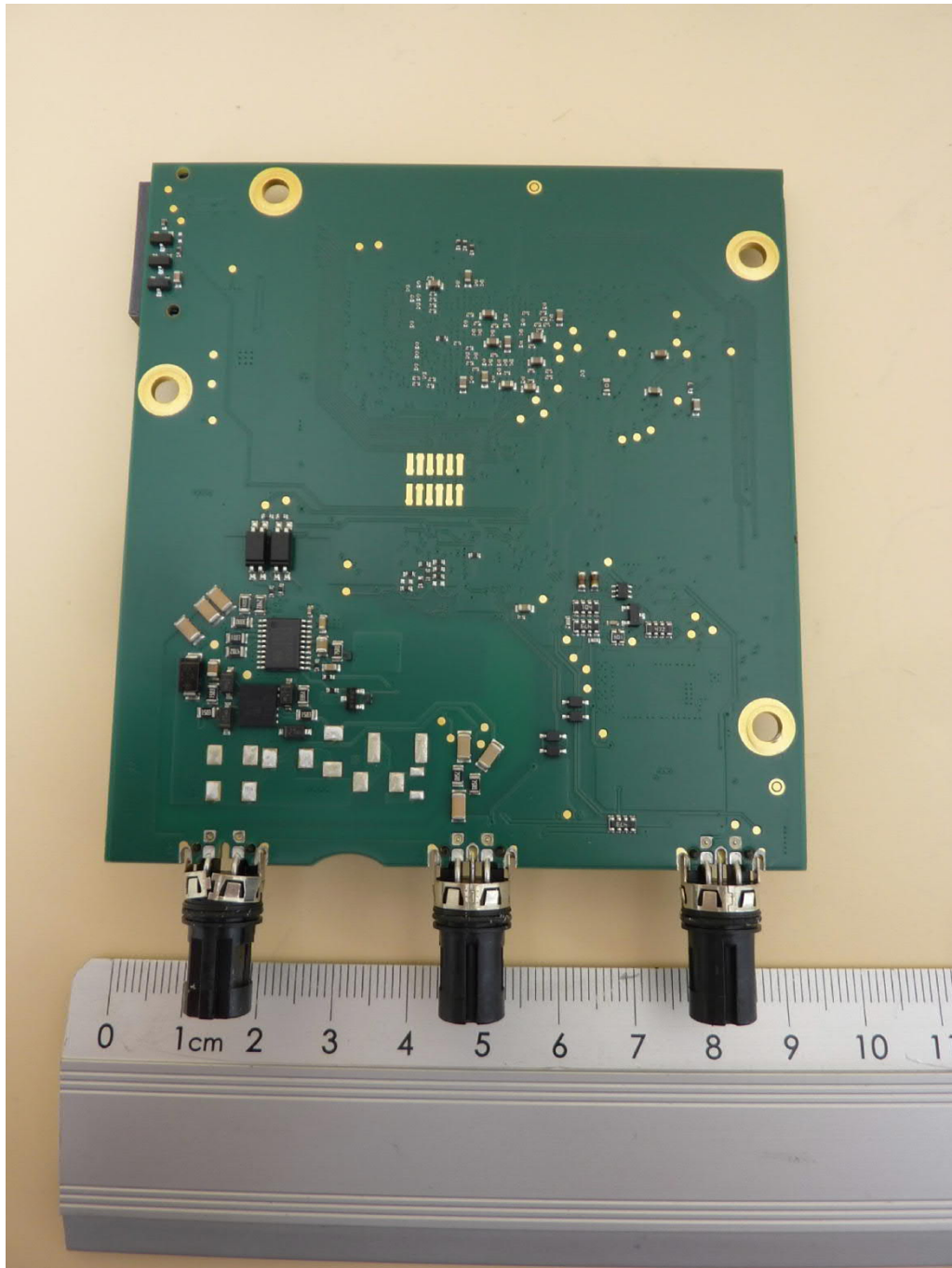
TN-UHF-Q180L300-NA-CDS, digital PCB, bottom view
