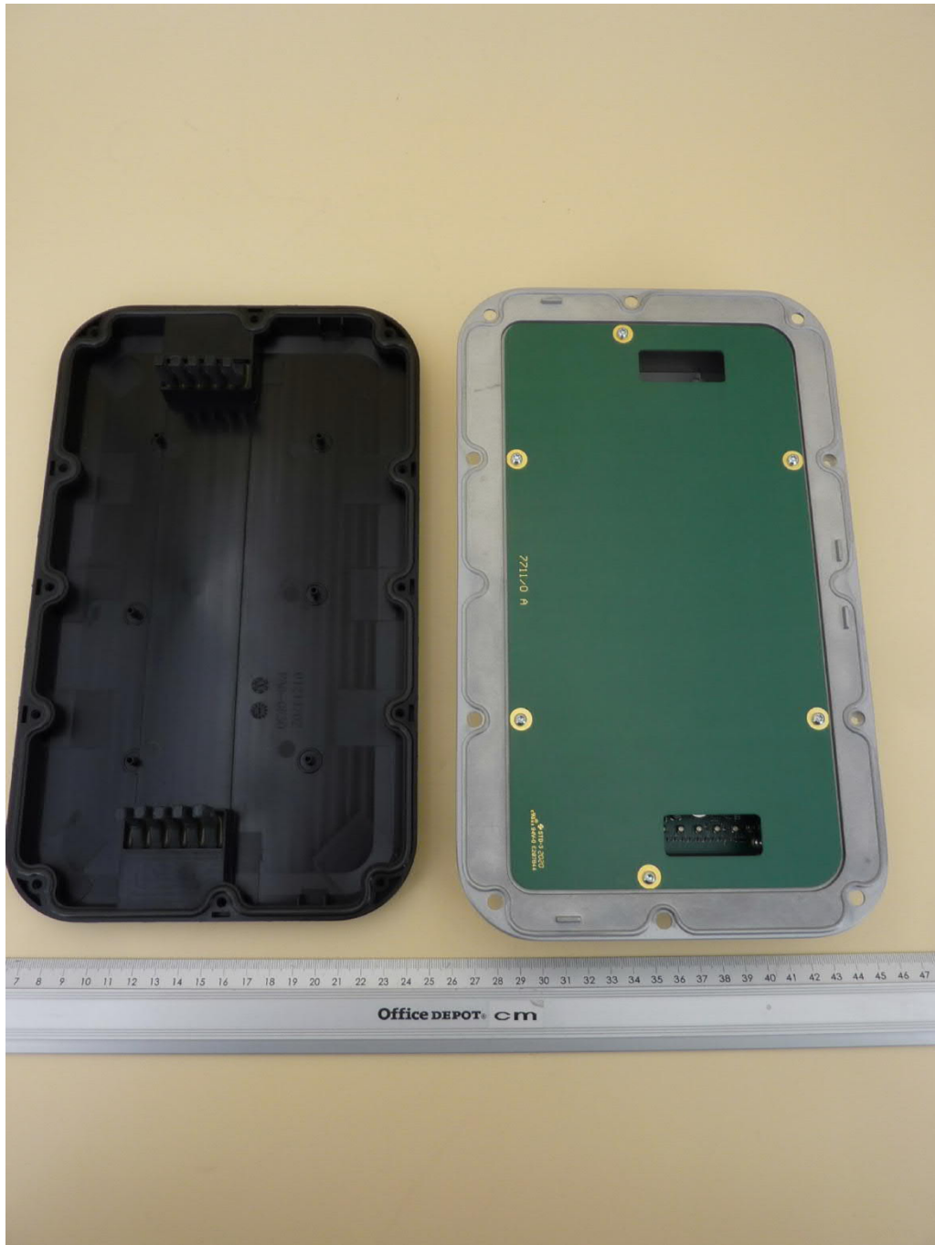
TN-UHF-Q180L300-NA-CDS, internal view 1 (housing opened)
