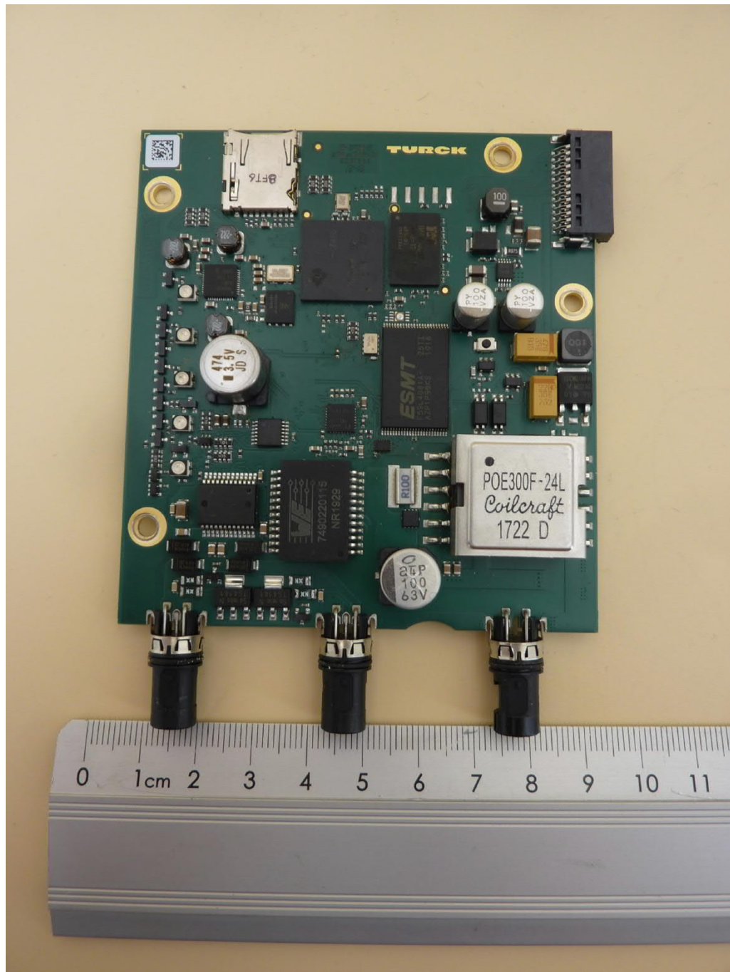
TN-UHF-Q180L300-NA-CDS, digital PCB, top view
