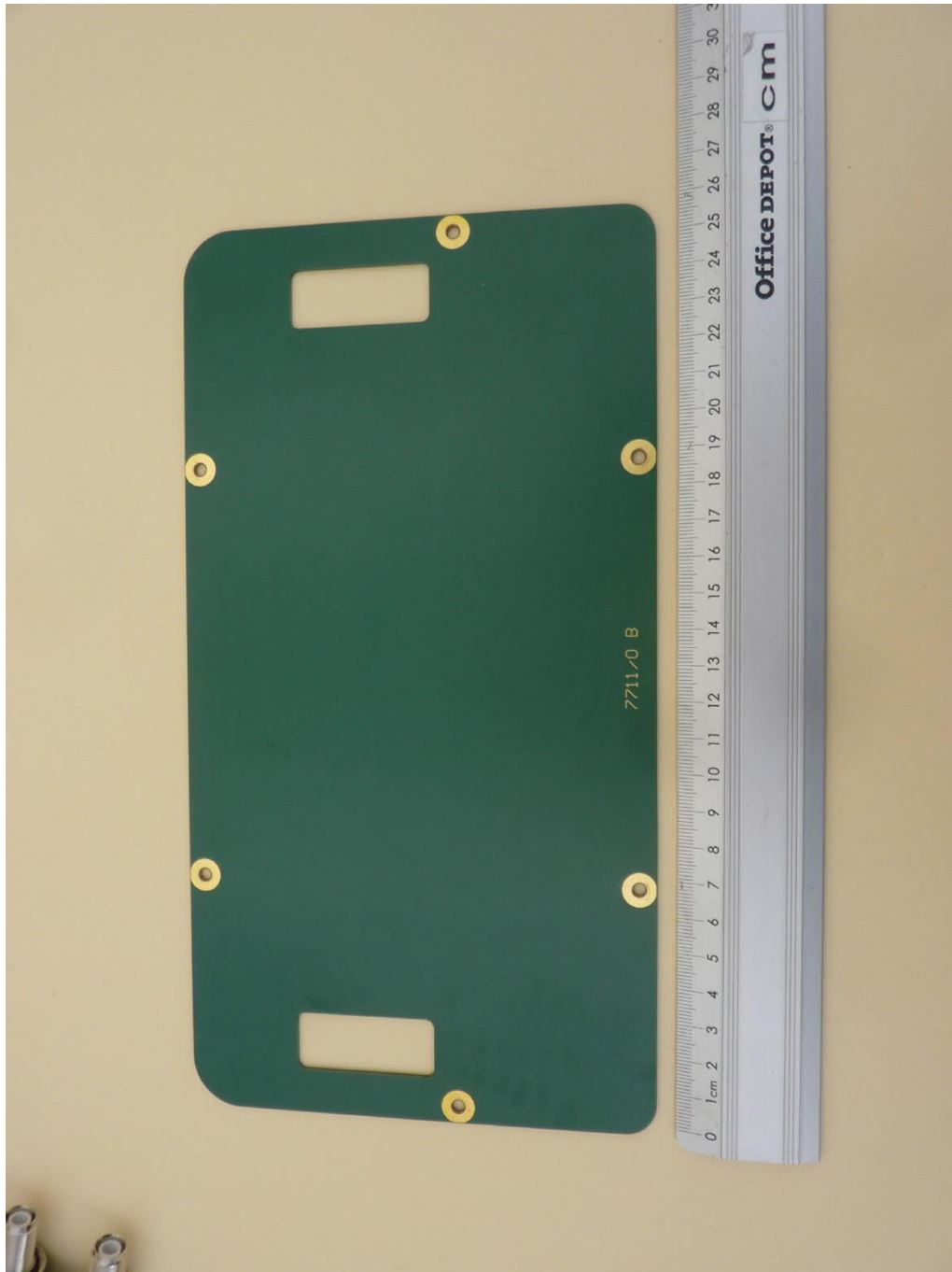
TN-UHF-Q180L300-NA-CDS, shield, top view
