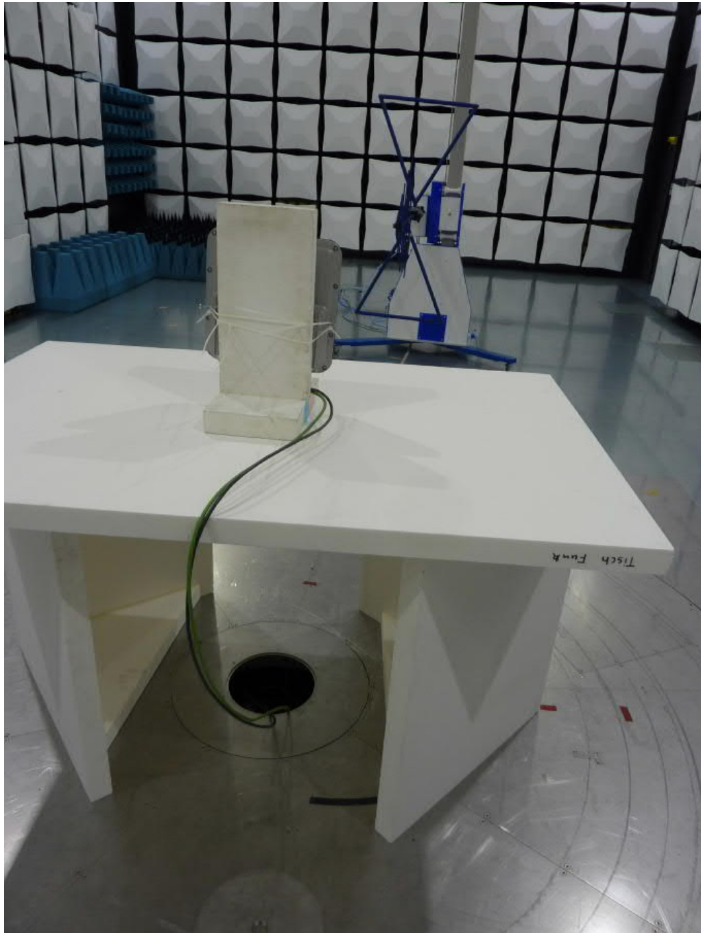
Test setup semi anechoic chamber, measurement from 30 MHz to 1 GHz
