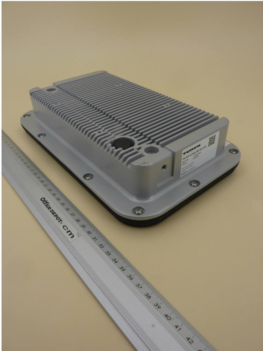
TN-UHF-Q180L300-NA-CDS, 3-D-view 2
