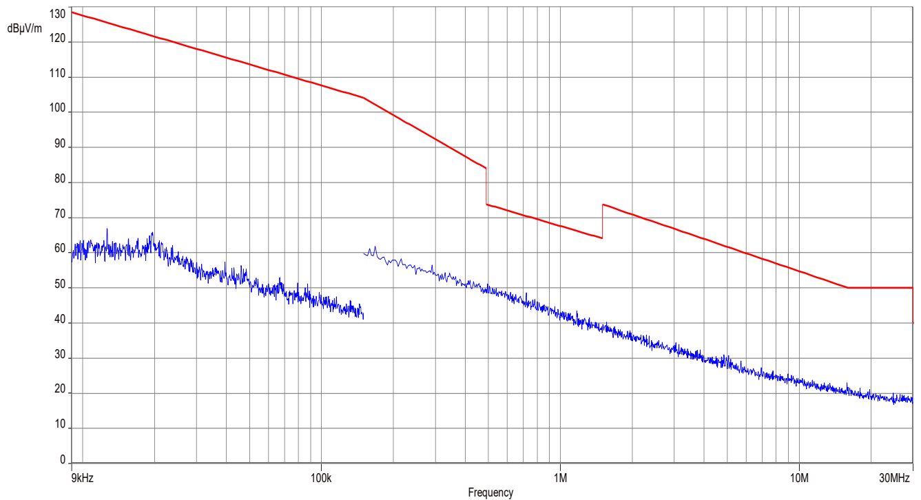
Plot 9: 9 kHz – 30 MHz, stop mode, high frequency
