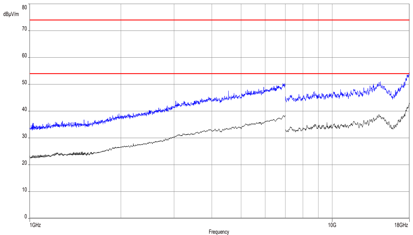
Plot 17: 1GHz – 18 GHz, stop mode, high frequency
