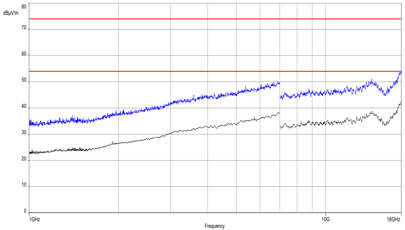
Plot 16: 1GHz – 18 GHz, stop mode, middle frequency
