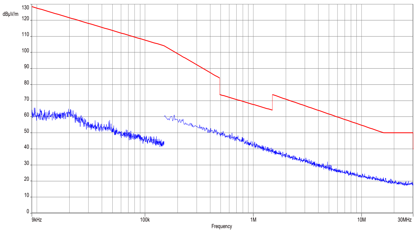
Plot 7: 9 kHz – 30 MHz, stop mode, low frequency
