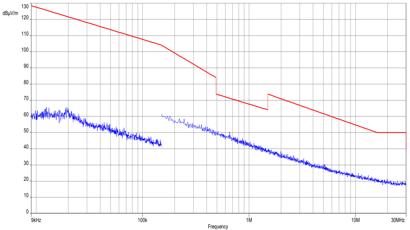
Plot 6: 9 kHz – 30 MHz, normal operation mode
