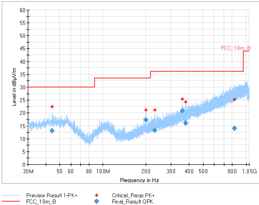
Plot 11: 30 MHz – 1GHz, stop mode, low frequency
