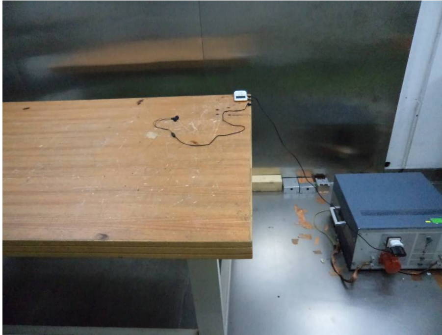
Conducted Emissions - Front View (charging & Multimedia playing mode)
