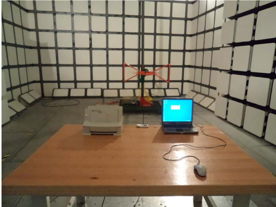
Radiated Emissions - Front View (downloading mode)
