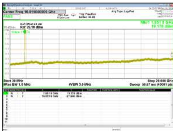
B2_HSDPA_Lower_Conducted Spurious
