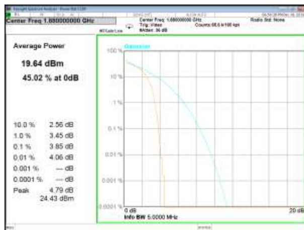
HSPA2_Middle_
