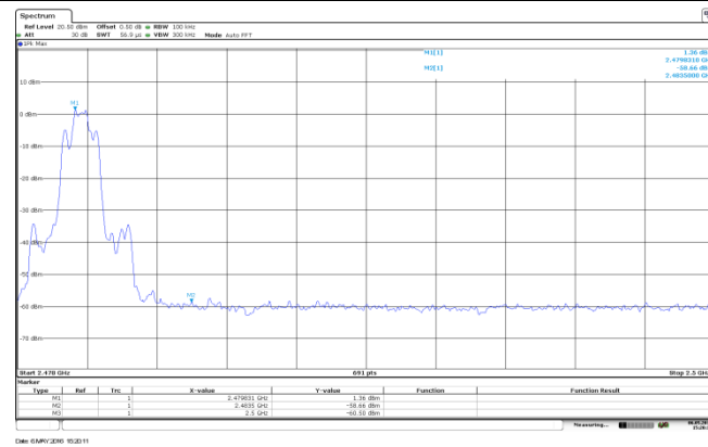
Bandedge- no hopping mode (CH78)
