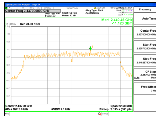
Channel 6 / 2437 MHz
