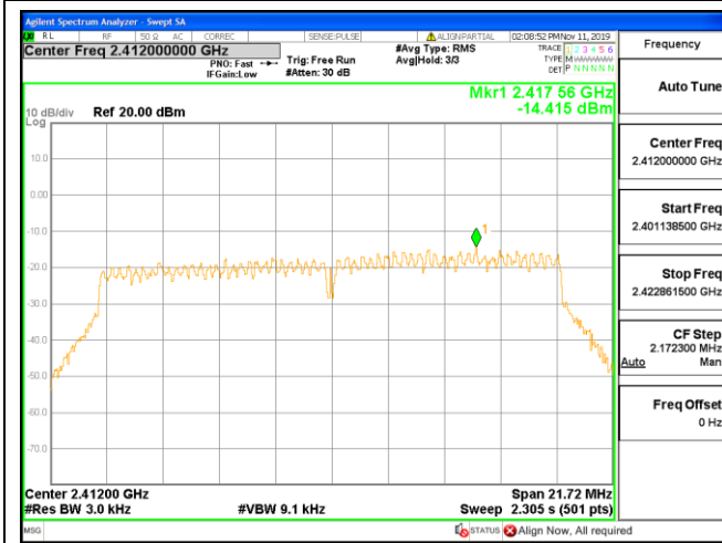
Channel 1 / 2412 MHz
