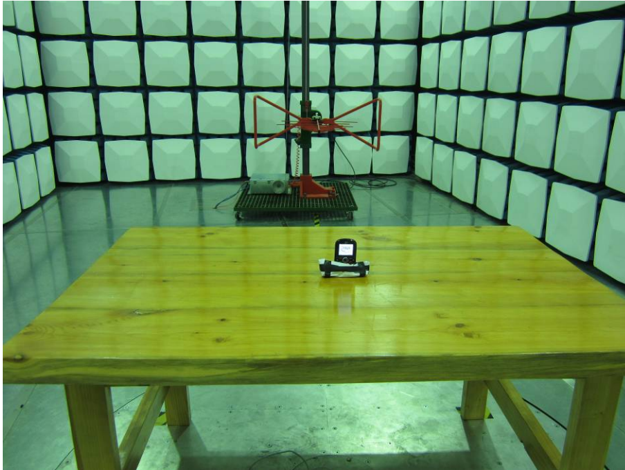
Below 1GHz: Radiated Emissions
