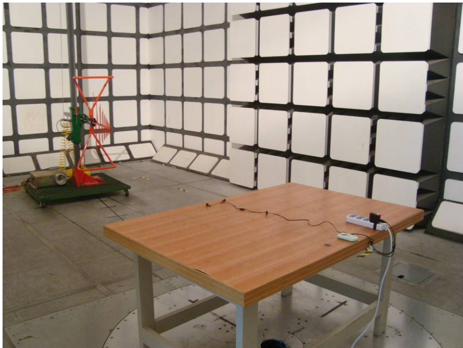
Radiated Emissions - Rear View (Multimedia Playing mode)
