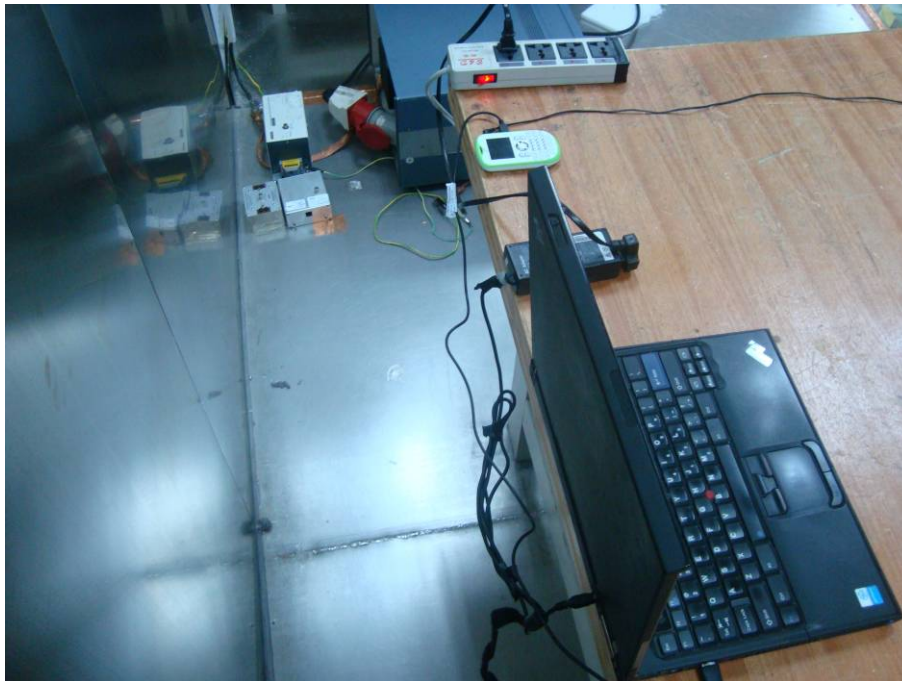
Conduction Emissions - Side View (USB Charging Mode)
